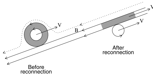
Figure 13 Mass depletion in the eruptive filament moving along the magnetic field. Left: two circular poloidal field lines indicate the cross section of the flux rope representing the erupting filament. Cool plasma between them (gray shading) moves together with the rope with a velocity V . Right: after magnetic reconnection. The center of the rope is displaced across the outer field B , and cool plasma continues to move along B .
