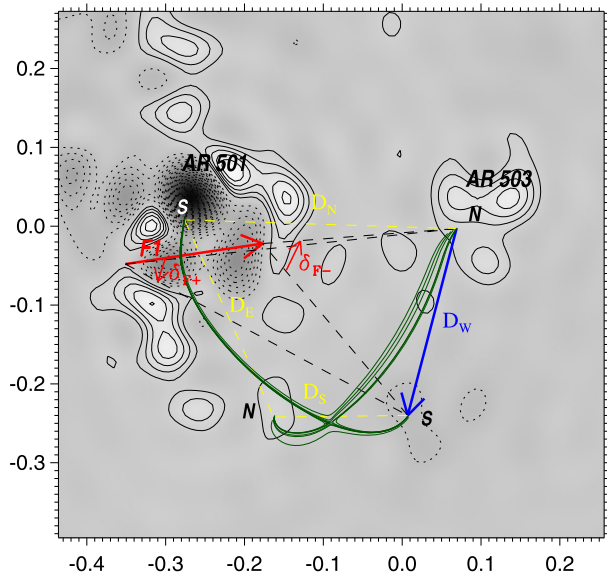
Figure 10 Top view of the magnetic configuration presented in Figure 8. The red vector \mathbf{F1} connects the photospheric bases of the erupted portion of the filament in AR 501. The yellow dashed lines D_N , D_S , D_E , and the blue vector \mathbf{D}_W connect the photospheric bases of the North, South, East, and West magnetic dipoles. \delta_{F1+} and \delta_{F1-} are the angular spans of vector \mathbf{D}_W measured from the ends of vector \mathbf{F1} . The axes are in solar radii from the solar disk center. The contour levels are symmetric relative to zero in steps of 35 G; dotted -(35, 70, \dots, 805) G, continuous +(35, 70, \dots, 175) G.
