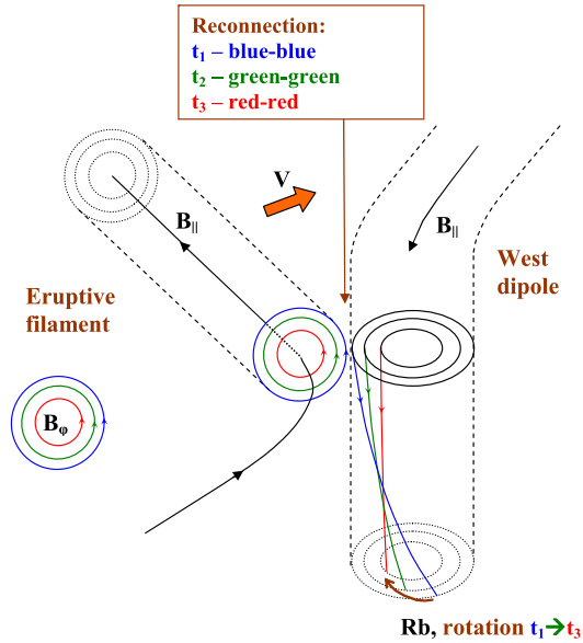
Figure 9 Interaction of the eruptive flux rope (left) and a nonuniformly twisted bundle (right) of magnetic field lines belonging to the West dipole and rooted in Rb. Their normal cross-sections are shown to be orthogonal in the place of interaction. The orange thick arrow indicates the direction of motion of the flux rope. The field lines sequentially involved in magnetic reconnection at times t_1 , t_2 , and t_3 are denoted with the colors presented in the top rectangle. Magnetic reconnection leads to a concurrent brightening that runs clockwise in the chromosphere and low corona above the Rb region (the brown round arrow at the bottom). The axial magnetic fields, B_{\parallel} , of the eruptive flux rope and the bundle correspond to the positions of the thick blue and red loops at t_1 in Figure 14(a), respectively.
