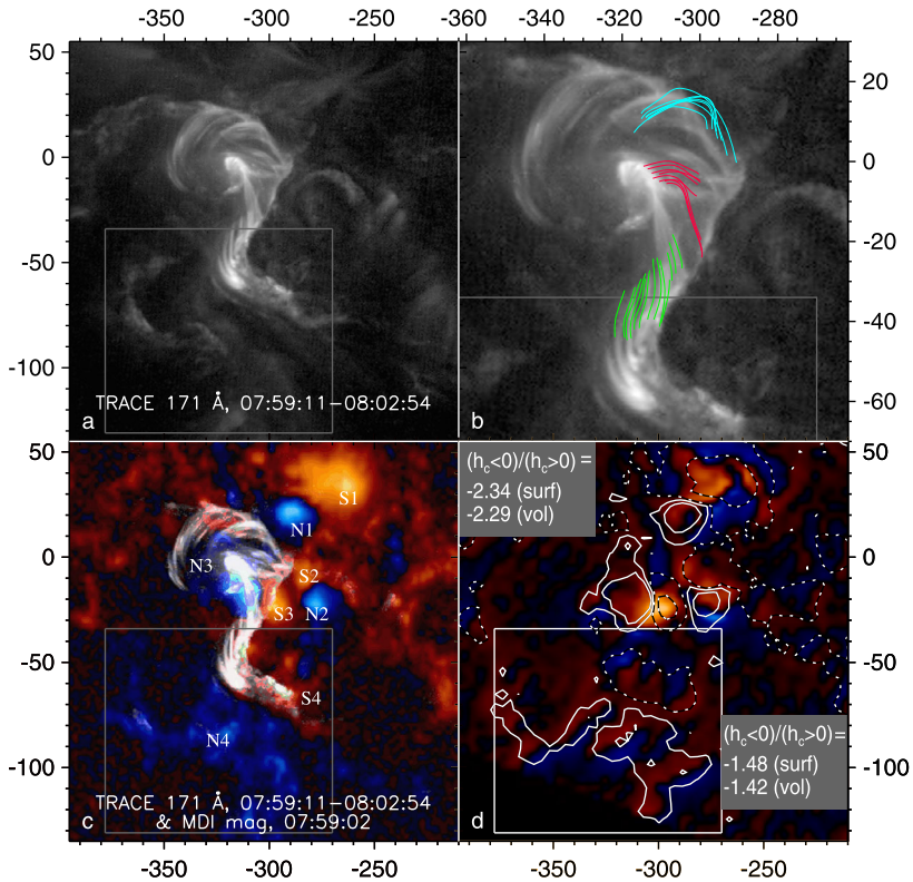
Figure 7 The magnetic helicity sign issue. (a) Inverse S-shaped arcade in a TRACE 171 Å composite image. The region analyzed by Chandra et al. (2010) is framed in all panels. (b) Enlarged image of the arcade overlaid with magnetic field lines calculated from the NLFF extrapolation. (c) Combination of the TRACE image in panel (a) with an MDI magnetogram (N-polarity blue, S-polarity red, numbering according to Chandra et al. , 2010). (d) Current helicity map computed from the NLFF extrapolation. Each pixel of this map is the photospheric base of a vertical column as high as 135 Mm. The red- (blue-) shaded regions correspond to the values of negative (positive) current helicity within the volume of this column. The contours outline the negative (dotted, -(120, 600) G) and positive (continuous, +(30, 250) G) B_z polarities in the BBSO magnetogram used in the computations. The top-left gray box presents the ratio of the total negative to positive current helicity at the photospheric layer (surf) and in the coronal volume (vol) for the whole region. The bottom-right gray box is related to the framed region. The axes are in arcseconds from the solar disk center.
