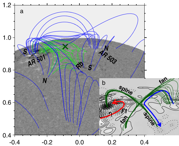
Figure 8 Side view of the coronal magnetic configuration around the pre-eruptive filament computed from the SOHO/MDI magnetogram of 18 November, 09:35 UT. (a) Field lines in the large-scale environment of the magnetic null point denoted with the dark-green slanted cross. (b) A selected set of field lines passing close to the magnetic null point shown in the same scale as in panel (a). The null point at their apparent intersection corresponds to the dark-green slanted cross in panel (a). The thick red arrow represents the pre-eruptive filament and the direction of its axial field. The small black circular arrow around it indicates its negative handedness. The blue arrow represents the connectivity of the west N–S dipole, which is a part of the S–N–S–N quadrupole. The relative position of the red and blue arrows suggests a positive handedness. The contour levels of the radial magnetic component are symmetric relative to zero in steps of 31 G: dotted -(15, 46, \dots, 728) G, continuous +(15, 46, \dots, 139) G. The axes are in solar radii from the solar disk center.
