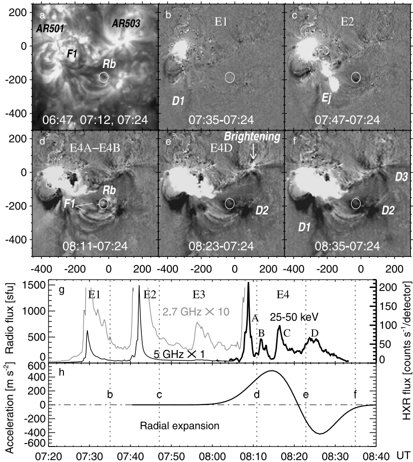
Figure 2 History of the event. (a) Pre-event situation in an averaged EIT 195 Å image, which is built with images taken at the hours indicated at the bottom of the panel. (b–f) Milestones in the event in the EIT 195 Å fixed-base difference images (the differences are taken between the hours indicated at the bottom of each panel). The solar rotation was compensated to 08:20 UT. The axes are in arcseconds from the solar disk center. (g) Time profiles in microwaves at 5 GHz (thin black line), 2.7 GHz (gray line, magnified by a factor of 10), and in HXR (thick black line). (h) The acceleration of the radial expansion of the invisible CME, which presumably erupted near the solar disk center close to region Rb. The labels E1–E4D in panels (b–f) denote the eruptive episodes marked in the time profiles in panel (g). The vertical dotted lines in panels (g) and (h) mark the observation times of panels (b–f).
