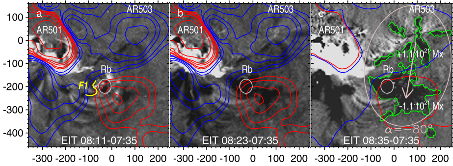
Figure 11 Manifestations of a presumable eruption at the solar disk center around 08:14 UT shown by the development of dimmings in EIT 195 Å images overlaid with the contours of the coronal B_r magnetogram extrapolated from an MDI magnetogram at a height of 28 Mm (blue N-polarity, red S-polarity). The contour levels are \pm(2.5, 5, 10, 15, 30, 60) G in panels (a) and (b) and \pm 2.5 G in panel (c). The yellow contour in panel (a) outlines the leading edge of the eruptive filament pouncing on a coronal obstacle above the bifurcation region Rb denoted by the small oval. The green contours in panel (c) outline the darkest dimming areas, which overlay a dipole outlined with a large oval. The arrow shows the direction of the resulting magnetic field in the dipole.
