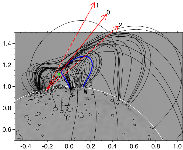
Figure 12 Side view of the magnetic configuration including arrows that indicate the trajectory of the upper part of the magnetic flux rope replacing the erupting filament F1. The trajectory of the rope (0) crosses a magnetic null point (green slanted cross). The cross section of the expanding field line is limited with the red dashed arrows 1 and 2. The thick solid curves correspond to the magnetic field lines. The blue magnetic field line denotes the magnetic flux from the West dipole (same as in Figure 8(b)). The thin contours on the solar surface correspond to the magnetic field values in steps of 34 G; they are -25 G (dotted) and +9 G (continuous) away from the stronger-field regions near the limb. The thick white circle denotes the solar limb. The axes are in solar radii from the solar disk center.
