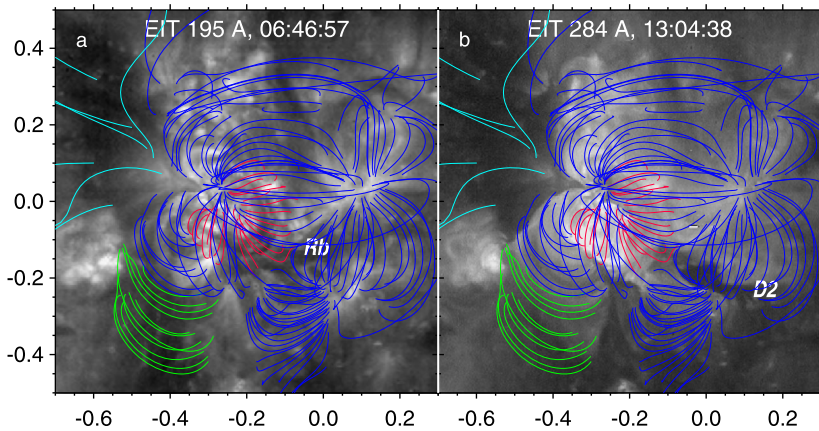
Figure 5 Extrapolated field lines overlaid on (a) a pre-event EIT 195 Å image and (b) a post-event EIT 284 Å image. All data were taken on 18 November. The MDI magnetogram at 09:35 UT was used for the potential extrapolation. The EIT images are corrected for the solar rotation to this time. The axes are in solar radii from the solar disk center.
