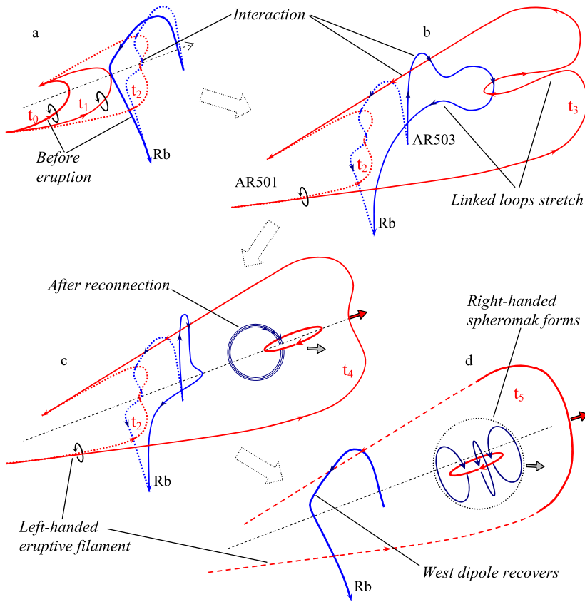
Figure 14 A hypothetical development of the situation presented in Figures 8(b) and 10 for the case when the trajectory (black dashed line) of the eruptive filament (active red loop) passes below the magnetic null point (arrow 2 in Figure 12). The blue loop is anchored at the West dipole involved in the eruption. Rb is the bifurcation region shown in Figures 1, 8, and 11. (a) t_0 : denotes the time before the eruption; the interaction of the loops starts at t_1 . The dotted lines at t_2 show the loops just after the onset of their interaction. The expanding red loop embraces the leg of the blue loop rooted in Rb and takes the Y-like shape (cf. Figure 1). (b) The stretching of the red and blue magnetic structures results in the formation of secondary loops, which are linked. (c) Magnetic reconnection detaches the secondary loops from the parent ones. A closed system of red and blue magnetic rings is formed. (d) The blue rings separate from each other and get distributed along the red ring, thus destroying remnants of its left helicity. A right-handed spheromak develops. The apparent intersections of the blue and red loops in panels (a)–(d) are due to the projection effect and do not imply the possibility of reconnection. Figure 4 roughly outlines the dynamic reconfiguration presented in panels (a) and (b) of this figure, but viewed from a different angle.
