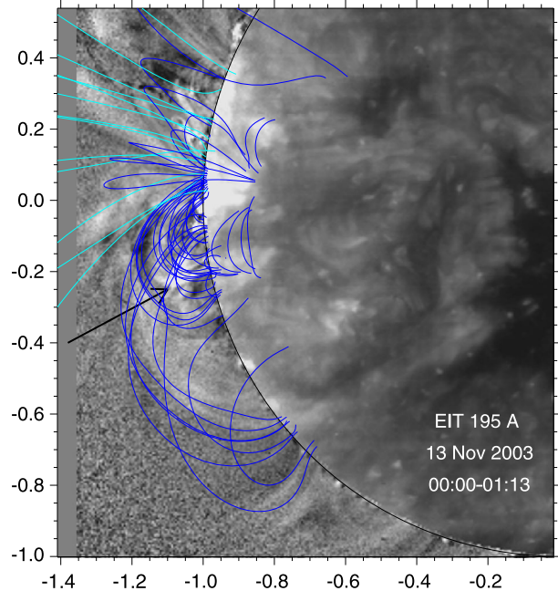
Figure 6 Comparison of the field lines computed in the potential approximation for the MDI magnetogram produced at 09:35 UT on 18 November with a synthetic EUV image composed from EIT 195 Å images actually observed on 13 November. The black arrow indicates the position of the topological discontinuity as it was on 18 November. The axes are in solar radii from the solar disk center.
