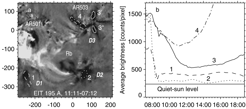
Figure 3 Dimming regions near the solar disk center well after the event. (a) The configuration of dimmings in the EIT 195 Å difference image. Five significantly dark and long-lived dimmed regions are selected using contours of different line styles. The solar rotation is compensated to 08:20 UT. The axes are in arcseconds from the solar disk center. (b) Time profiles in separate dimmed regions. Labels 1–4 denote the corresponding regions in panel (a); the styles of the lines in panel (b) and the corresponding contours in panel (a) are the same. The time profile 3 is averaged over regions 3' and 3''. The horizontal line presents the average quiet-Sun intensity level in the EIT 195 Å images, two of which were used for the difference in panel (a).
