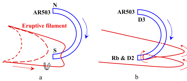
Figure 4 Presumable interaction between the eruptive filament (red) and a static coronal structure (blue) suggested by the observational hints. The static structure connects the N-polarity of AR 503 with an S-polarity plage region and region of bifurcation Rb. The arrows indicate the directions of the axial magnetic fields. The curled arrow indicates the direction of the poloidal flux in the filament. (a) The onset of the interaction. (b) Subsequent expansion of the eruptive filament. The interaction results in the development of dimmings D3, D2, and at the former position of Rb.
