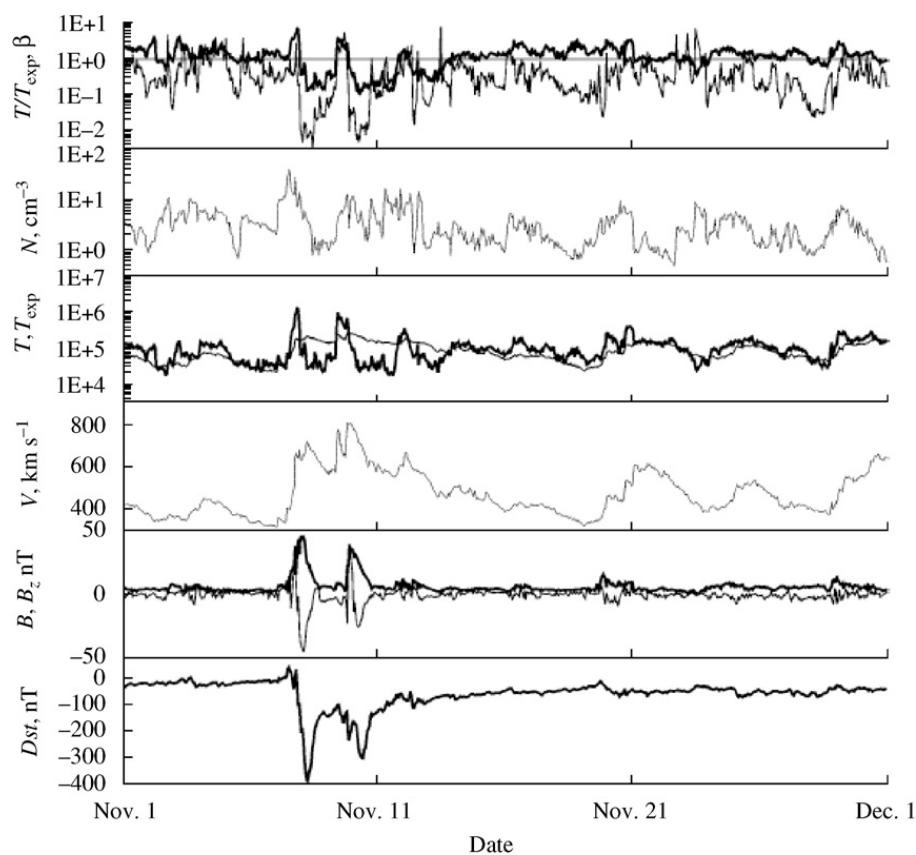
Fig. 6. Interplanetary space parameters in November 2004. Panels: 1— \beta -parameter (the ratio of the thermal and magnetic pressures, thin line) and the ratio of the proton temperature to such a temperature calculated from the average dependence of temperature on velocity, T/T_{\text{exp}} (thick line), 2—density, N , 3—proton temperatures T (thick line) and T_{\text{exp}} (thin line), 4—solar wind velocity, V , 5—IMF magnitude B (thick line) and B_z component (thin line), 6—Dst index.
