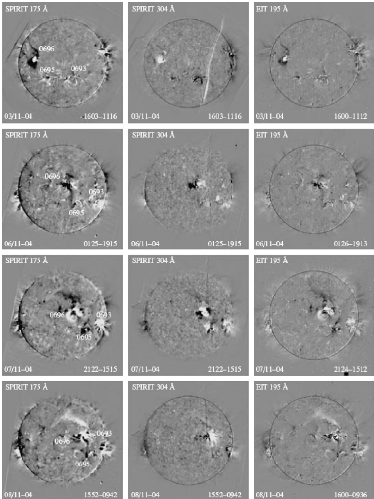
Fig. 3. Fixed-base difference images in the 175 and 304 Å channels of the SPIRIT telescope and similar images in the 195 Å channel of the SOHO/EIT telescope obtained on November 3, 6, 7, and 8, 2004.
