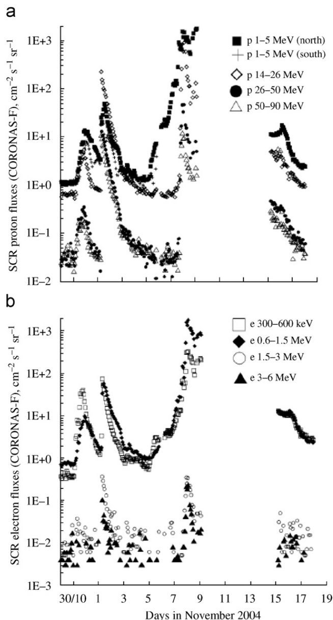
Fig. 7. Fluxes of (a) protons in both polar caps and (b) electrons in the northern polar cap from October 29 to November 18, 2004, according to the CORONAS-F satellite data.
