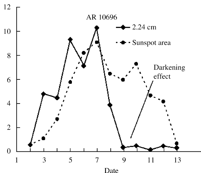
Fig. 5. Darkening effect in AR 10696 before the M2.5 flare of November 10, 2004. Dots show a change in the Sunspot area in the group at the level of the photosphere. Solid line corresponds to the total emission flux from AR 10696 at a wavelength of 2.24 cm.
