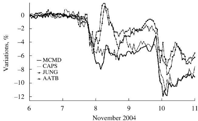
Fig. 9. Variations in the neutron monitor count rate relative to the base on November 6 at the stations: McMurdo (MCMD), R_c = 0.01 GV; Cape Schmidt (CAPS), R_c = 0.52 ; Jungfrauioh (JUNG), R_c = 4.48 ; Alma Ata 3300 m (AATB), R_c = 6.69 GV in November 2004.
