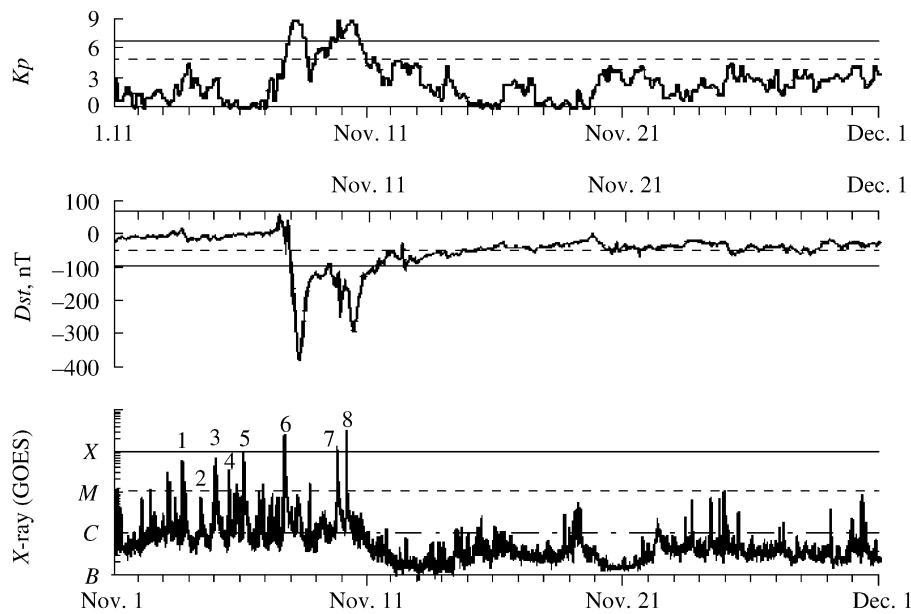
Fig. 1. The series of solar and ground-based measurements in November 2004. Nos. 1–8 correspond to the flares presented in Table 1.
