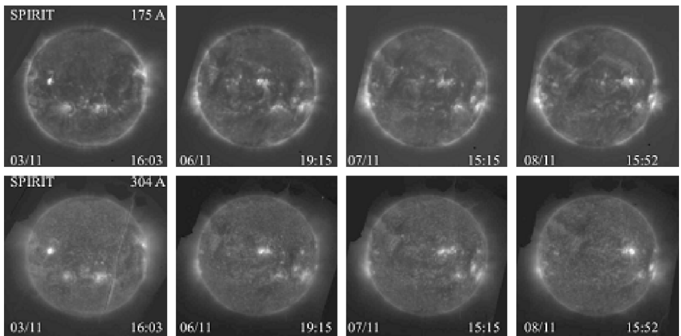
Fig. 2. SPIRIT/CORONAS-F images of the Sun in the 175 and 304 Å channels obtained on November 3–7, 2004.
