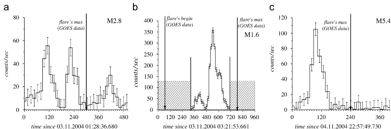
Fig. 4. Temporal profiles of solar flares observed by AVS-F instrument in November 3–4 2004 in energy band 0.1–1 MeV. Dashed areas correspond to satellite passing through Earth radiation belt.
