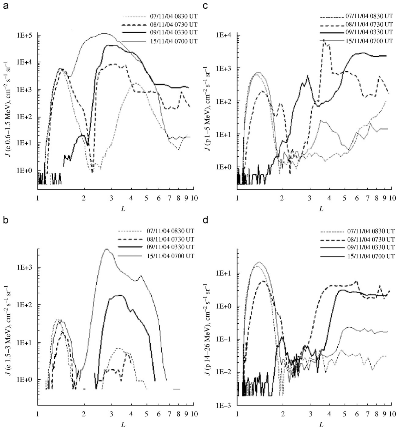
Fig. 8. Comparison of the profiles of the radiation belt particle fluxes: electrons with energies of (a) 600 keV–1.5 MeV and (b) 1.5–3 MeV and protons with energies of (c) 1–5 MeV and (d) 14–26 MeV.
