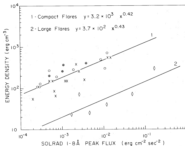
FIG. 13.—Plot of the energy density 3nkT ( \text{erg cm}^{-3} ) of X-ray limb flares versus the peak flux ( \text{erg cm}^{-2} \text{sec}^{-1} ) given by the Solrad 9 satellite in the spectral band 1–8 Å. Symbols have the same meaning as in Fig. 9. The two straight lines are least-squares fits for events of group C and of group A plus B, respectively.
