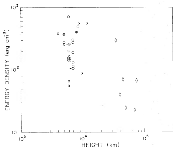
FIG. 12.—Plot of the energy density 3nkT ( \text{erg cm}^{-3} ) of X-ray limb flares versus the height (km). Symbols have the same meaning as in Fig. 9.
