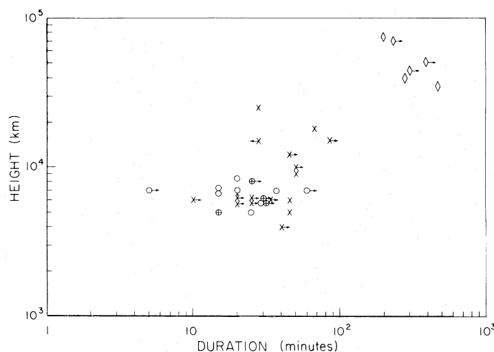
FIG. 9.—Plot of the height (km) of X-ray limb flares versus the total duration (minutes). Different symbols are used for the three morphological groups discussed in the text. Crosses, flares with compact loops (group A); circles, pointlike flares (group B); diamonds, flares with large and diffuse systems of loops (group C). Circles enclosing crosses are used for the cases in which the attribution of the event to group A or group B is uncertain.
