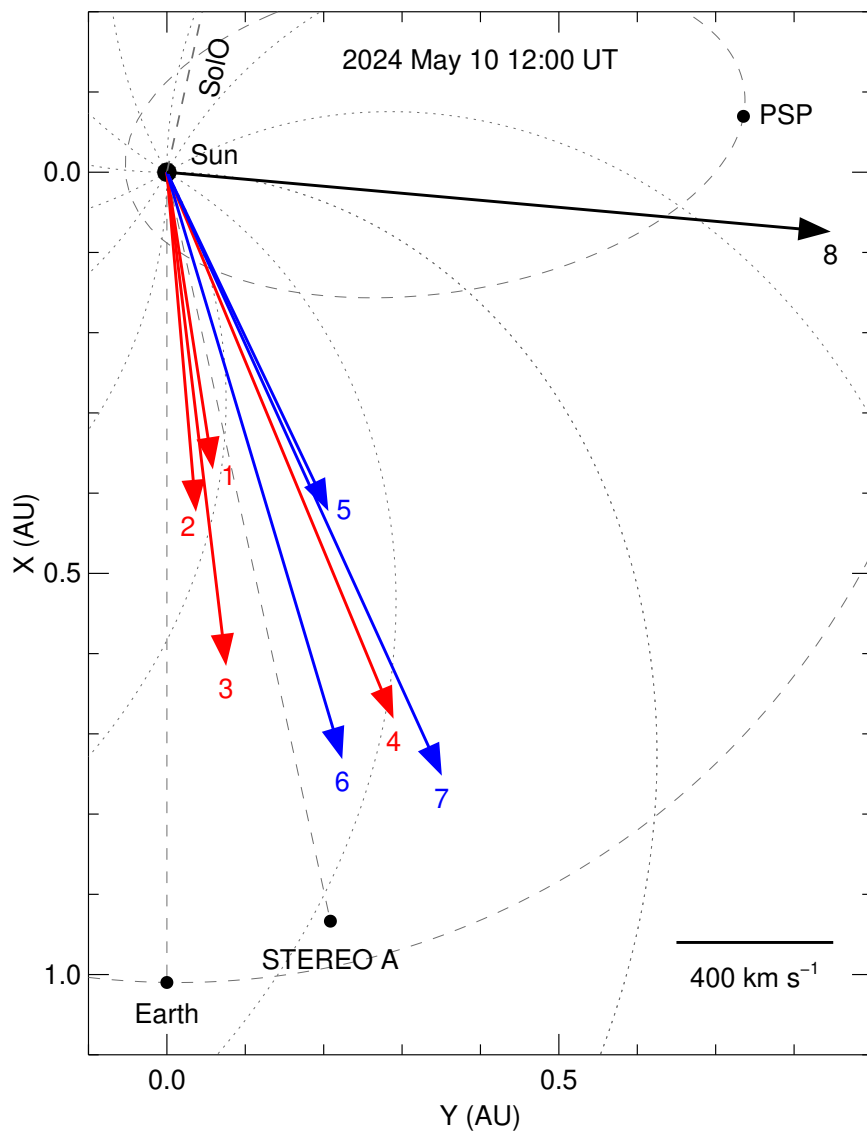
Fig. 1.— Positions of the spacecraft in the ecliptic plane at 12:00 UT on 2024 May 10. The dashed lines indicate the longitudes of the Earth (upstream of which Wind and SOHO are located), STEREO A and SolO, respectively. The gray dashed curves are the orbits of the Earth and PSP. The dotted lines show Parker spiral magnetic fields created with a solar wind speed of 450 \text{ km s}^{-1} . The arrows mark the propagation directions of the full halo CMEs from May 8 - 13 obtained through CME reconstruction, with the lengths of the arrows indicating CME velocities near the Sun. Red (blue) arrows represent CMEs that likely contributed to the first (second) complex ejecta at the Earth. The numbers label the CMEs as in Table 1.
