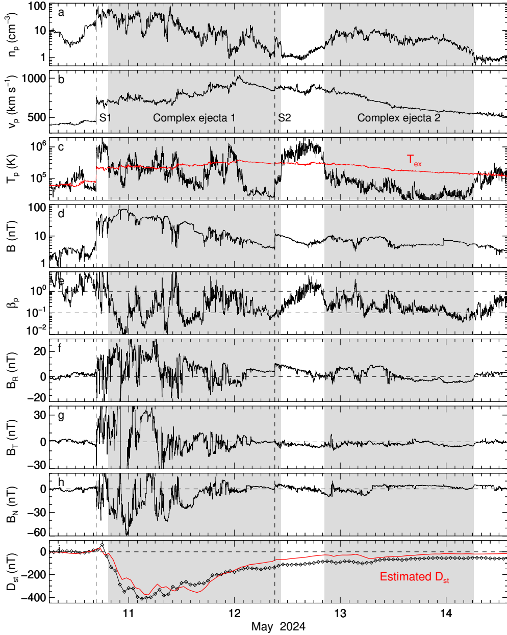
Fig. 3.— Solar wind parameters observed at Wind and measured D_{st} index. From top to bottom, the panels show the proton density (a), bulk speed (b), proton temperature (c), magnetic field strength (d), proton \beta (e), magnetic field components (f-h), and D_{st} index (i), respectively. The shaded regions indicate the intervals of two complex ejecta, and the vertical dashed lines mark the associated shocks. The red curve in panel (c) denotes the expected proton temperature calculated from the observed speed (Lopez 1987; Richardson & Cane 1995). The red curve in panel (i) represents the estimated D_{st} index by combining the formulas of Burton et al. (1975) and O’Brien & McPherron (2000).
