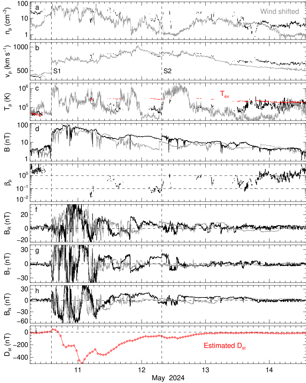
Fig. 4.— Solar wind parameters observed at STEREO A and estimated D_{st} index. Data at Wind, which are shifted forward in time by about 2.6 hr, are shown in gray for comparison. Similar to Figure 3.
