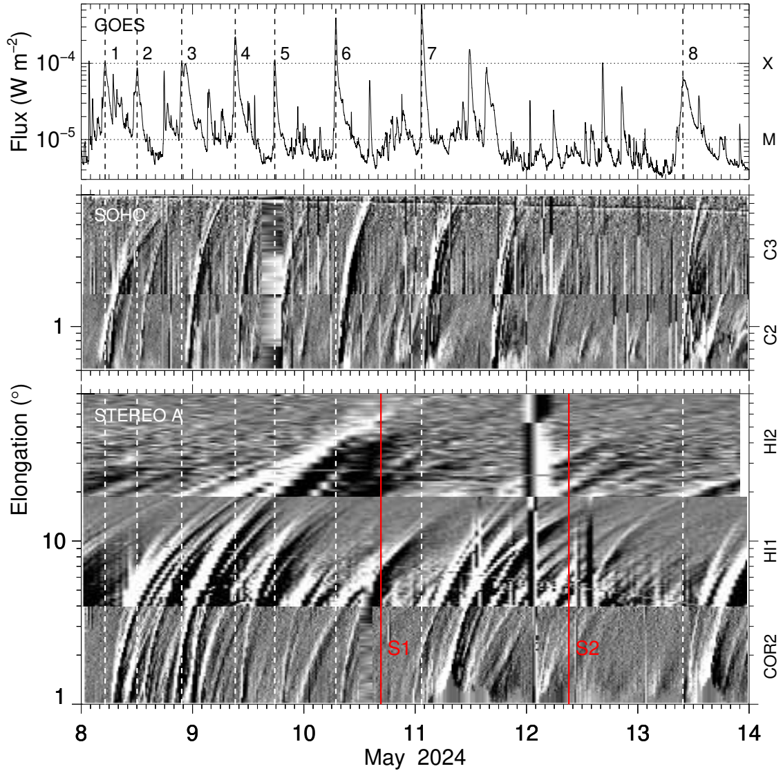
Fig. 2.— Full halo eruptions on May 8 - 13. Top: GOES X-ray flux at 1 - 8 Å. Middle: Time-elongation maps from LASCO of SOHO (at a position angle of 90^\circ measured clockwise from the solar north). Bottom: Time-elongation maps from SECCHI of STEREO A (at a position angle of 270^\circ clockwise from the solar north). The vertical dashed lines indicate the peak times of the associated flares, with the numbers labelling the eruptions as in Table 1. The red vertical lines mark the observed arrival times of the shocks at the Earth.
