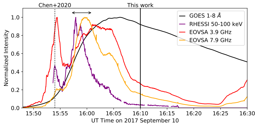
Figure 2. Microwave and X-ray light curves of the X8.2-class eruptive solar flare on 2017 September 10. The solid vertical line indicates the time of interest of this work during the gradual phase of the flare (around 16:10 UT). The vertical dotted line marks the time studied by Chen et al. (2020b) during the early impulsive phase of the flare when the eruption was initiated, and the double-sided arrow denotes the main impulsive phase of the flare around the primary hard X-ray and microwave peak (see Gary et al. 2018 for more details on the flare evolution).
