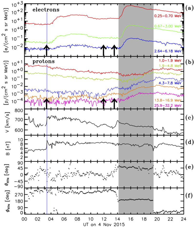
Figure 20 Energetic electron and proton, solar wind speed, and magnetic field vector observations during 4 November 2015, from instruments on SOHO and ACE at L 1 . Thick vertical black arrows mark the start times of Events 1–3.
