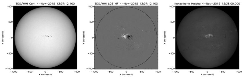
Figure 1 Overview of the Sun at 13:37 UT on 4 November 2015. ( Left ) SDO/HMI continuum image, ( middle ) SDO/HMI line-of-sight magnetogram, ( right ) H\alpha image from the Kanzelhöhe Observatory, all recorded during the rise phase of Event 3.
