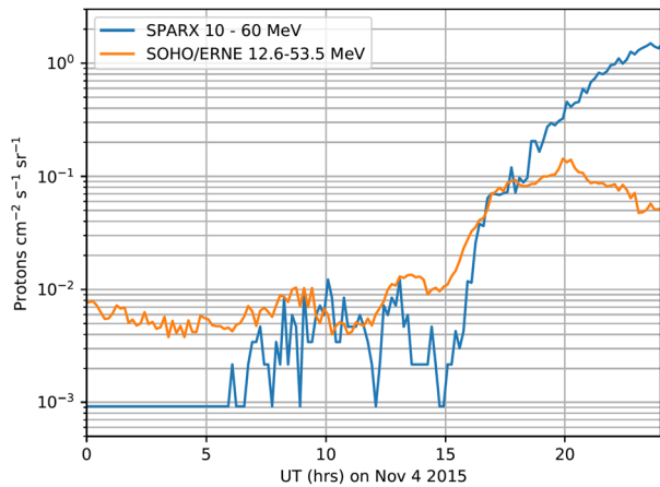
Figure 24 Combined integral ERNE HED proton observations on 4 November for 12.6–53.5 MeV (orange) are compared with the temporal profile predicted for 10–60 MeV protons by the SPARX forecasting software of Marsh et al. (2015) (blue), assuming a mean solar wind speed of 700 \text{ km s}^{-1} . At the time of this event, SOHO was rotated 180 degrees, so ERNE was pointing perpendicular to the mean magnetic field.
