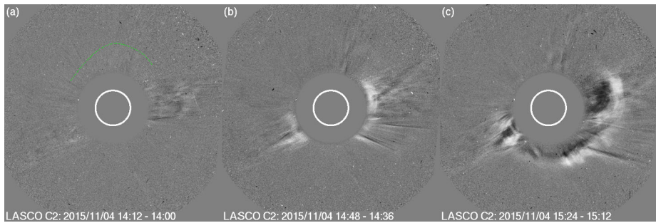
Figure 14 The evolution of the CME for Event 3. See text for detail.
