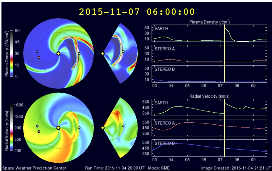
Figure 25 Snapshots of spatial maps in (left) the ecliptic plane and (middle) the meridional plane through the Sun–Earth line, as well as (right) temporal variations at Earth’s location for the (upper row) plasma density and (lower row) plasma speed. According to this run, the predicted shock-arrival time was 06:00 UT on 7 November 2015.
