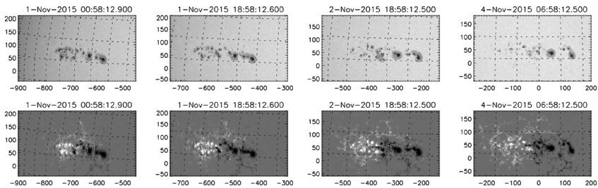
Figure 2 Evolution of NOAA AR 12443 from 1 to 4 November 2015. ( Top ) SDO/HMI continuum images and ( bottom ) SDO/HMI line-of-sight magnetograms (with the grayscale saturated at \pm 1000 G). Units are arcseconds from Sun center.
