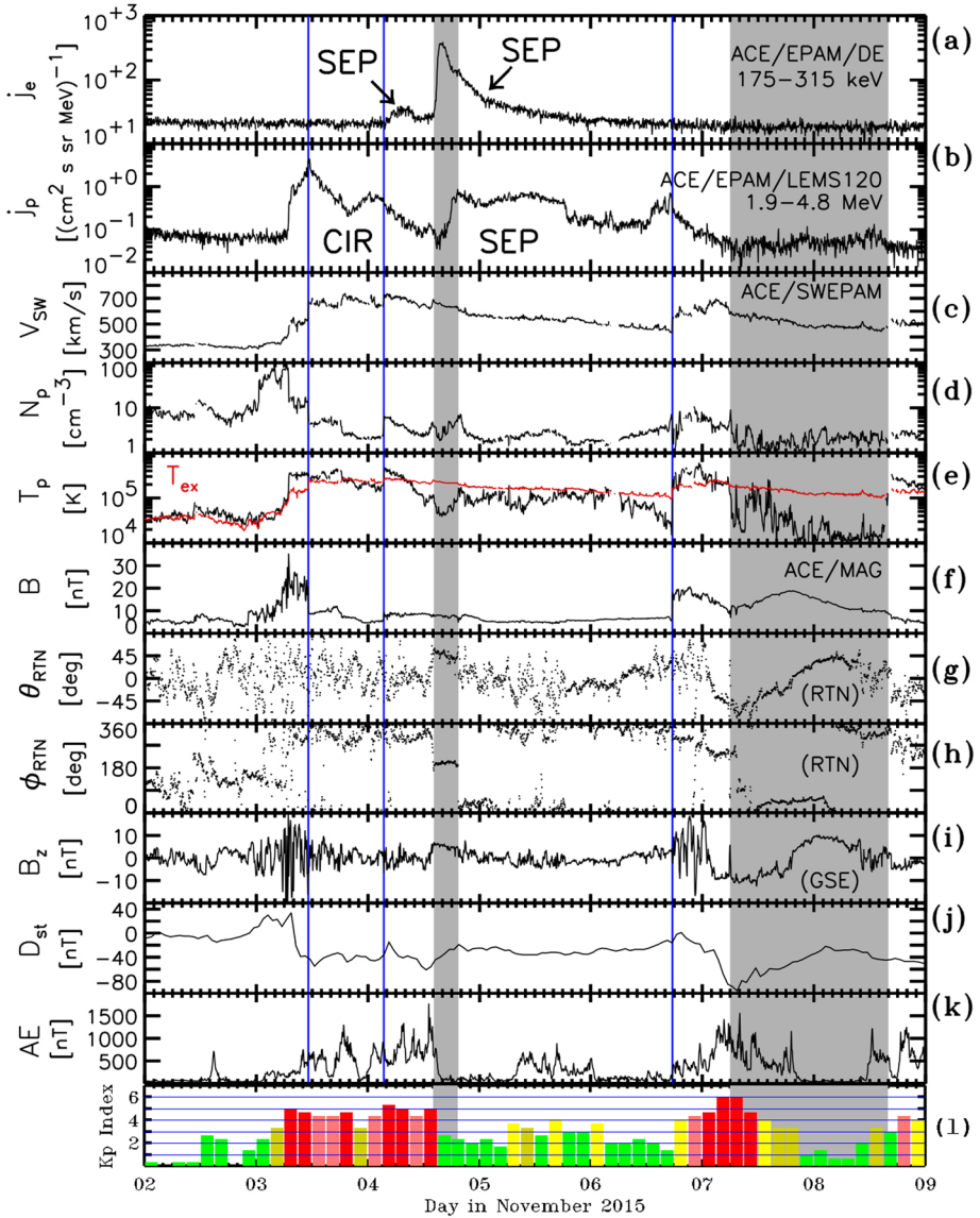
Figure 19 Overview of in-situ observations: (a) 175–315 keV electron intensities, (b) 1.9–4.8 MeV ion intensities, (c) solar wind proton speed, (d) solar wind proton density, (e) solar wind proton temperature, (f) magnetic field magnitude, (g) magnetic field latitudinal angle, (h) magnetic field azimuthal angle, (i) B_z , the z GSE component of the field, (j) Dst index, (k) AE index, and (l) Kp index. Blue-vertical lines identify shocks while shaded areas correspond to ICME periods. See text for details.
