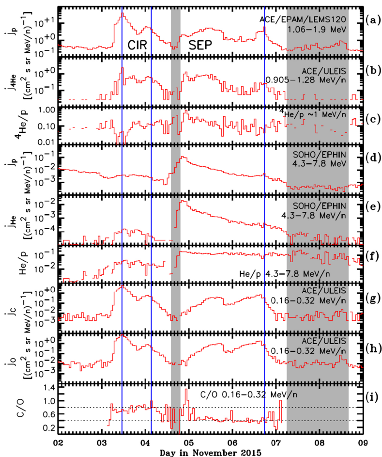
Figure 21 Intensities and abundance ratios of multiple energetic ions observed by ACE/EPAM, ACE/ULEIS, and SOHO/EPHIN between 2 November and 9 November 2015: (a) 1.06–1.9 MeV proton intensity, (b) 0.905–1.28 MeV n^{-1} helium intensity, (c) helium to proton abundance ratio at \approx 1 MeV n^{-1} , (d) 4.3–7.8 MeV proton intensity, (e) 4.3–7.8 MeV n^{-1} helium intensity, (f) 4.3–7.8 helium to proton ratio, (g) 0.16–0.32 MeV n^{-1} carbon intensity, (h) 0.16–0.32 MeV n^{-1} oxygen intensity, and (i) 0.16–0.32 MeV n^{-1} carbon-to-oxygen ratio. Increases associated with CIRs and SEPs are labeled, as are ICME periods ( shaded regions ) and shocks ( blue-vertical lines ).
