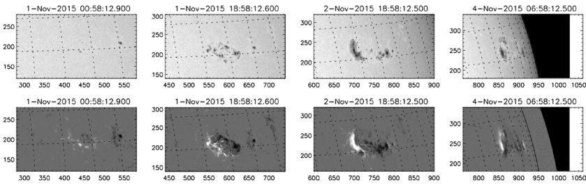
Figure 3 Evolution of NOAA AR 12445 from 1 to 4 November 2015. ( Top ) SDO/HMI continuum images and ( bottom ) SDO/HMI line-of-sight magnetograms (with the grayscale saturated at \pm 1000 G). Units are arcseconds from Sun center.
