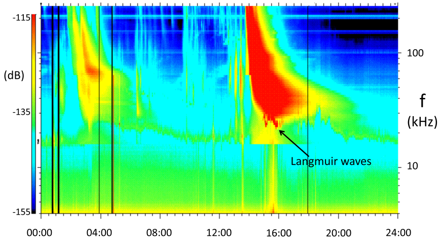
Figure 16 Wind /WAVES/TNR dynamic spectrum for 4 November 2015.
