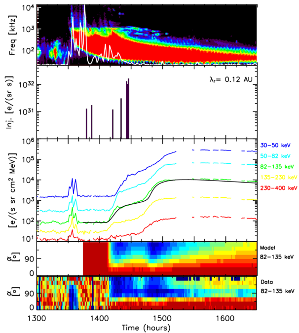
Figure 23 From top to bottom: Radio spectra observed by Wind / WAVES (color-coded by intensity, with red corresponding to large values and black the background) and 13 MHz microwave emission (white curve, the relative intensity) on 4 November 2015 (for comparison purposes with the particle data, the emissions were shifted by -500 seconds); 82–135 keV electron source profile deduced at 2 R_{\odot} ; omni-directional intensities observed by Wind / 3DP in the energy range 30–400 keV, with the black curve showing the best fit to the 82–135 keV data for \lambda_r = 0.12 AU; the two bottom panels show the modeled and observed 82–135 keV electron pitch-angle distributions normalized to the maximum value (1 = red to 0 = blue).
