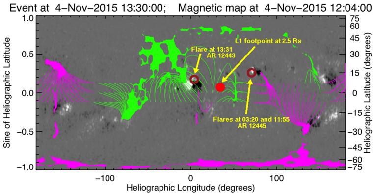
Figure 17 Predictions of a PFSS model with HMI photospheric magnetic field data for a synoptic magnetic map at the photosphere in Carrington coordinates around the time of the second flare, except that the Carrington longitudes are translated to Earth-view longitudes. The open circles show the photospheric locations of the flares with solar rotation corrected. The red circle is the footpoint of the magnetic field line traced from L_1 to the source surface at 2.5 R_{\odot} using Wind spacecraft velocity data and the Parker spiral (second method in the text). Open field regions are marked in two colors (green: positive, and pink: negative).
