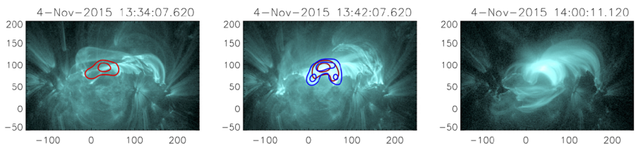
Figure 8 Snapshots showing the evolution of Event 3 in AIA 131 Å filtergrams. Red and blue lines are contours from RHESSI X-ray images reconstructed during the early rise phase (left) and peak (middle) in the 6–12 and 20–50 keV energy bands, respectively. The right-most image is after the event. Units are arcseconds from Sun center.
