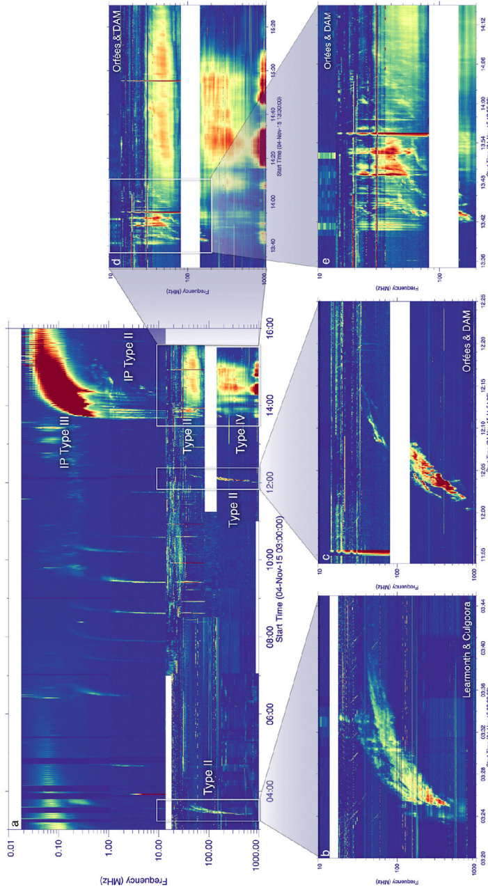
Figure 15 (a) Summary of all radio dynamic spectra for the events on 4 November 2015. Constructed from a mosaic of Wind /WAVES, Learmonth, Culgoora, Orfées, Nançay (NDA), and Callisto (Bleten, Mauritius, and Gauribidanur). (b) Event 1 was associated with a metric Type II radio burst that began at \approx 600 MHz that does not extend obviously below 10 MHz. Weak Type III radio bursts occur prior to the Type II burst and then start at the same frequency as the Type II near 03:30:15, 03:31:15, and 03:33:00 UT. These are associated with a small interplanetary Type III observed by Wind /WAVES in (a). (c) Event 2 was associated with strong metric Type II emission, beginning at \approx 800 MHz. No interplanetary Type IIs or IIIs were observed for this event. (d) – (e) Event 3 was associated with at least three metric Type II bursts (see the details in (e)); multiple metric Type III bursts, and a Type IV burst over the band 20–700 MHz. These metric events led to an interplanetary Type II and numerous interplanetary Type IIIs.
