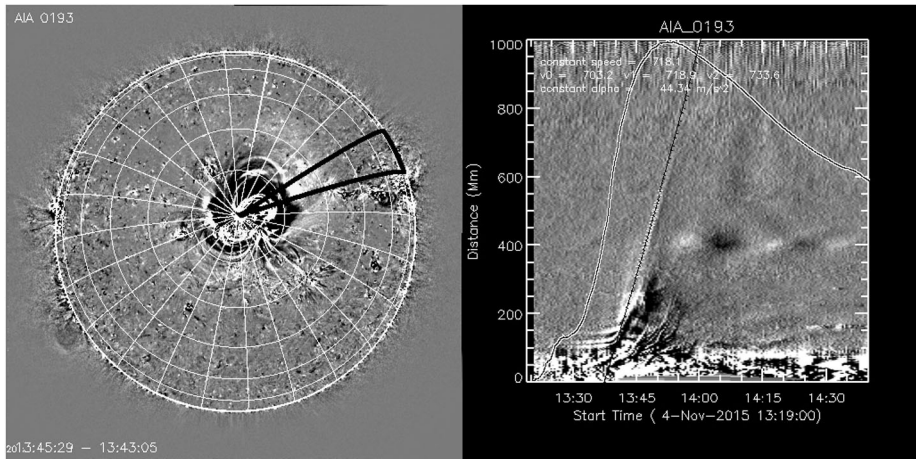
Figure 11 The kinematics of the EUV wave for Event 3. (Left): The speed and acceleration are calculated along great circles averaged in 24 15°-wide sectors that originate at the flare center. (Right): Space–time plot of the sector marked in black in the left panel. The normalized GOES 1–8 Å light curve is overplotted using a black line superposed on a broader white curve. Even in running-difference images the wave front is diffuse. The selected sector is one of the few that let us trace the front edge of the wave.
