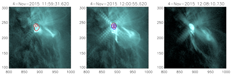
Figure 7 Snapshots showing the evolution of Event 2 in AIA 131 Å filtergrams. Red and blue lines are contours from RHESSI X-ray images reconstructed during the early rise phase (left) and peak (middle) in the 6–12 and 20–50 keV energy bands, respectively. The right-most image is after the event. Units are arcseconds from Sun center.
