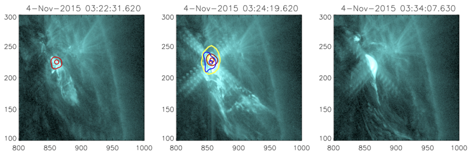
Figure 5 Snapshots showing the evolution of Event 1 in AIA 131 Å filtergrams. Red and blue lines are contours from RHESSI X-ray images reconstructed during the early rise phase ( left ) and peak ( middle ) in the 6–12 and 30–100 keV energy bands, respectively. The right-most image is after the event. Yellow contours are from a NoRH 17 GHz image at event peak. Units are arcseconds from Sun center.
