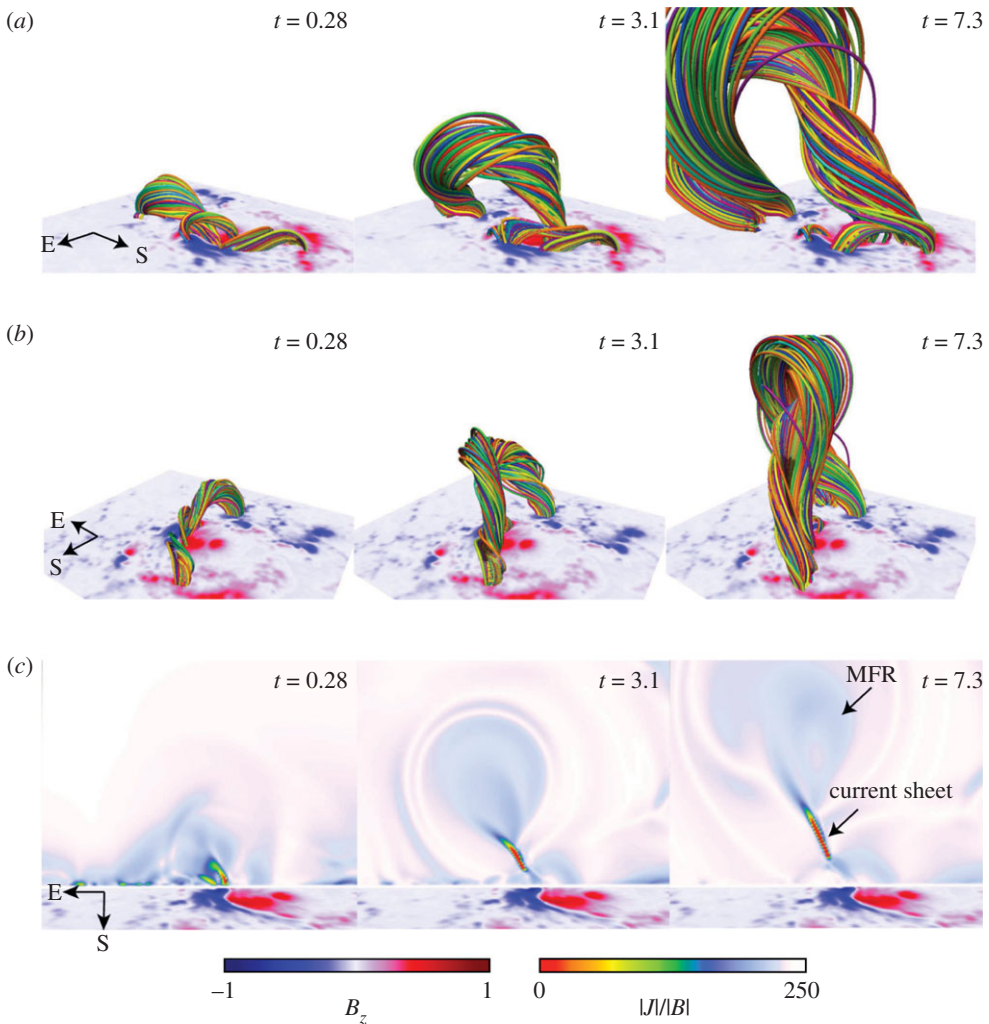
Figure 4. Temporal evolution of the formation and dynamics of an eruptive magnetic flux rope (MFR). ( a,b ) The field lines from different viewing angles. E and S stand for east and south. An animation of these panels is available in the original article, its duration is 4 s. ( c ) Temporal evolution of |J|/|B| plotted in the x - z plane at y = 0.38 , with a viewpoint from the south [58].
