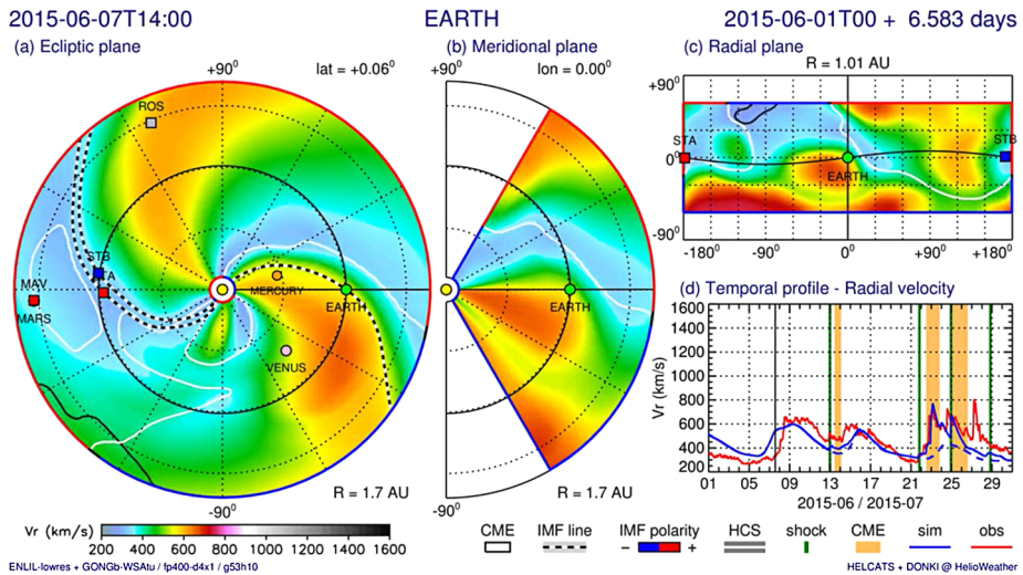
Figure 5 Solar wind radial velocity contour plots for 7 June 2015 14 UT shown in the ecliptic (a), meridional (b), and radial (c) planes. Panel d shows the time profiles of the measured and simulated (red and blue, respectively) radial solar wind velocity near Earth. Simulation results are taken from http://helioweather.net .
