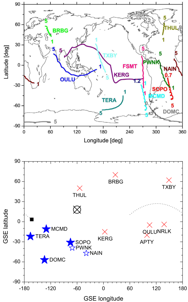
Figure 3 Asymptotic directions of the analyzed NMs for the peak of the event (6 June 2017 15:00 UT). The upper panel shows the directions (in geographical coordinates) for protons in the rigidity range from 0.7–5 GV. The bottom panel shows the directions (in GSE coordinates) for 1 GV rigidity protons. Stations with significant, marginal, and no increase are denoted as filled stars , open stars , and red crosses , respectively. Acronyms of station names are open in Table 1. The crossed circle corresponds to the direction of the IMF derived from the ACE satellite measurements during the event onset. The dotted curve represents the asymptotic cone for 1–1.5 GV protons (the small black square corresponds to 1 GV) of the southernmost point of the PAMELA orbit at 14:34 UT.
