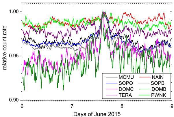
Figure 2 Normalized smoothed count rates of the NMs (cf. Figure 1). All curves were smoothed by the 45-minute running average and normalized to unity on 15:00 UT 7 June 2015.
