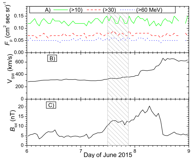
Figure 4 Near-Earth interplanetary conditions (hourly data) during the period of 6–8 June 2015 according to the OMNIWeb Database. Top panel: integral proton flux, F_p , with energies above 10, 30, and 60 MeV as denoted in the legend. Central panel: solar wind proton flow speed. Bottom panel: magnitude of the total IMF. The gray hatched area denotes the interval of the event as identified from NMs.
