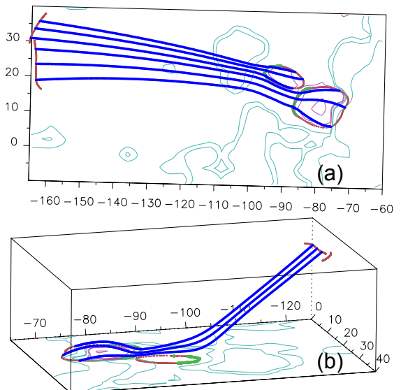
Fig. 11. Magnetic field model showing field lines that trace the BP separatrices. (a) Corresponds to the observer’s point of view. Field lines extending to the east are large-scale and open in our model (ie they reach the borders of our computational domain). (b) Shows the field lines from a different point of view (rotated by around 180^\circ and seen sideways) to clearly illustrate that the separatrix traces to the east are not at the photosphere but reach the top surface of the drawn box. The height of the box is 50 Mm in this figure. For clarity we are only including field lines tracing BP1 separatrix in this panel, a similar field-line tracing is found for BP2. The conventions for the field isocontours, axes, BPs, and separatrix traces are the same as in Fig. 10.
