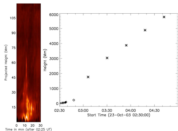
Fig. 7. Projected height vs. time plots showing the link between the jet and the narrow CME. The left panel shows the time-slice diagram built along the white dashed line shown on the H\alpha image at 02:37:48 UT (Fig. 6e). The right panel is a height-time plot combining the H\alpha measurements of the jet length projected on the POS (vertical crosses), a similar measurement done on the EIT image at 02:48 UT (diamond), and those of the associated CME using data from the CDAW SOHO/LASCO Catalog (asterisks).
