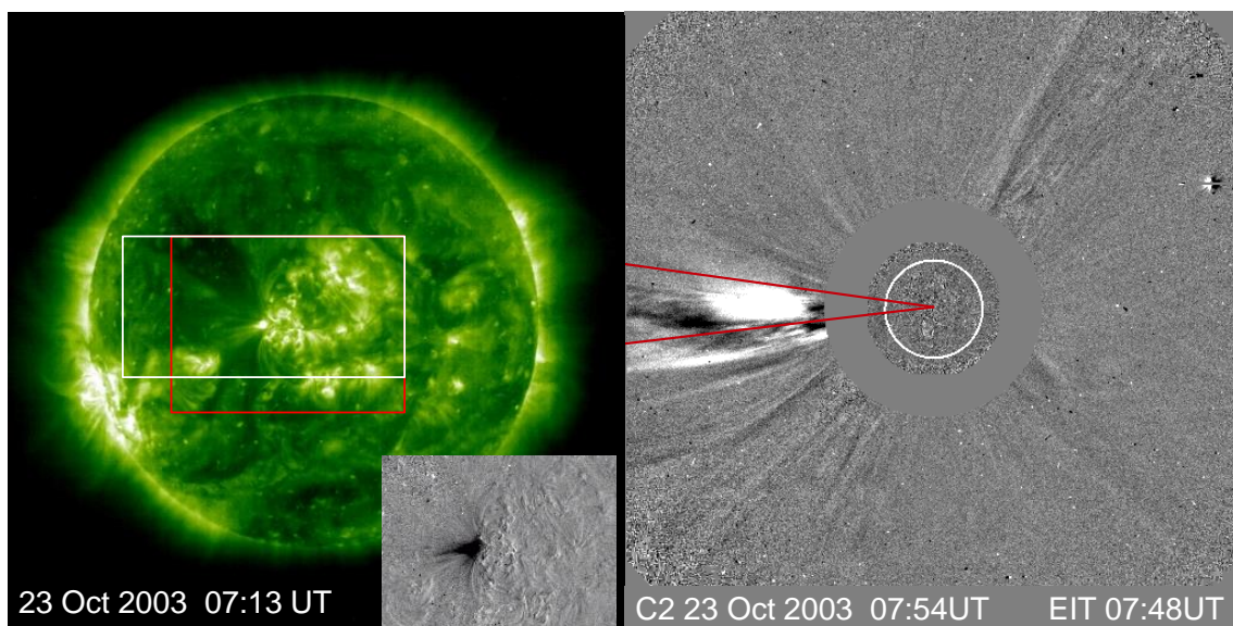
Fig. 1. EIT image and LASCO C2 difference image of a jet and associated narrow CME. (left panel) EIT full-disk image on 23 October 2003 at 07:13 UT showing a broad jet originating from the eastern border of AR 10484 at its maximum extension. The inset to its bottom right is the partial EIT difference image within the red rectangle in the full-disk image. (right panel) LASCO C2 difference image of the associated narrow CME. The two red continuous lines are drawn to indicate the CME angular width. Notice a very weak feature to the north of the CME bulk emission. This feature could appear due to projection effect because the CME propagation direction has an important component towards the observer, as deduced from the source region location. If we take it as the northern CME edge, then, the AW would be of \approx 23^\circ , while the true width of the ejection is smaller. The broad feature to the south corresponds to a previous CME. The coronal evolution in the region indicated by the white rectangle is available as a movie in the online edition. These white and red rectangles partially overlap to the north and west.
