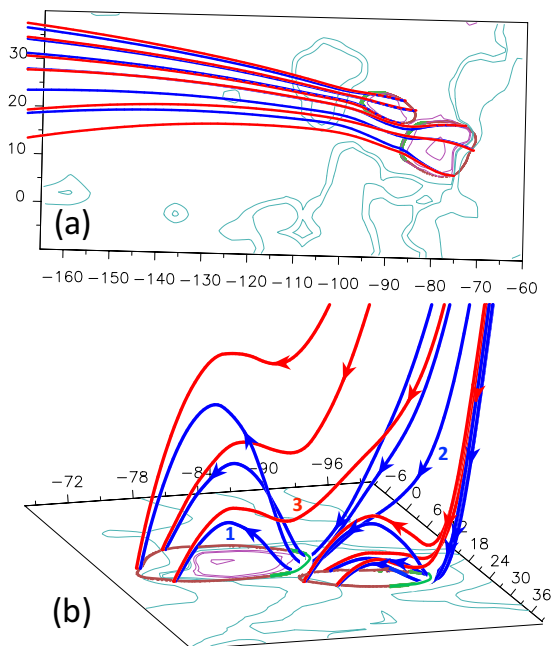
Fig. 12. Magnetic field model showing the two BPs and a set of pre-reconnected and reconnected field lines as inferred when comparing with observations. (a) The blue solid lines would correspond to the situation before reconnection, while the set of red continuous lines issued from the separatrix located at the photospheric level would correspond to the lines after reconnection. This panel is shown in the observer's point of view. (b) Same set of field lines as in panel (a) drawn from a different perspective so that the field connectivity becomes clear. We have also added arrows to the computed lines to indicate the direction of the magnetic field and numbers to some of them to explain how reconnection can proceed (see Sect. 5.2.2). The height of these field lines has been multiplied by a factor of four so that they can be clearly distinguished. The conventions for the field isocontours, axes, BPs, and separatrices are the same as in Fig. 10
