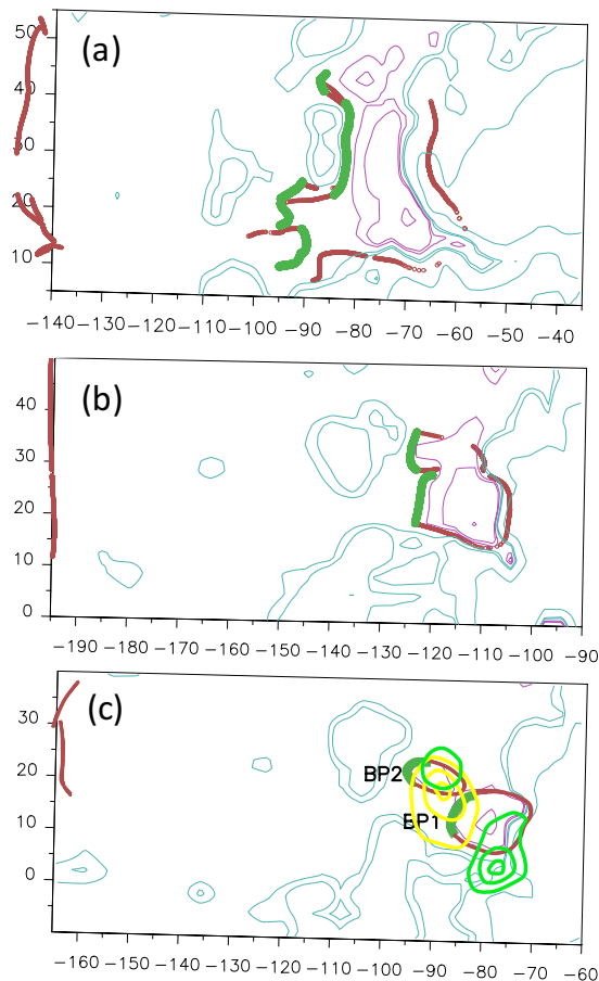
Fig. 10. Magnetic field models showing the location of the BPs and the intersections with the photosphere of their associated separatrices from 21 to 23 October 2003. (a) Corresponds to the MDI map at 20:47 UT on 21 October, (b) to the MDI map at 14:23 UT on 22 October, and (c) to that at 01:35 UT on 23 October. The later is the closest in time to the events we analyze in detail in this article. In panel (c) we have labeled the BPs as BP1 and BP2 and overlaid the RHESSI contours shown in Fig. 4d (light green contours correspond to the 50–100 keV range and yellow ones to the 10–15 keV range). The three panels are shown from the observer’s point of view. The inclination of the sides of the boxes (defined in the local frame) indicates that the AR was not at CM. BPs are shown as the thickest green continuous lines, while the magenta thick continuous lines correspond to the photospheric trace of the BP separatrices. The contours correspond to \pm 50 G, \pm 100 G, and \pm 500 G (magenta (cyan) for positive (negative) field values) and the axes are in Mm.
