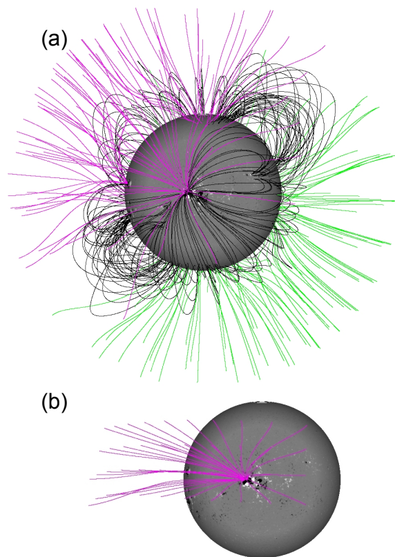
Fig. 13. PFSS model of CR 2009 with AR 10484 at CMP (Carrington longitude 5.5^\circ ). (a) Global coronal field. (b) Selection of field lines chosen in a box of 20^\circ \times 20^\circ with the AR in its center. The field-line colour convention is such that black indicates closed lines and pink (green) corresponds to open lines anchored in the negative-polarity (positive-polarity) field.
