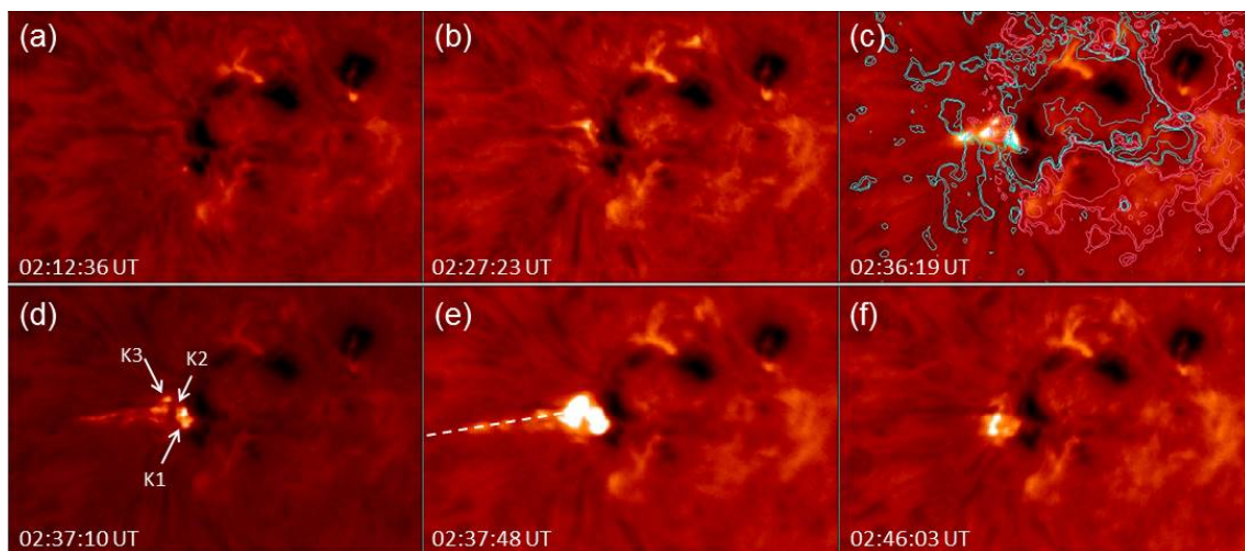
Fig. 6. Evolution of the flare in H\alpha . Three magnetic field contours ( \pm 50 , \pm 100 , and \pm 500 G) of the closest in time MDI map have been added to panel (c) in continuous magenta (cyan) line for positive (negative) field. The three brightest kernels have been labelled as K1, K2, and K3 in panel (d). All images have a FOV of 290 per 200'' , similar to that of Fig. 2 and Fig. 4. The white dashed line in panel (e) indicates the direction along which the height-time measurements in Fig. 7 are performed.
