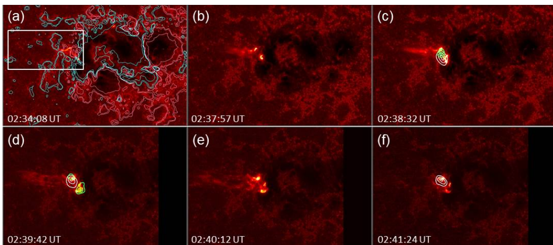
Fig. 4. Sequence of TRACE 1700 Å images overlaid by co-temporal RHESSI X-ray contours. The yellow contours correspond to the 10–15 keV range, while the light green contours to the 50–100 keV one. The integration time for each RHESSI image is 1 min. The contour levels are 40%, 70%, and 95% of the peak flux in each image. We have overlaid the same isocountours of the MDI magnetogram at 01:35 UT, shown in Fig. 2e, to panel (a) in continuous magenta (cyan) line for positive (negative) field. The field of view is the same as the one shown in Fig. 2e and has been kept as such even when TRACE FOV size changed (see the black band to the west of panels (d), (e), and (f) and explanations in the text). The white rectangle in panel (a) indicates the FOV shown in Fig. 10c, Fig. 11a, and Fig. 12a.
