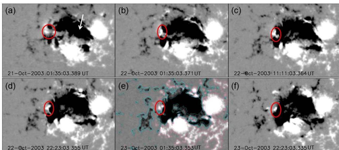
Fig. 2. Magnetic field evolution at the photospheric level. Panels (a)–(f) show the LOS magnetic field evolution as seen with MDI. We have marked with an arrow the location of a major negative sunspot around which a northern sunspot rotated from the north-east to the south-west. The ellipses indicate the approximate location of the flare and jet activity along those days. The images are derotated to Sun center and the size of the field of view (FOV) is 290 per 200". The images have been saturated below (above) -500 G (500 G). We have added three contours to panel (e) at \pm 50 , \pm 100 , and \pm 500 G in magenta (cyan) for positive (negative) values.
