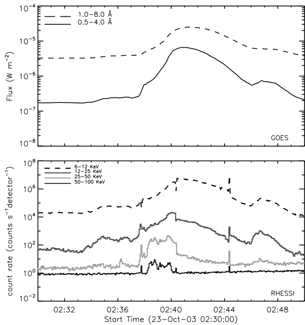
Fig. 3. GOES and RHESSI light curves of the M2.4 flare. RHESSI count rates are averaged over every 4 sec. To allow for the comparison of these curves, the RHESSI count rates are scaled by factors of 1, 1/5, 1/10, and 1/60 in the energy bands 6–12, 12–25, 25–50, and 50–100 keV, respectively.
