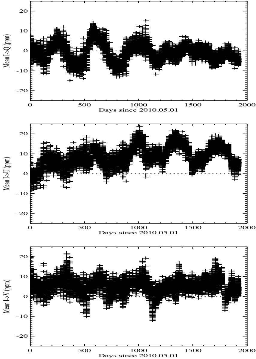
Figure 5. Plots of the mean of the telescope polarization terms in parts per million after the standard correction has been applied as a function of time. Only results for the first day of each month between May 2010 and August 2015 are shown. The means are calculated inside a radius of 1741 pixels, corresponding to roughly 0.93R .
