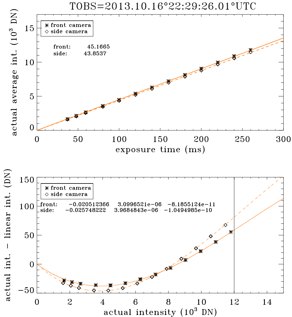
Figure 1. Results of the non-linearity analysis for the front and side cameras for 16 October 2013. The top panel shows the measured intensity vs. exposure time. The bottom panel shows 3rd-order polynomial fits to the residual as a function of intensity. A typical HMI exposure is about 140 ms.
