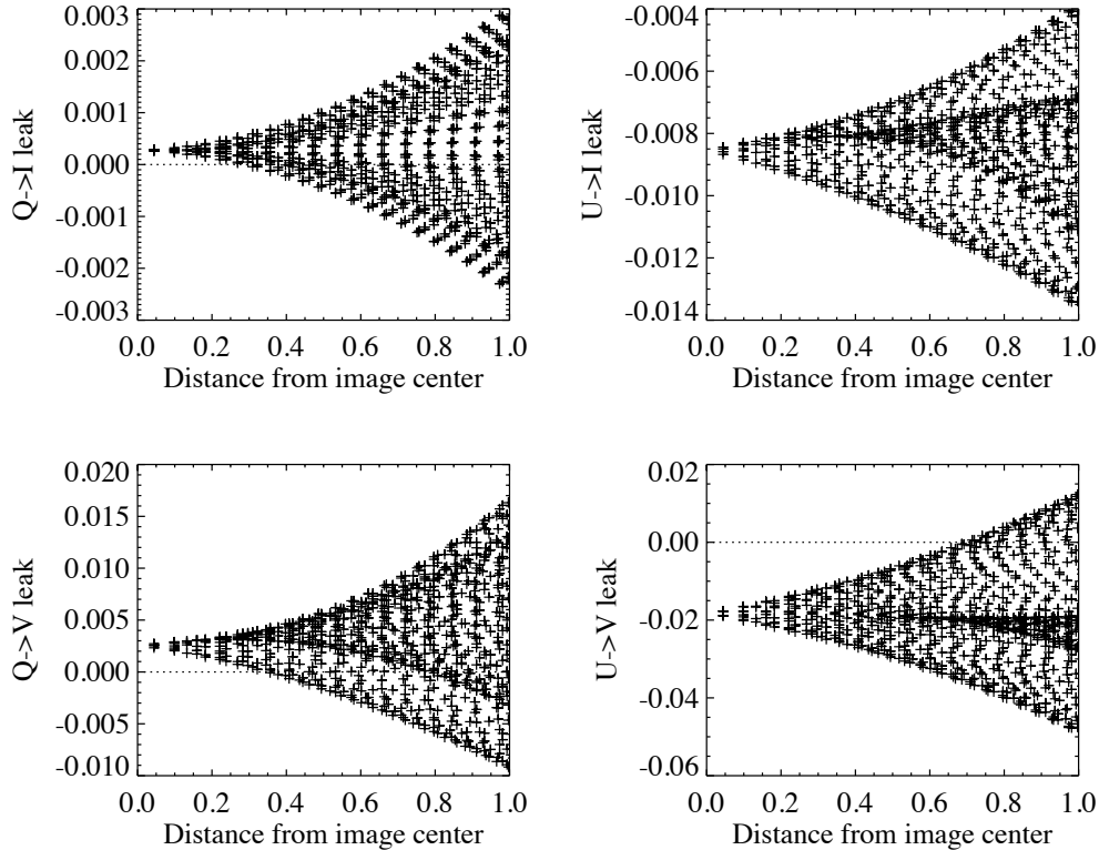
Figure 8. Computed leaks from the linear polarization into the intensity and circular polarization. Points from the entire CCD are plotted as a function of distance from the image center. The model was calculated for a polarization selector temperature of 22.5 C, representative of the mission. As mentioned in the main text, the telescope temperature is not used.
