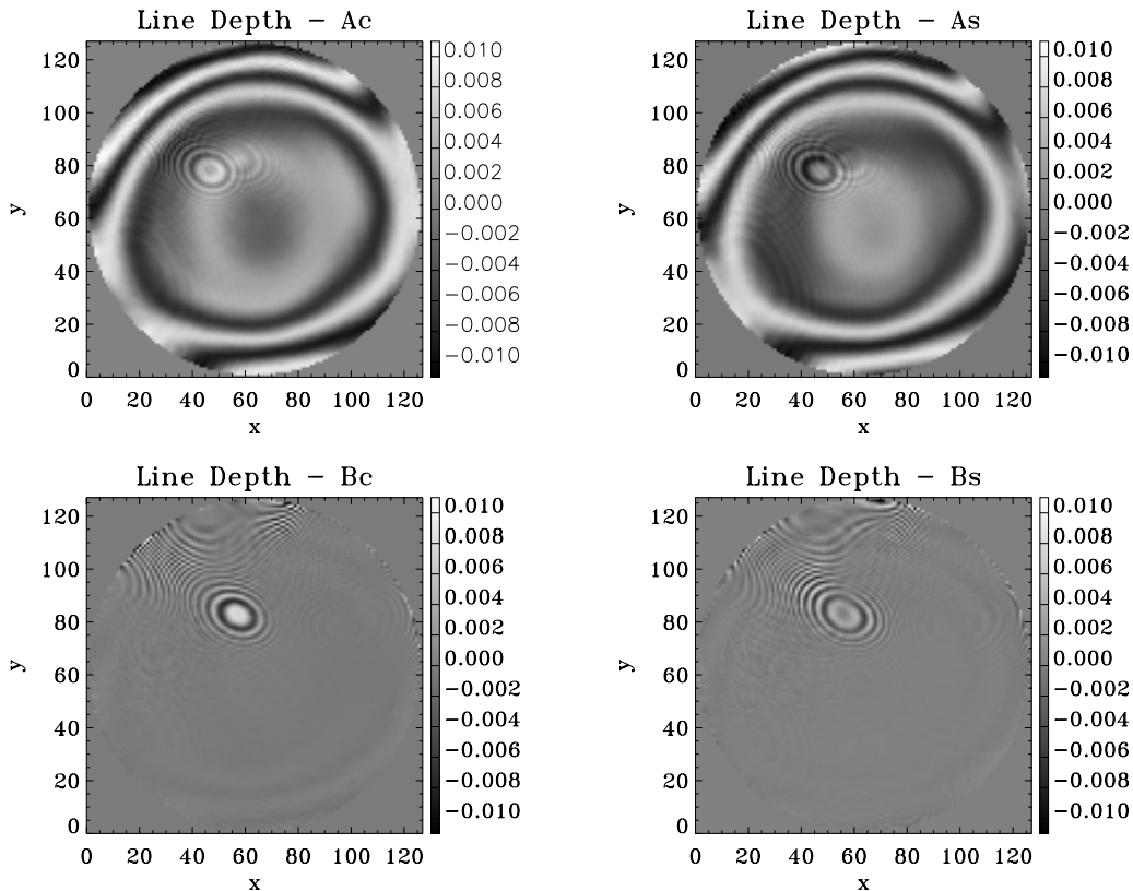
Figure 10. The larger- and smaller-scale fringe terms, A_C , A_S , B_C and B_S , determined as described in the text according to Equation 2 that are used to remove interference fringes in the phase maps. The values shown are for line depth for Calibration13 (Section 2.9.3).
