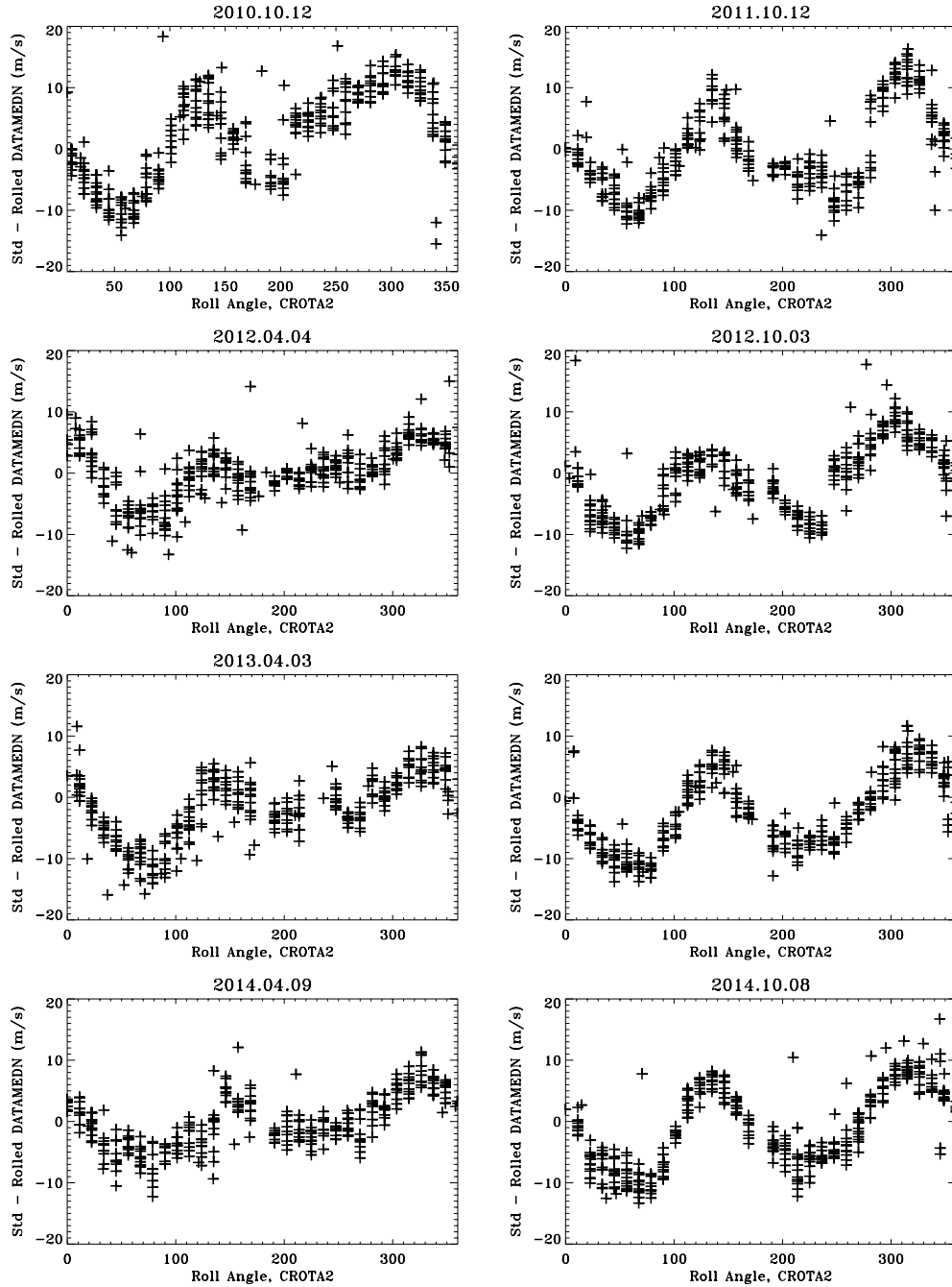
Figure 17. The dependence on roll angle of the corrected full-disk median velocity during several roll maneuvers. Plotted as a function of roll angle is the difference between the corrected full-disk median velocity, DATAMEDN, measured during the spacecraft roll and the velocity measured at the same OBS_VR when the spacecraft was not rolled. Note that the nominal CROTA2 for HMI is \approx 179.93^\circ . The panels show results for eight SDO rolls from October 2010 to October 2014. There is a systematic dependence on roll angle at the \pm 10 \text{ m s}^{-1} level. Curves in October and April are a little different, owing to the difference in the range of OBS_VR, as shown in Figure 14.
