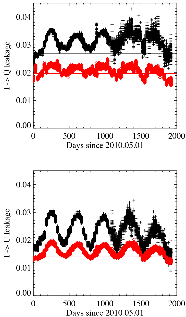
Figure 7. The top plot shows parameters for the polarization-PSF leakage from I to Q, while the bottom plot shows the I to U polarization-PSF leakage. Black pluses show the central pixel in the kernel suggesting that about 2 – 3% of the intensity signal leaks into the same pixel in Q and U. Because the sum of the kernel is zero, an equivalent negative signal leaks into other nearby pixels. Red diamonds indicate the norm of the other elements. The smaller telescope polarization term is shown in Figure 5.
