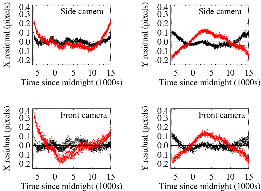
Figure 3. Residuals from the fit of the ephemeris data to the measured positions of Venus. Red points show the results using raw data, while the black points use the distortion-corrected data. The top panels show the x and y residuals for Camera 2 (the side camera) and the bottom for Camera 1 (the front camera). Times are given in thousands of seconds relative to 0 UT on 6 June 2012. The side camera observed only continuum intensity in linear polarization.
