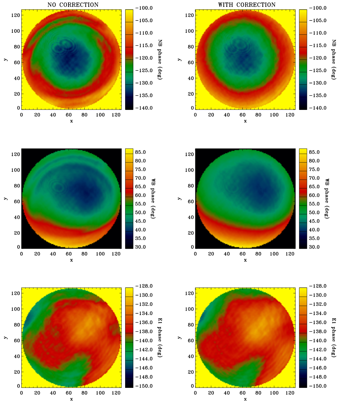
Figure 9. Phase maps for the HMI tunable filter elements. From top to bottom the rows show phase maps of the narrow-band Michelson, wide-band Michelson, and E1 Lyot element. The two columns illustrate the impact of the CalMode interference fringes on the phase maps. Panels on the right show the corrected maps.
