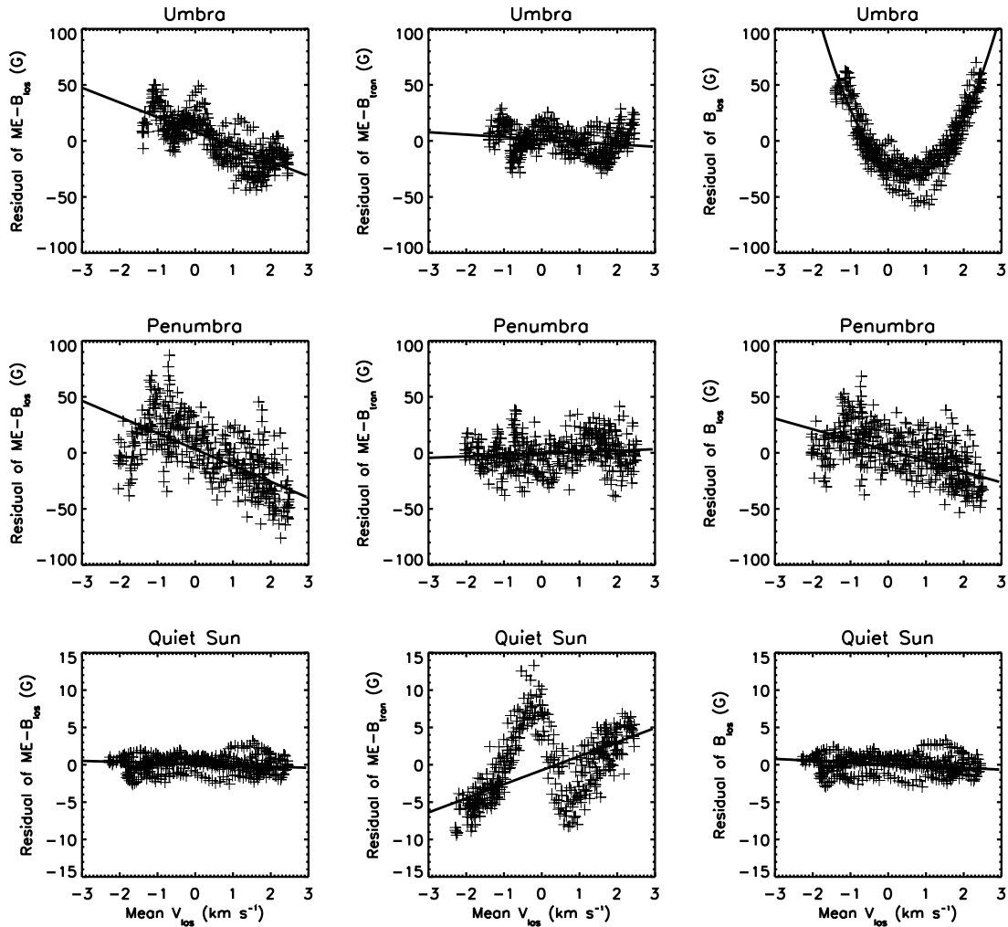
Figure 18. Scatter plots show how the measured magnetic field depends on velocity for regions of different field strength. The panels show the magnetic field residual, which is the difference between the measured field and a four-day polynomial fit (see text for details) versus velocity. From top to bottom the rows show umbra ( \approx 2500 G), penumbra ( \approx 1300 G), and a quiet Sun region ( \approx 100 G). Pixels are actually selected by intensity (see text). Panels from left to right show the line-of-sight component of the full vector magnetic field, the transverse component of the vector field, and the line-of-sight field derived using MDI-like algorithm. All filtergrams are from the side camera. The curve in the top right panel is a second-order polynomial fit to the data; solid straight lines in the other panels are linear fits. Note the difference in scale in the quiet-Sun panels in the bottom row.
