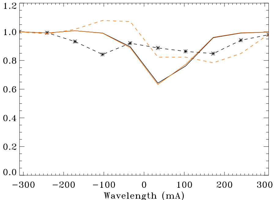
Figure 23. LCP (black lines) and RCP (red lines) components of the Fe I line profile in a pixel within a sunspot umbra (dashed lines) and in a quiet-Sun pixel (solid lines). Results are from a ten-wavelength observables sequence taken on 24 October 2014. Intensity units are normalized to the value of the intensity at -310 mÅ.
