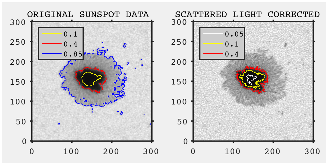
Figure 27. A cropped filtergram image containing a sunspot from the HMI side camera taken on 18 November 2013 is shown at left. The corresponding deconvolved image, with scattered light removed, is shown at right. The axes are labeled in 0.5'' pixels. Colored contours indicate the fraction of the quiet-Sun continuum intensity. The dark core of the sunspot changes from 5.5% of the nearby quiet-Sun continuum intensity in the original image to 3.3% in the deconvolved image. The inferred minimum temperature changes from 3370 K in the original to 3140 K in the deconvolved. The granulation contrast doubles; the standard deviation of the intensity in the quiet-Sun region is 3.7% of the average in the original vs. 7.2% in the deconvolved image.
