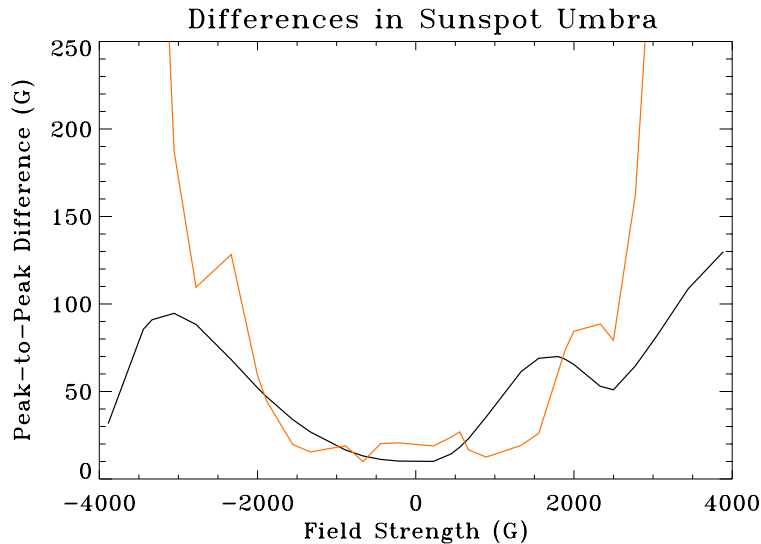
Figure 19. Computed peak-to-peak difference in the LoS magnetic-field strength returned by the observables algorithm as a function of model field strength, for the Doppler velocity ranging from -2016 to +1860 \text{m s}^{-1} . That range is typical of the daily Sun-SDO orbital velocity. The black curve shows the field-strength variation for the MDI-like algorithm. The red curve is for a least-squares fit using a Voigt profile.
