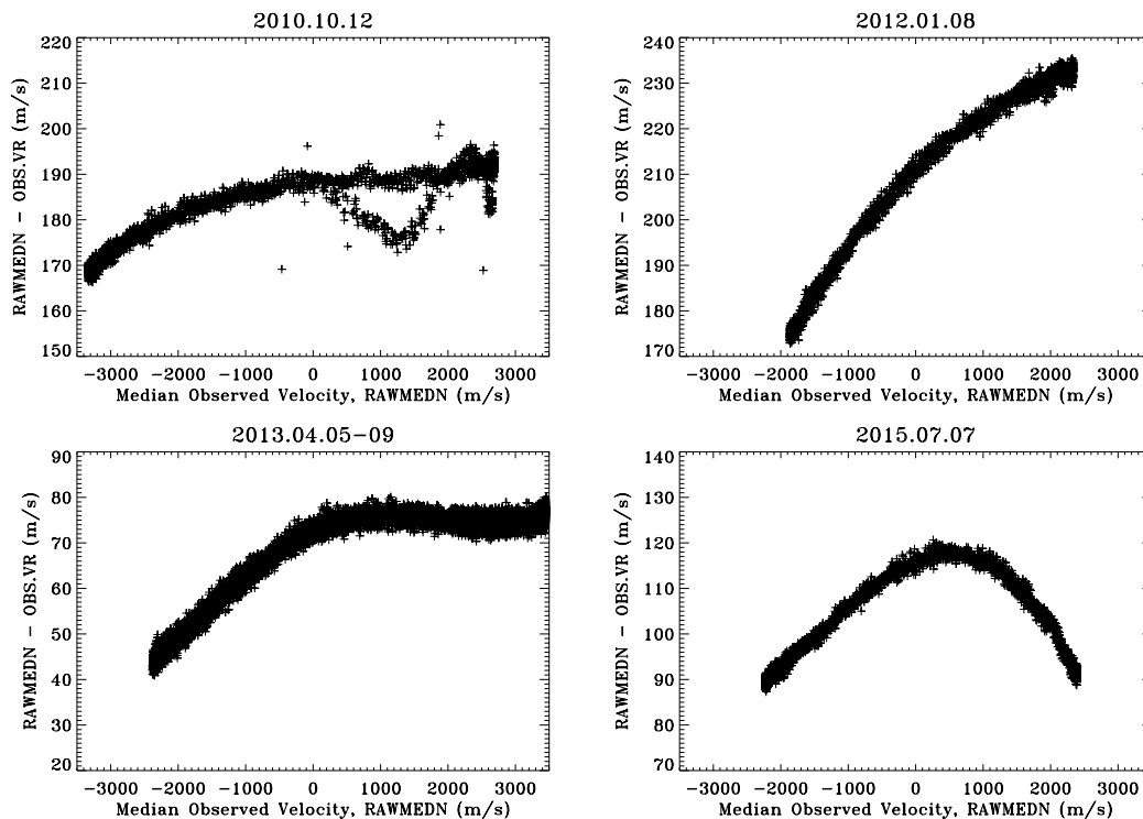
Figure 14. Median Doppler velocity returned by the line-of-sight algorithm prior to applying the polynomial velocity correction for several intervals during the course of the SDO mission. The panels show the difference between the median velocity observed in the inner 99% of the disk, RAWMEDN, and the known Sun-SDO radial velocity, OBS_VR, as a function of RAWMEDN. The three panels clockwise from the upper left show different 24-hour intervals; the lower-left panel shows five consecutive days. Note the difference in the observed range of RAWMEDN at different times of year. The upper-left panel shows observations on 12 October 2010 during which the SDO spacecraft completed a roll maneuver. The roll starts at \sim 18 UT and takes place mostly during an interval of positive RAWMEDN, after local noon. During non-roll times the difference between RAWMEDN and OBS_VR for a given RAWMEDN lies within a very narrow band of about 5 \text{ m s}^{-1} . During roll maneuvers the median velocity varies systematically, as is better illustrated in Figure 17. The lower left panel shows the difference over a five-day interval in April 2013. While slightly broader than the one-day plots, this panel demonstrates the slow evolution of the daily velocity pattern.
