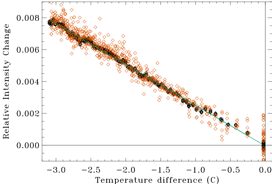
Figure 25. Dependence of the HMI front-camera CCD gain on temperature difference. The plot shows the difference in the corrected median intensity as a function of detector-temperature difference for pairs of filtergrams with identical filter tuning and the same Sun-SDO velocity on 28 September 2011. The filtergrams represented by darker black diamonds had higher overall intensities due to the tuning of the Lyot filter, and therefore less noise. The trend line is the result of a linear regression. See text for details.
