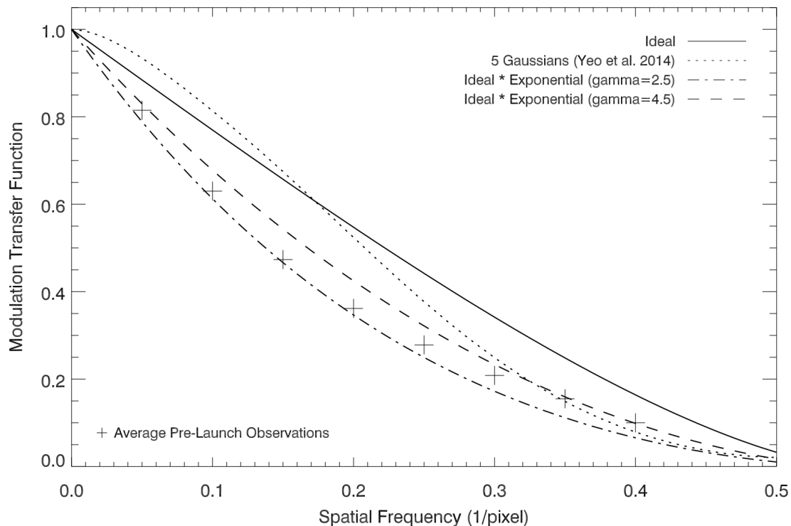
Figure 26. The ideal MTF is shown as a function of spatial frequency. Also plotted are two MTFs that are the ideal OTF multiplied by a simple exponential with \gamma = 2.5 and \gamma = 4.5 . The Yeo et al. (2014) MTF is overplotted, as is an MTF determined by the ideal multiplied by an exponential function (Equation 20). The symbols represent the average of three of the ground based curves observed during instrument calibration, as reported in Wachter et al. (2012).
