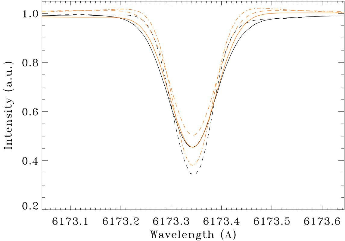
Figure 13. Different FeI line profiles used for the calibration of HMI. Three synthetic profiles are shown in red and two observed line profiles (in black). The solid black is from the NSO Solar Atlas and the dashed black is from Mount Wilson Observatory. The solid red is the profile used for HMI calibrations from May 2010 - January 2012, red dashed is January 2012 - January 2014, and red dot-dashed is after January 2014. For ease of comparison each curve has been divided by the nearby continuum intensity for that instrument.
