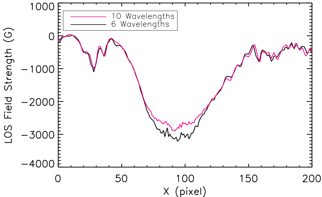
Figure 24. Comparison of inversion results of VFISV for the calculated line-of-sight component of the vector magnetic field — cosine of the inclination angle times the field strength — derived from six- and ten-wavelength observable sequences. We show a cut across the umbra of the sunspot in NOAA AR #12192 on 24 October 2014. A 75-second-cadence observables sequence with ten wavelengths rather than the usual six was run for an hour that day.
