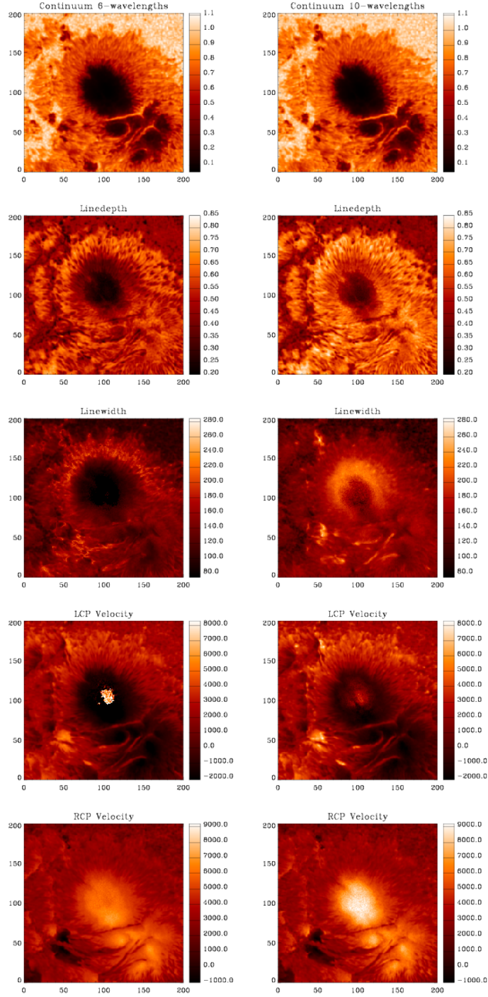
Figure 22. LoS observables returned by the MDI-like algorithm based on observations at six and ten wavelengths in different columns. Results are derived from a ten-wavelength sequence taken on 24 October 2014 for NOAA AR #12192. The color bars for each quantity in the left and right columns are the same.
