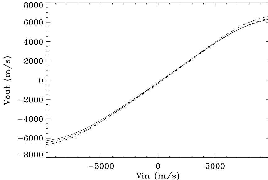
Figure 12. Sensitivity table for the first Fourier coefficients determined for the central CCD pixel on the front camera. The x axis shows the input solar velocity and the y axis shows the output velocity computed with the MDI-like algorithm. The lines show sensitivity curves for three of the six calibration tables used during the HMI mission. The solid line shows the values from the beginning of the mission determined with Calibration version 11. The dotted-line shows the sensitivity calculated using Calibration version 12 starting in early 2012, and dashed line shows the result after the retune in 2015 using version 13. The inverse of this table is used to determine the solar inputvelocity from the raw output velocity determined with the MDI algorithm.
