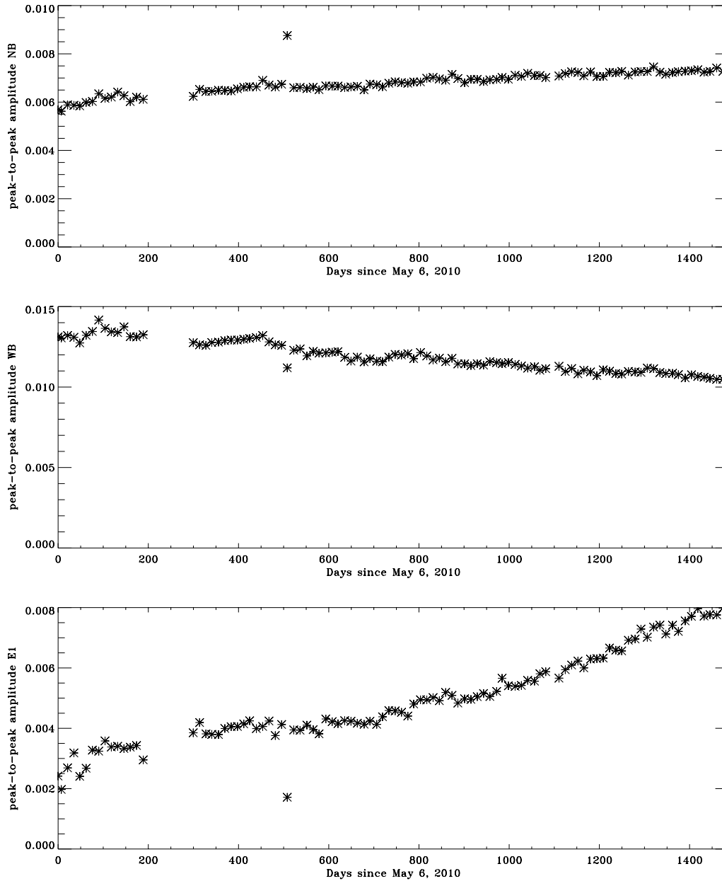
Figure 11. Peak-to-peak amplitudes of the tunable-element I-ripple for the first \sim 1500 days of operation. From top to bottom the panels show the amplitude as a fraction of the transmitted intensity in the Narrow-Band Michelson, the Wide-Band Michelson, and the tunable Lyot element, E1. The measured amplitudes of the I-ripple are consistent with those measured before launch (Couvidat et al. , 2012b).
