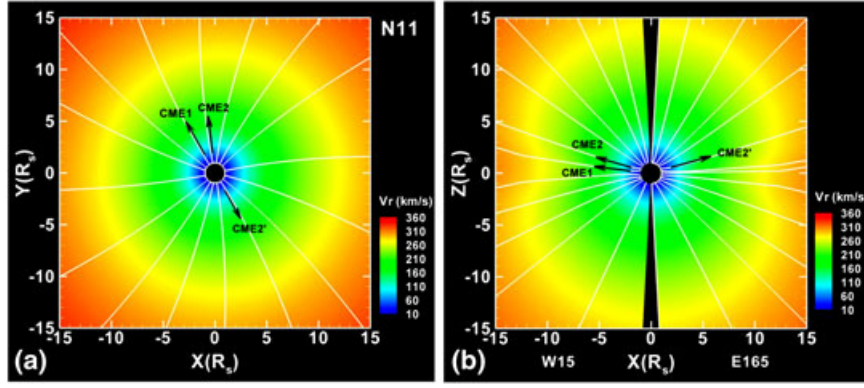
Figure 1. Background solar wind in (a) the plane of the latitude of N11^\circ and (b) the meridian plane passing through the longitude of 15^\circ W and 165^\circ E . The white lines show the magnetic field lines. The propagation directions of CMES to be introduced are indicated by arrows.
