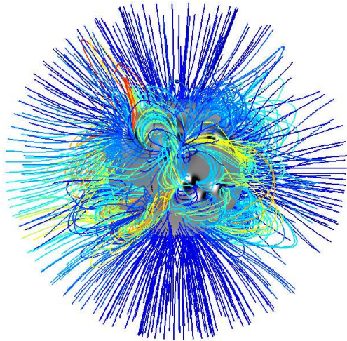
Figure 4. Magnetofrictional field model for case B for 2011/02/16, shown from the Earth perspective on the 14th. The field lines are colored depending on the angular spacing of their endpoints in latitude and longitude (regardless of whether they close on the surface or on the source surface) to reduce confusion in closely packed regions and in flux-rope configurations.
