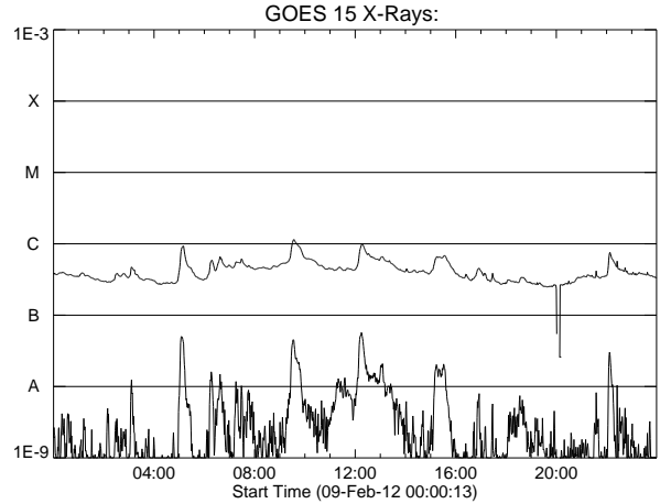
Figure 26. GOES light curve for case I, 2012/02/09.
