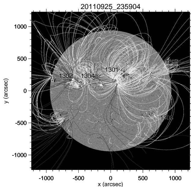
Figure 7. HMI magnetogram, PFSS extrapolation, and AR numbers for case C, 2011/09/25.
