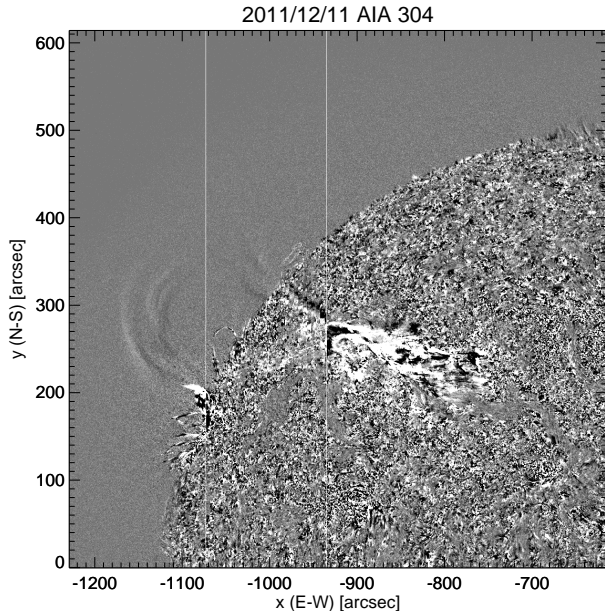
Figure 21. Composite running-difference image for 304 Å exposures on 2011/12/11 (case G), displaying the northeast quadrant of the Sun (summarizing the image sequence shown in the on-line Table S0 that also shows the STEREO images for comparison). This composite image highlights the connection between the on-disk and off-limb erupting regions. The figure is an assemblage of a series of running difference images, each computed for a time spacing 4 min (the image sequence can be accessed on line S20 ). To the right of the rightmost vertical white line is the difference image for 05:45 UT, for the early phases of the eruption. To the left of the leftmost vertical line is the image for 07:07 UT. Between the two vertical lines is a series of narrow strips cut out of running difference images with positions shifting from left to right with time, advancing in steps of 3 min., moving in the general direction of motion of the eruption.
