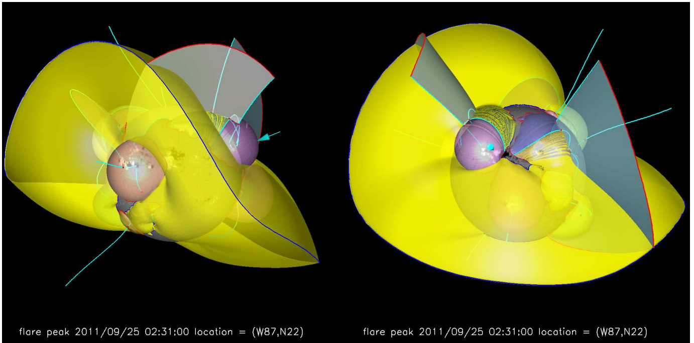
Figure 6. PFSS field topology for case C, 2011/09/25 (cf. Fig. 5 for a description of the details).
