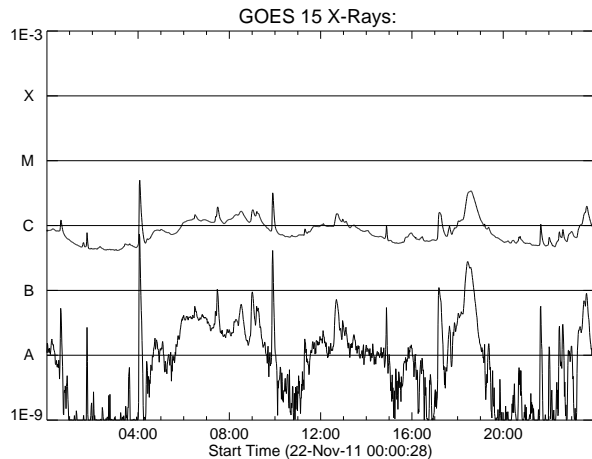
Figure 14. GOES light curve for case E, 2011/11/22.
