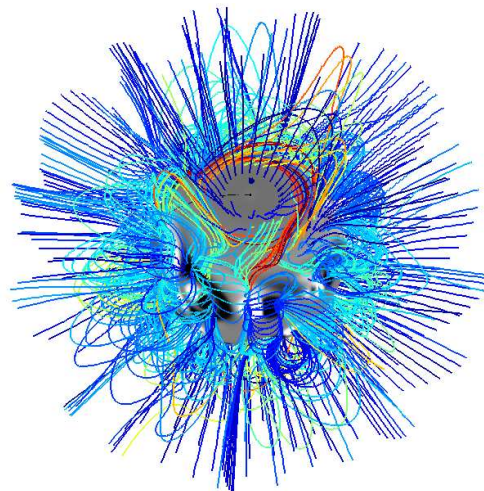
Figure 13. Magnetofrictional field model, tipped to a viewing angle of 57 degrees north latitude for case D, 2011/11/09 (cf. Fig. 4 for a description of the details).
