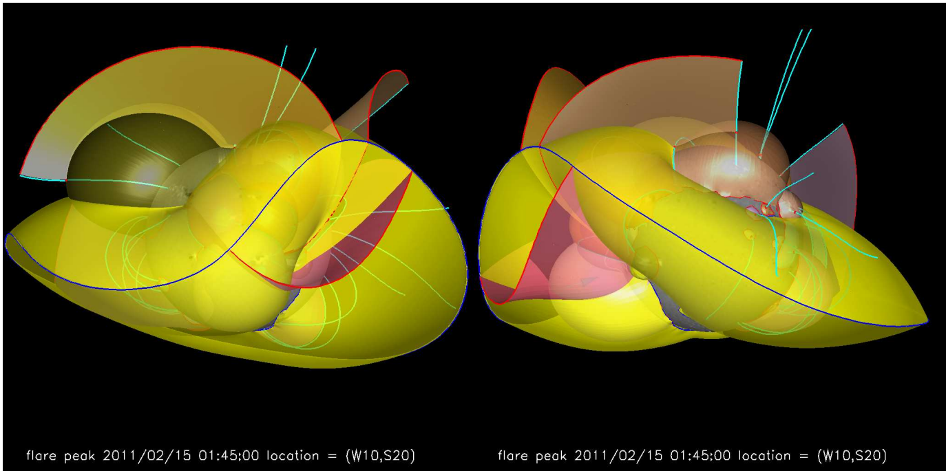
Figure 5. PFSS field topology for case B, 2011/02/15, from the perspectives of Earth and of STEREO-A. The main, yellow, surface is the PFSS helmet, i.e., the envelope of the domain in the solar corona within which all field is closed. At its cusp the radial field component vanishes, so that this cusp forms the basis of the heliospheric current sheet above. Underneath and outside it are other surfaces that are the main topological domains defined by coronal null points (red dots), with their spine field lines shown in light blue. The dark blue curve is the null line for the radial field component on the source surface (at 2.5 solar radii). The red curves are the intersections of the domes and curtains with the solar surface and source surface, respectively.
