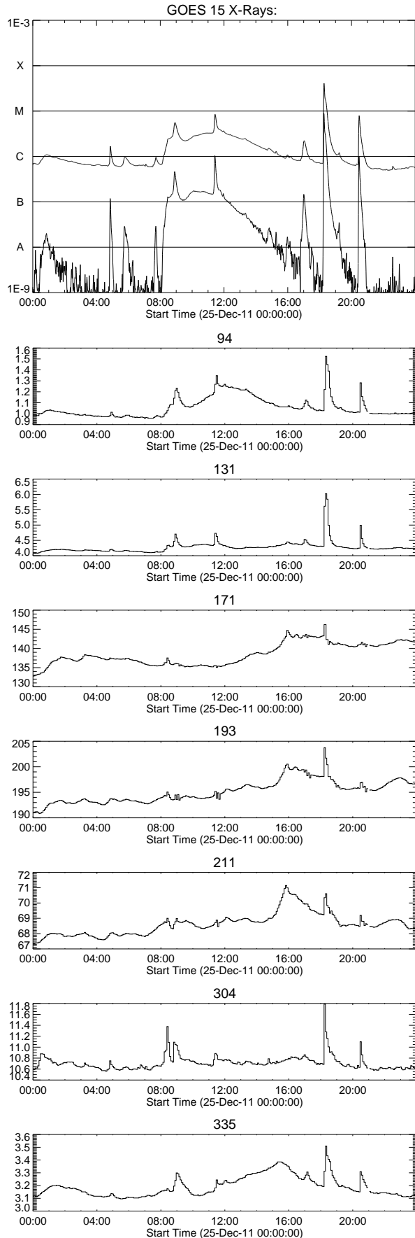
Figure 22. GOES and AIA light curves for case H, 2011/12/25 (for AIA in DN/pixel/s).
