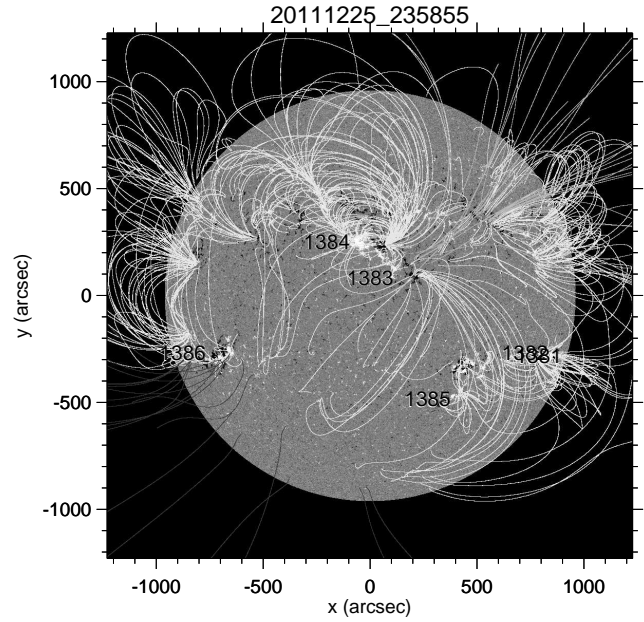
Figure 23. HMI magnetogram, PFSS extrapolation, and AR numbers for case H, 2011/12/25.
