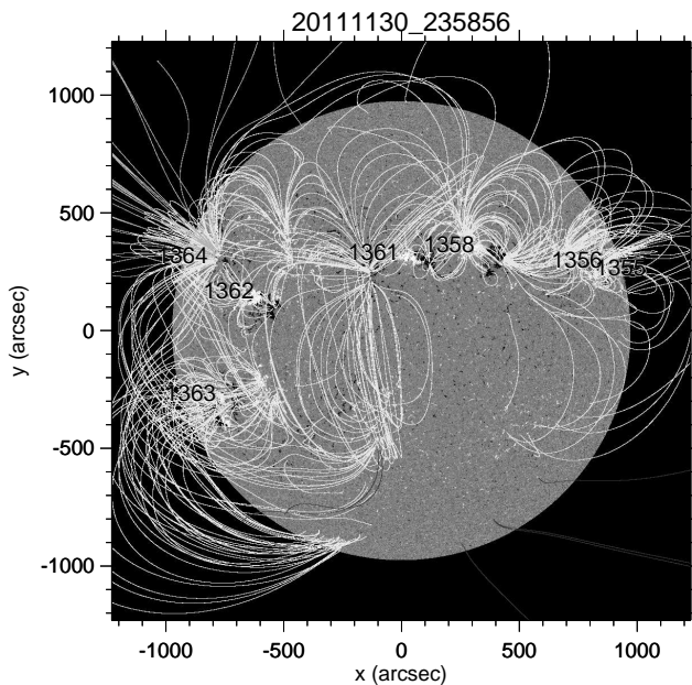
Figure 18. HMI magnetogram, PFSS extrapolation, and AR numbers for case F, 2011/11/30.
