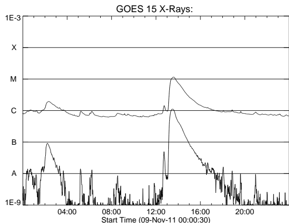
Figure 10. GOES light curve for case D, 2011/11/09.
