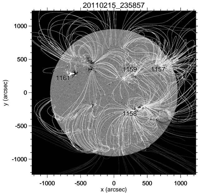
Figure 3. HMI magnetogram, PFSS extrapolation, and AR numbers (showing the last four digits, as is a common standard, here and in subsequent similar figures for other cases) for case B, 2011/02/15.
