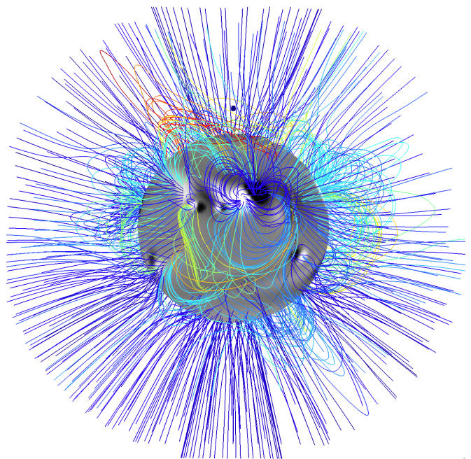
Figure 9. Magnetofrictional field model for case C, 2011/09/25 (cf. Fig. 4 for a description of the details).
