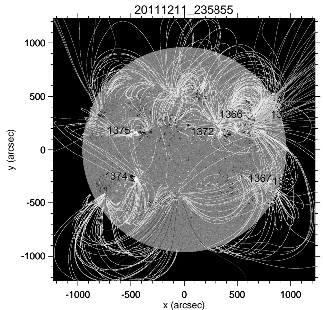
Figure 20. HMI magnetogram, PFSS extrapolation, and AR numbers for case G, 2011/12/11.
