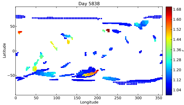
Figure 25. Flux rope positions, colored by height (see color bar, in units of solar radii), from the magnetofrictional model for case H. The Carrington longitude of disk center on 2011/12/25 is 209^\circ
