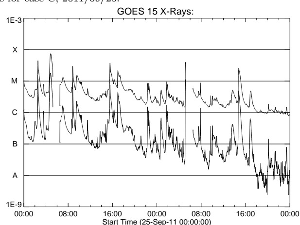
Figure 8. GOES light curve for case C, 2011/09/25.
