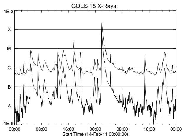
Figure 2. GOES light curve for case B, 2011/02/14-15.
