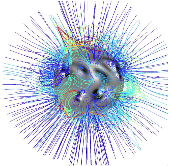
Figure 24. Magnetofrictional field model for case H, 2011/12/25, rotated eastward by 30 degrees relative to the Carrington longitude (cf. Fig. 4 for a description of the details).
