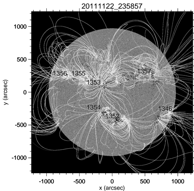
Figure 15. HMI magnetogram, PFSS extrapolation, and AR numbers for case E, 2011/11/22.
