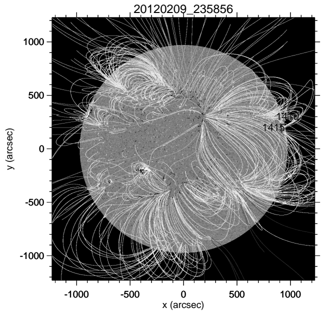
Figure 27. HMI magnetogram, PFSS extrapolation, and AR numbers for case I, 2012/02/09.
