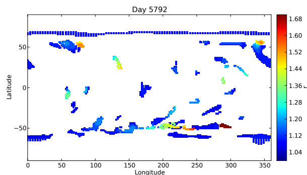
Figure 12. Flux rope positions, colored by height (see color bar, in units of solar radii), from the magnetofrictional model for case D. The Carrington longitude of disk center on 2011/11/09 is 96°.
