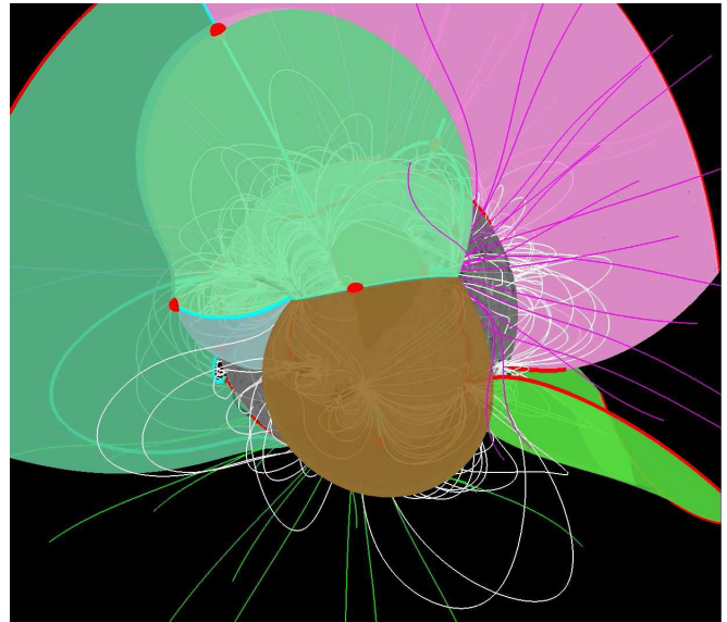
Figure 16. Partial rendering of the topological domains for the PFSS model for case E, 2011/11/22. Selected domain boundaries are shown as translucent surfaces for those separatrices associated with coronal null points (shown as red balls on the blue spine field lines).
