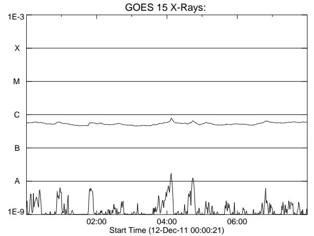
Figure 19. GOES light curve for case G, 2011/12/11.
