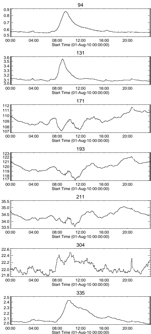
Figure 1. AIA light curves for case A, 2010/08/01 (in DN/pixel/s).
