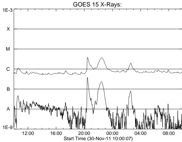
Figure 17. GOES light curve for case F, 2011/11/30.
