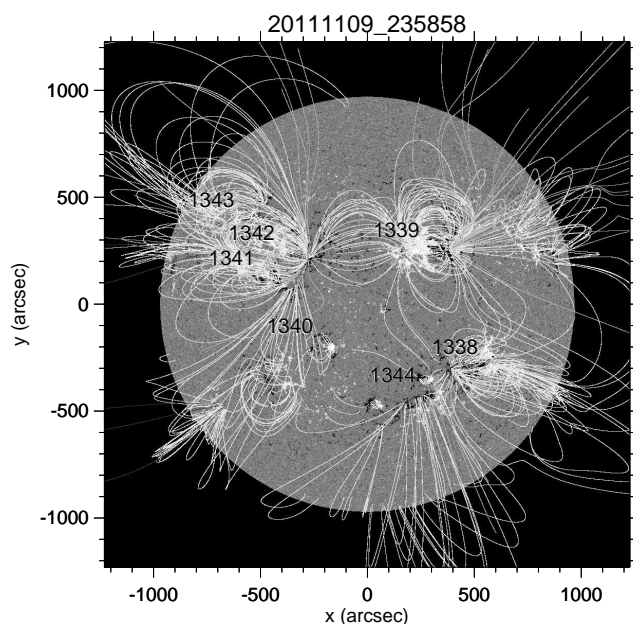
Figure 11. HMI magnetogram, PFSS extrapolation, and AR numbers for case D, 2011/11/09.
