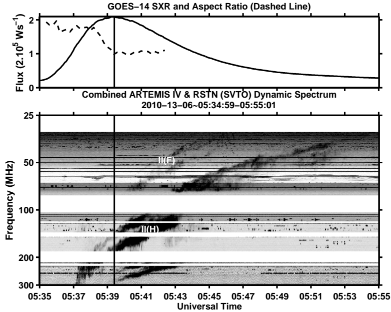
Figure 2. Top: GOES-14 SXR flux in the 0.5-4 \text{ \AA} channel and EUV bubble aspect ratio (dashed line). The vertical line at 05:39 UT marks at the transition from aspect ratio \approx two to \approx one marking the start of the EUV bubble lateral expansion phase (see Table 1). Bottom: Combined dynamic spectra of ARTEMIS IV and RSTN (San Vito) in the 25–300 MHz range; the fundamental and the harmonic of the Type-II burst are annotated with II(F) and II(H) respectively. The Type-II bands below the II(H) in the range 275–300 MHz were found to be an artefact due to the non-linear response of the ARTEMIS IV pre-amplifier which introduced an image of II(H) displaced by 100 MHz. (The horizontal black stripes are interference from terrestrial emitters; the white stripes are disturbed frequency ranges that have been suppressed.)
