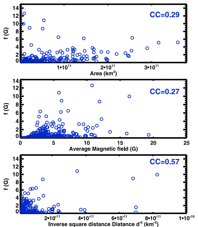
Figure 7. The individual CHIP ( f ) versus the CH parameters: area ( A ), average magnetic field ( \langle B \rangle ), and inverse square distance ( d^{-2} ) for 308 CHs on the solar disk in the 72 events during the three phases of the solar cycle 23. The correlation coefficient is the highest for f vs d^{-2} .
