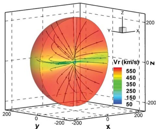
Figure 1. The calculated steady state 3-D magnetic field lines and radial velocity distribution from 2.5 to 220 R_s at 100 h. (Axis units given in R_s .)
