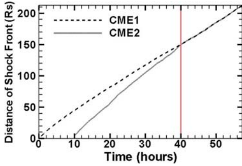
Figure 4. Comparison of the shock front heliocentric distance between the first CME (dashed line) and the second CME (solid line).
