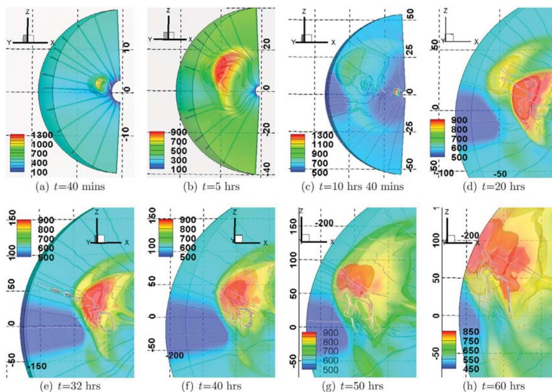
Figure 6. Three-dimensional representation of the CMES ( 140^\circ < \varphi < 180^\circ ) shown (a) 40 min, (b) 5 h, (c) 10 h 40 min (40 min after the second CME launched), (d) 20 h, (e) 32 h, (f) 40 h, (g) 50 h, and (h) 60 h after the first CME initiation. The solid rod-shaped lines are magnetic field lines, and the color codes represent the radial velocity magnitude. (Axis units given in R_s .)
