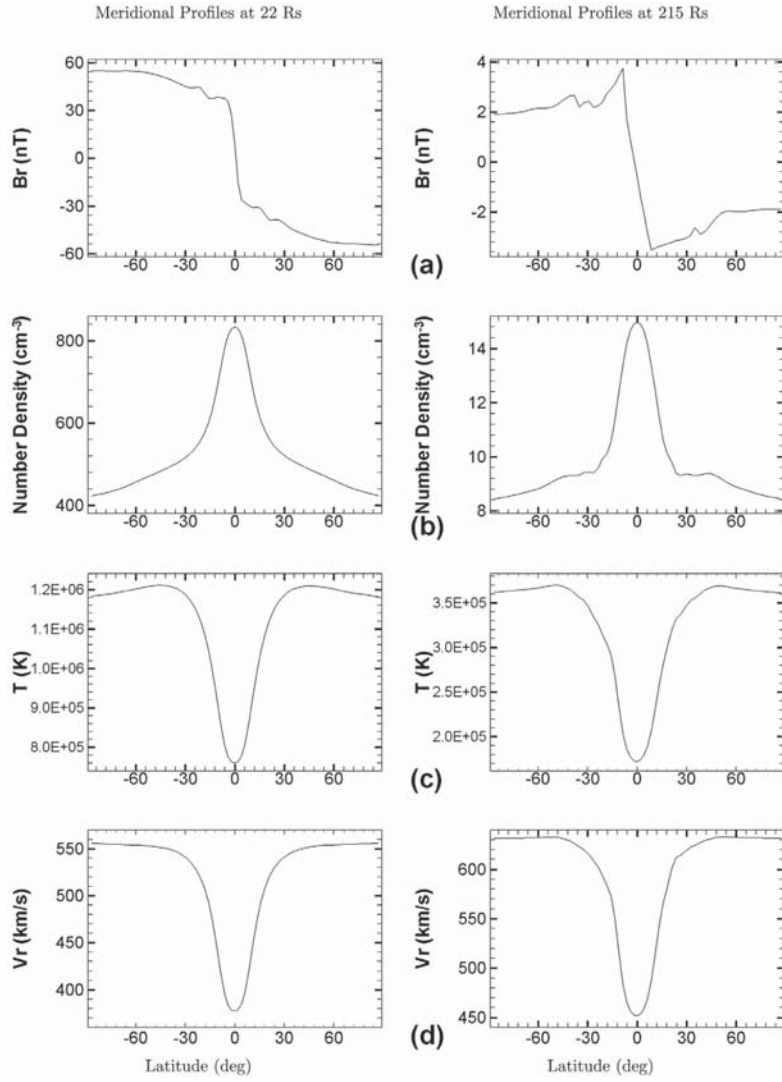
Figure 2. Profiles of (a) the radial magnetic field, (b) proton number density, (c) temperature, and (d) the radial velocity at r = 22 R_s (corona, left) and r = 215 R_s (heliosphere, right; meridional profiles at \phi = 180^\circ ).
