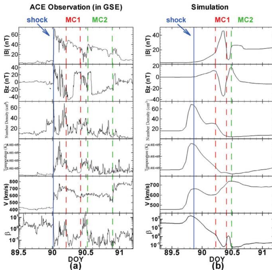
Figure 10. A comparison of the MHD simulation of the magnetic field and plasma parameters with the measured (ACE spacecraft) magnetic field and solar wind parameters at the L1 point in 2001. (a) Measured parameters by ACE, top to bottom: magnetic field strength |B| (nT), B_z (nT) at GSE coordinate system, proton density ( \text{cm}^{-3} ), proton temperature (K), velocity (km/s), and plasma \beta . (b) Simulation parameters, top to bottom: magnetic field strength |B| (nT), B_z (nT) at GSE coordinate system, number density ( \text{cm}^{-3} ), plasma temperature (K), velocity (km/s), and plasma \beta . The blue vertical solid lines indicate the arrival time at L1 of the shock, the red vertical dashed lines denote the beginning and ending of the first MC, and the green vertical dashed line denotes the beginning of the second MC.
