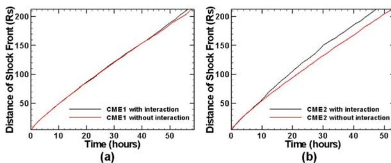
Figure 8. (a) Temporal evolution of shock front distance of the first CME with (black line) and without (red line) interaction with the second CME and (b) temporal evolution of shock front distance of the second CME with (black line) and without (red line) interaction with the first CME. For the black line in Figure 8b the time reference has been shifted by 10 h so that time t = 0 h corresponds to the initiation of the second CME.
