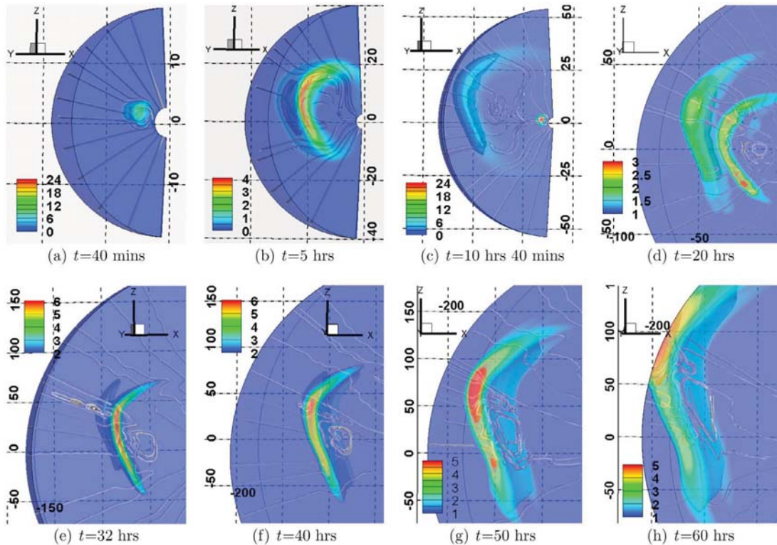
Figure 5. Three-dimensional representation of the CMES ( 140^\circ < \varphi < 180^\circ ) shown (a) 40 min, (b) 5 h, (c) 10 h 40 min (40 min after the second CME launched), (d) 20 h, (e) 32 h, (f) 40 h, (g) 50 h, and (h) 60 h after the first CME initiation. The solid rod-shaped lines are magnetic field lines, and the color codes represent the relative density ((\rho - \rho_o)/\rho_o) . (Axis units given in R_s .)
