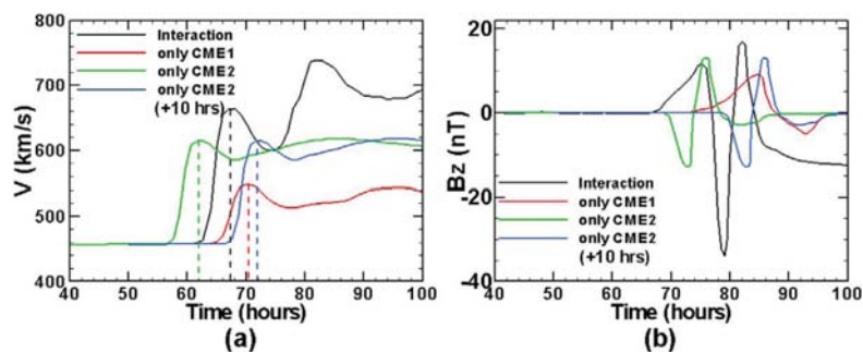
Figure 9. Temporal evolution of (a) velocity ( v ) and (b) z component magnetic field ( B_z ) at the L1 point of the double-CME case (black line), only the first CME (red line), only the second CME (initial time t = 0 h, to be compared with only the first CME case) (green line), and only the second CME shifted by 10 h (initial time t = 10 h, to be compared with double-CME case) (blue line).
