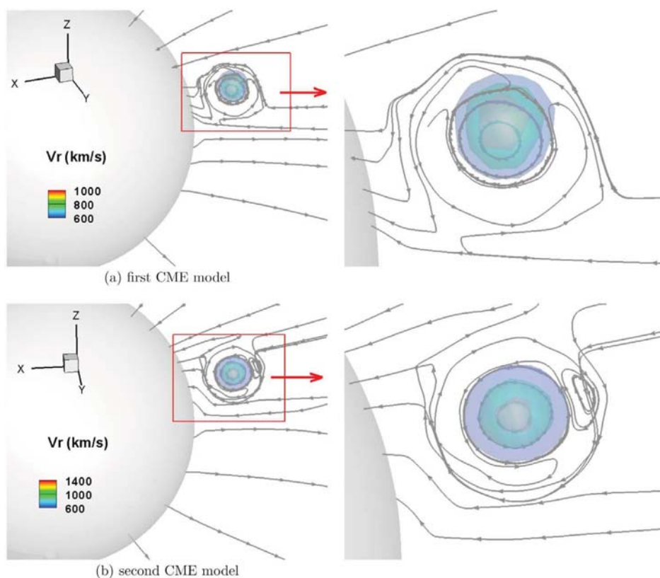
Figure 3. Three-dimensional views of the isosurface of the radial velocity v_r and the initial magnetic field lines of the CME initialization for (a) the first CME and (b) the second CME, including zooming in on the plasma blob.
