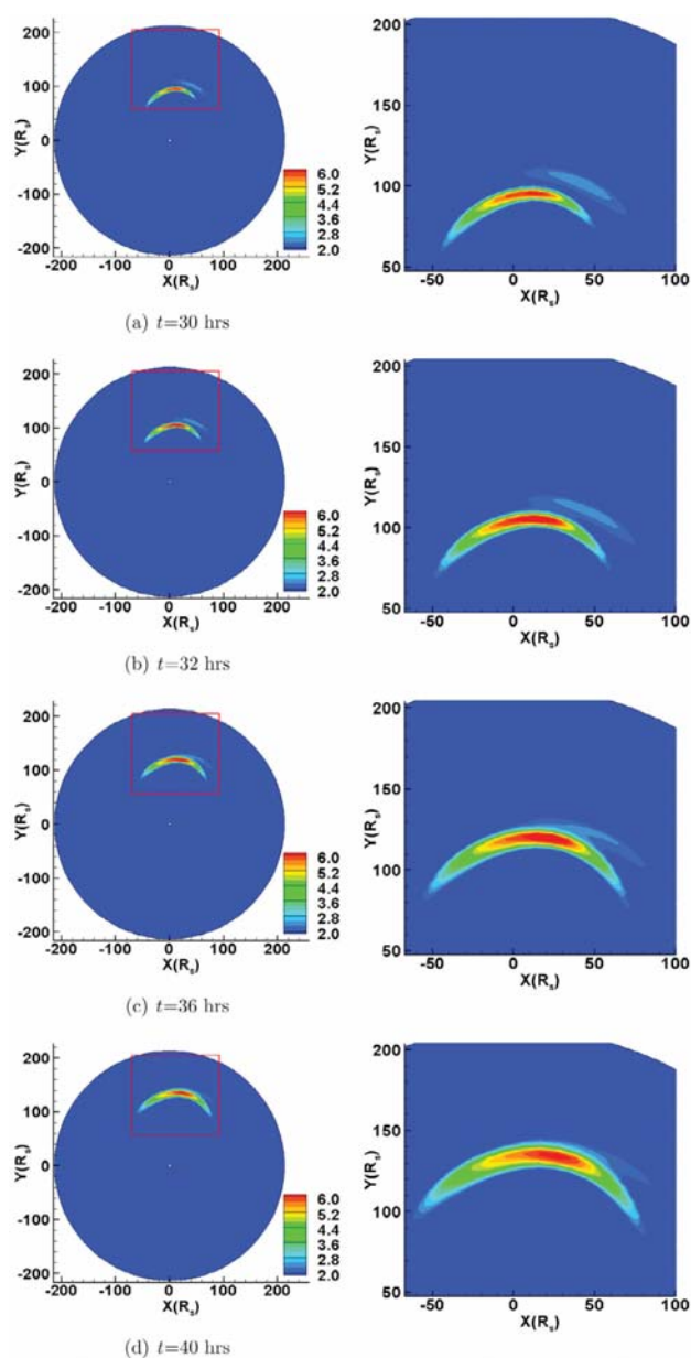
Figure 7. Evolution of the two-dimensional relative density ( (\rho - \rho_0)/\rho_0 ) contours of the constant latitude angle of \theta = 18^\circ at four consecutive times. (Axis units given in R_s .)
