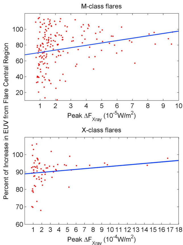
Figure 7. The dependences of percent of increase in EUV from flare central region on the strength of solar flares for both the M-class flares and the X-class flares. The solid lines represent the linear fitting.
