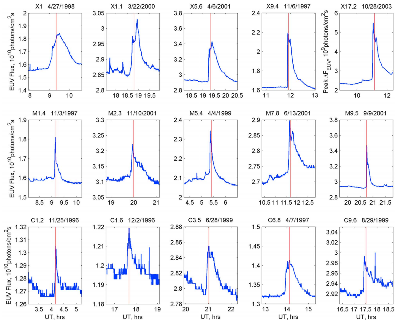
Figure 1. Sample time series of EUV fluxes during some X, M, and C class solar flares.
