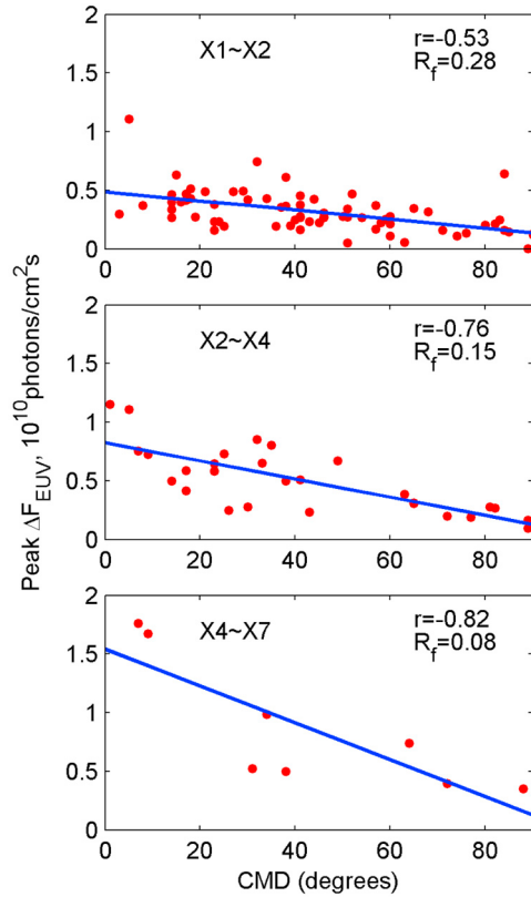
Figure 3. Dependence of the enhancement EUV flux on the values of CMD which represent the location of flares on the solar disc for X-class flares of 1996–2006. X-class flares are separated into following pieces: X1 ~ X2, X2 ~ X4, and X4 ~ X7, respectively. The solid lines represent the linear fitting. The correlation coefficient ( r ) and the ratio of peak \Delta F_{\text{EUV}} at \text{CMD} = 90^\circ to that at \text{CMD} = 0^\circ ( R_f ) are also marked in panels.
