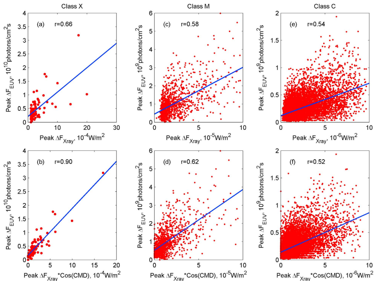
Figure 2. (a) Plots of SEM/SOHO measured peak \Delta F_{\text{EUV}} of 26–34 nm versus GOES measured peak \Delta F_{\text{Xray}} for 102 X-class flares from 1996 to 2006. (b) Same as top panels but for X-ray fluxes multiplied by \text{Cos}(\text{CMD}) . The correlation coefficients between the two fluxes are indicated in the panels. The solid lines represent the linear fitting. (c and d) For the M-class flares. (e and f) For the C-class flares.
