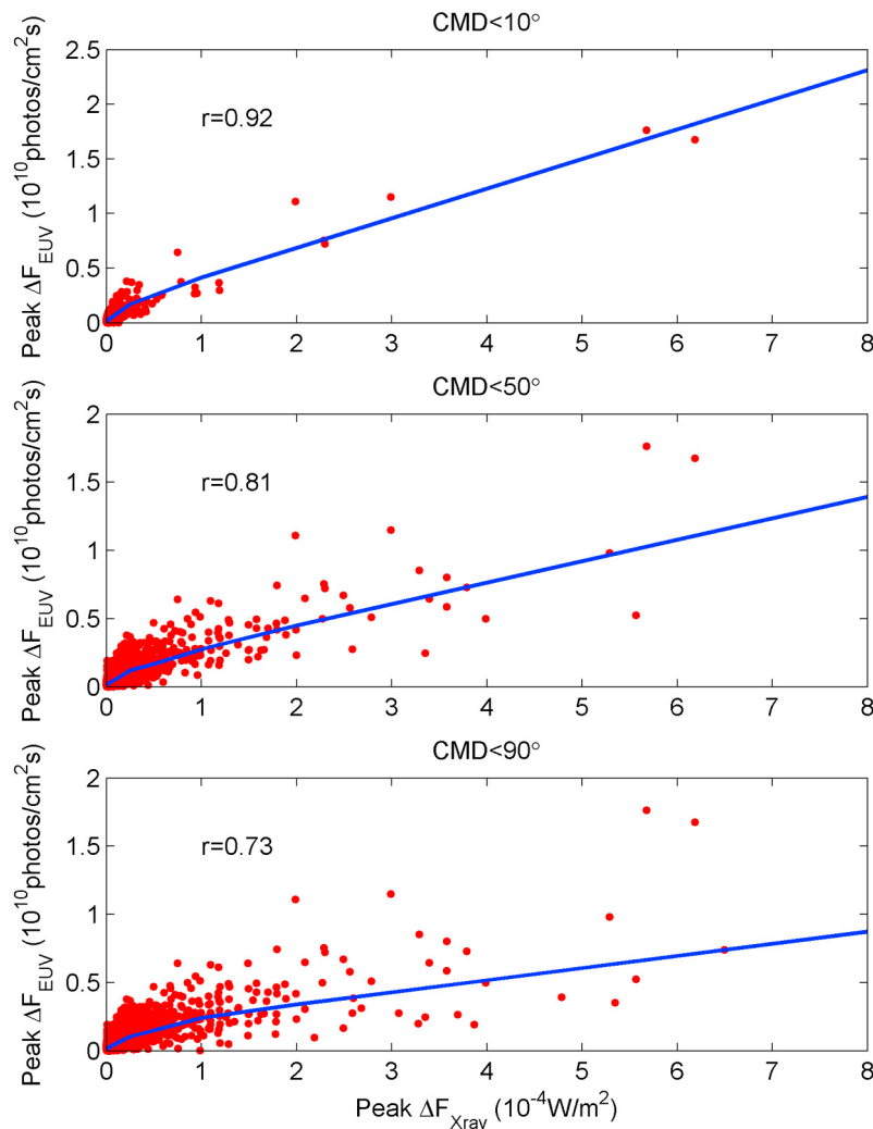
Figure 6. Plots of peak \Delta F_{\text{EUV}} versus peak \Delta F_{\text{Xray}} for solar flares with \text{CMD} < 10^\circ , \text{CMD} < 50^\circ , and \text{CMD} < 90^\circ , respectively. Solid lines are the line segment curve-fitting of the two fluxes. Their correlation coefficients are also marked in the figure.
