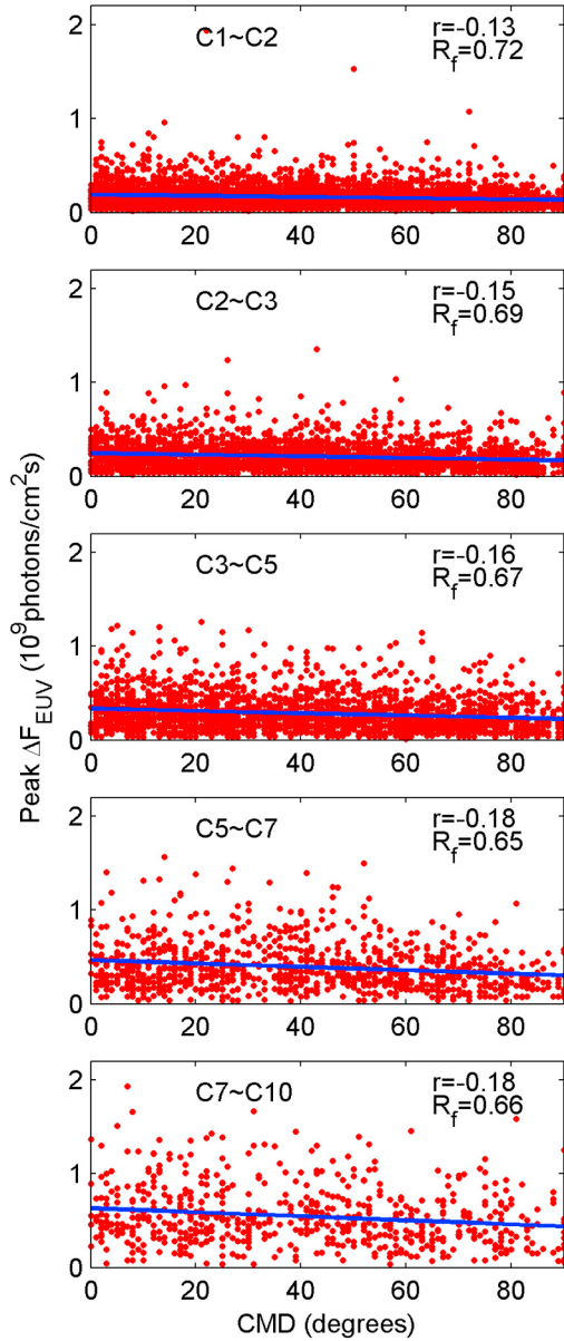
Figure 5. Same as Figure 3, but for C-class flares from 1996 to 2006. C-class flares are separated in following pieces: C1 ~ C2, C2 ~ C3, C3 ~ C5, C5 ~ C7, and C7 ~ C10, respectively.
