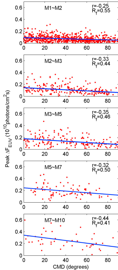
Figure 4. Same as Figure 3, but for M-class flares from 1996 to 2006. M-class flares are separated in following pieces: M1 ~ M2, M2 ~ M3, M3 ~ M5, M5 ~ M7, and M7 ~ M10, respectively.
