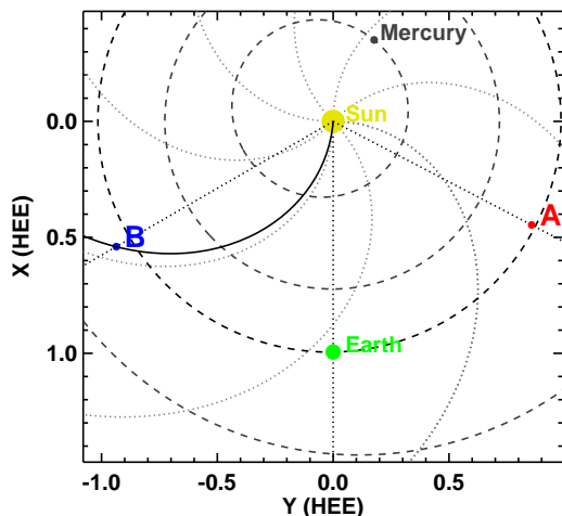
Figure 5. Solar magnetic field in the interplanetary medium represented by the Parker spiral for 2009 October 25 (in heliocentric Earth Ecliptic (HEE) coordinate system). On this day, STEREO B (marked by the blue dot B), was located near the Sun-Earth L5 point (trailing Earth by 60^\circ ). STEREO A (marked by the red dot A) was located near the L4 point. One of the spiral field lines with its foot point near the Sun center in Earth view is connected to STEREO B. If there were a coronal hole near the disk center, then this spiral would roughly correspond to a CIR and would rotate to Earth in about 4 days (neglecting the orbital motion of Earth, which is very small compared to the solar rotation).
