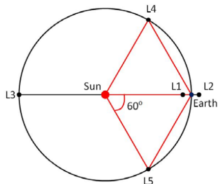
Figure 1. A sketch of the Sun-Earth system showing the five Lagrange points, L1 – L5 with respect to Earth’s orbit around the Sun. All the Lagrange points view the Sun continuously save L2, which is located on the night side of Earth. L5 is located at 60^\circ away from the Sun-Earth line, trailing Earth.
