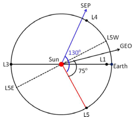
Figure 3. Average directions of Earth-affecting CMEs with respect to the Sun-L5 line marked GEO (geoeffective CMEs) and SEP (CMEs producing SEPs). Also marked is the solar hemisphere visible to L5 (L5E and L5W are the east and west limbs in the L5 view). GEO CMEs are limb CMEs in the L5 view, so they can be measured with minimal projection effects. SEP CMEs are behind-the-limb CMEs most of which can also be measured with minimal projection effects.
