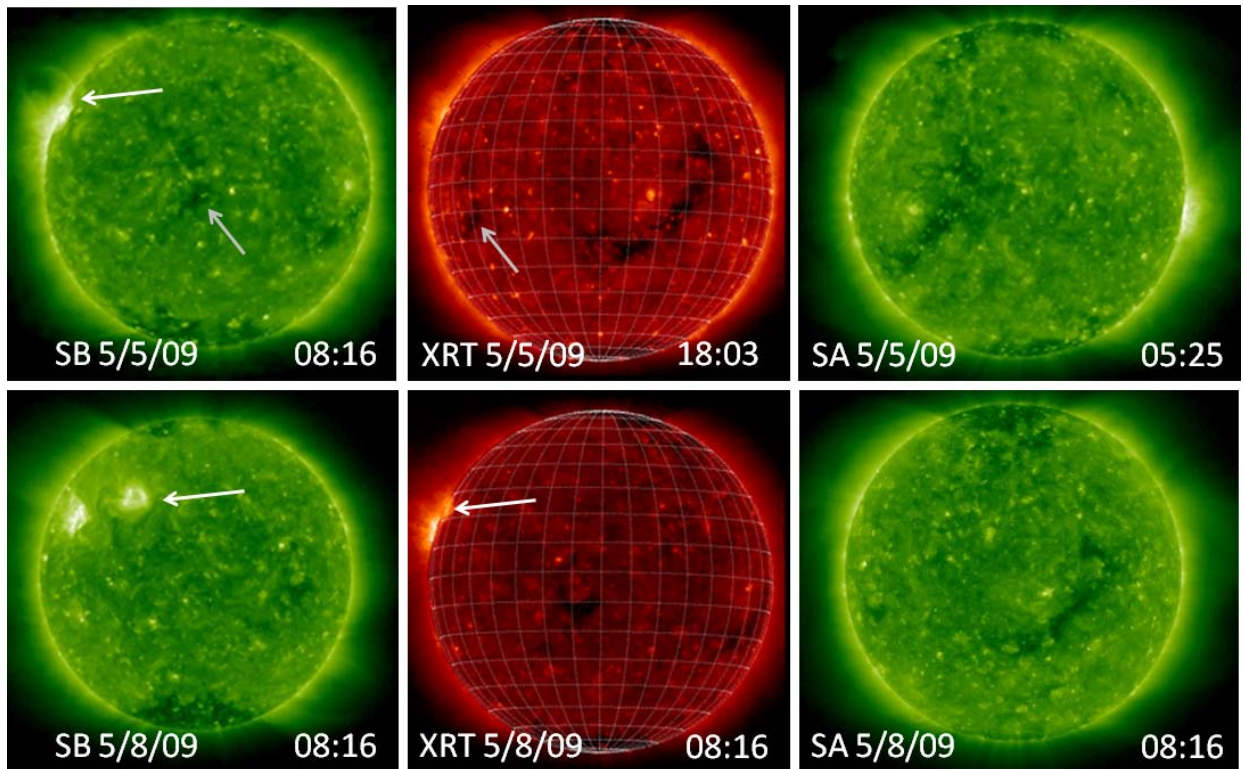
Figure 4. A set of active regions was observed by only STEREO B (SB) EUVI at the east limb on 2009 May 5. There was actually an eruption from one of these regions (pointed by arrow). The regions were not seen in Earth view (as shown by the Hinode XRT view) or STEREO A (SA) because the regions were behind the limb from these views. SB and SA were separated by 47^\circ and 48^\circ , respectively from Earth. The regions just appear at the east limb in Earth view on May 8, three days later as seen in the XRT image taken at 08:16 UT. The regions are still 48^\circ behind the east limb in SA view because SA was located 48^\circ west of Sun-Earth line. A small coronal hole (pointed by grey arrows) close to the disk center in SB view is near the east limb in Earth view, again demonstrating the importance of an L5 view for obtaining information on the coronal holes ahead of time.
