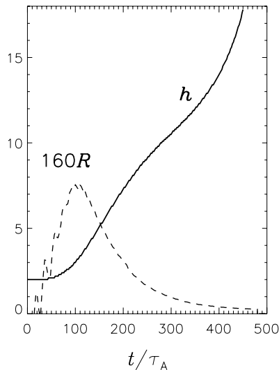
Figure 29: Temporal evolutions of the flux rope height ( h ) and the magnetic reconnection rate ( R ) in the numerical simulation of Chen and Shibata (2000) , which shows that the strong acceleration of the flux rope is coincident with the peak reconnection rate.
