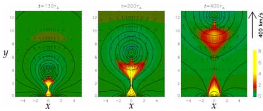
Figure 17: Still from a movie showing Evolutions of the magnetic field (lines), temperature (color, in unit of 10^6 \text{ K} ), and velocity (arrows) in the corona after the flux rope system is triggered to rise when the new flux emerges inside the filament channel (from Chen and Shibata, 2000). The scale for the velocity is shown at the upper-right corner. (To watch the movie, please go to the online version of this review article at http://www.livingreviews.org/lrsp-2011-1 .)
