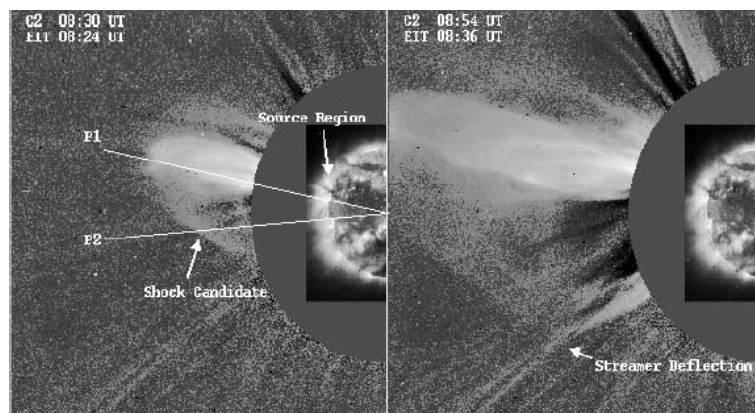
Figure 33: The LASCO/C2 white-light images showing a faint bow shock straddling over the 1999 April 2 CME. The solar disk is revealed by the EIT 195 Å images (adapted from Vourlidas et al. , 2003 ).
