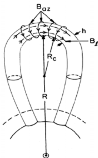
Figure 43: The flux rope model for the CME frontal loop (from Mouschovias and Poland, 1978).
