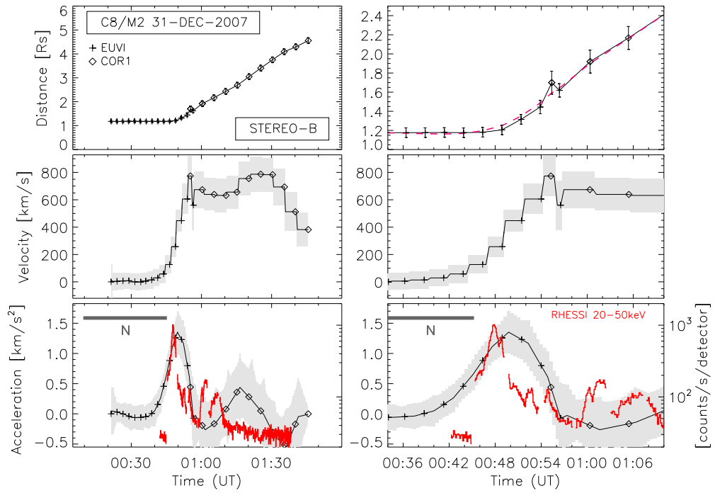
Fig. 9.— Same as Fig. 6 but for the 2007 December 31 C8.3 (M2) flare/CME event. The gray bar indicates the time range of RHESSI night (N).
