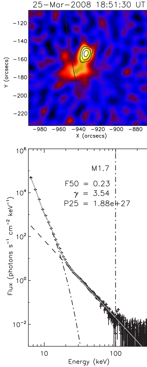
Fig. 11.— Same as in Fig. 5 but for the 2008 March 25 M1.7 flare. The HXR image is integrated over the energy band 18–30 keV. Contours show levels of 50%, 70%, and 90% of maximum emission for the energy band 30–50 keV.
