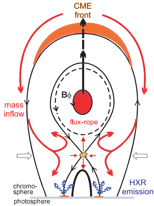
Fig. 13.— Cartoon illustrating the flare-CME feedback mechanism between the large-scale CME dynamics and small-scale flare processes. The upward moving CME evacuates the area in its wake, boosting mass inflow from aside into the reconnection region. The more mass and frozen-in magnetic field is transported into the region, the higher is the magnetic reconnection rate leading to larger flare energy release and to more efficient acceleration of particles. The successive closing of magnetic field lines due to reconnection increases the poloidal flux B_\phi in the eruption, which leads to a stronger upward oriented magnetic driving force (Lorentz force).
