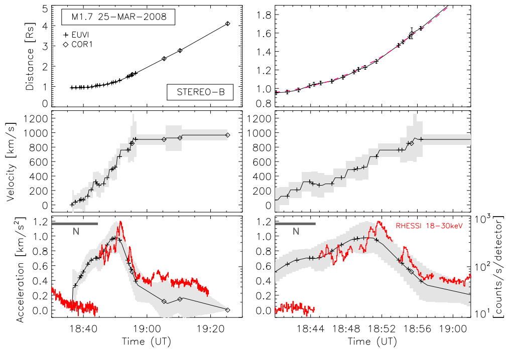
Fig. 12.— Same as Fig. 6 but for the 2008 March 25 M1.7 flare/CME event. The gray bar indicates the time range of RHESSI night (N).
