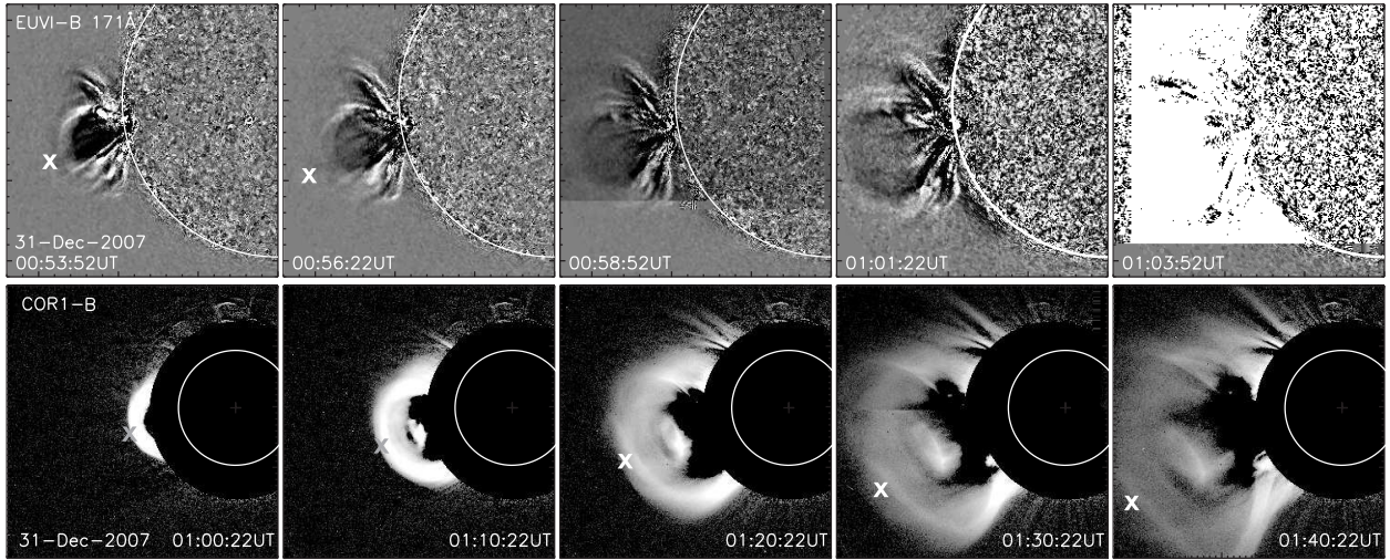
Fig. 7.— 2007 December 31, C8.3 (M2) flare/CME event observed with STEREO-B. Sequence of EUVI 171Å running difference images and COR1 images. Crosses indicate the measured leading edge from which the CME kinematics is derived (Fig. 9).
