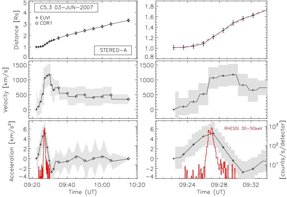
Fig. 6.— CME kinematics for the 2007 June 3 C5.3 flare/CME event. Top to bottom: CME distance, velocity, and acceleration against time together with the background subtracted flare HXR flux (red). Left: full height range, right: closeup view onto the early evolution phase. The pink dashed line in the right top panel (CME distance-time measurements) shows the regularized solution returned from the inversion technique. The grey shaded area in the CME velocity and acceleration curves indicates the 95% confidence level.
