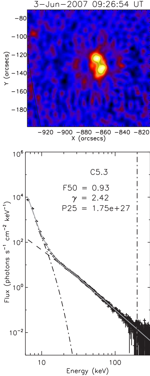
Fig. 5.— 2007 June 3 C5.3 flare. Top: RHESSI 30–50 keV HXR image integrated over 20 sec around the flare peak using front detectors 2 to 8 (except 5 and 7) reconstructed with the CLEAN algorithm. Bottom: RHESSI spectrum and fit components for the energy range 6–200 keV. The isothermal fit is indicated as dashed-dotted line, the non-thermal power-law fit as dashed line, and the sum of both components as thick gray line. The derived parameters, electron flux density at 50 keV F_{50} [photons s -1 cm -2 keV -1 ], photon spectral index \gamma , and power P_{25} [erg s -1 ] in electrons above a cutoff energy of 25 keV are given in the legend.
