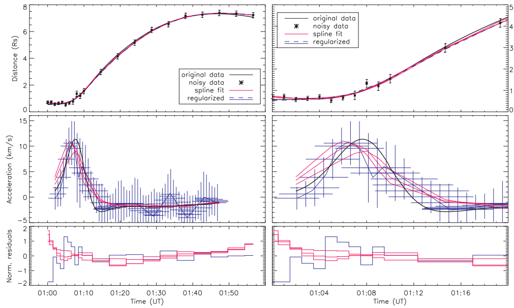
Fig. 2.— Top to bottom: same as in Fig. 1. Left: Impulsively accelerated CME evolution with rather high noise and errors. Right: Close up view for the time range during the peak acceleration phase.
