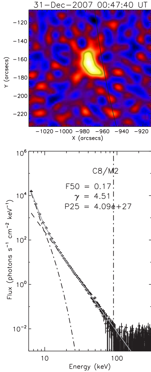
Fig. 8.— Same as in Fig. 5 but for the 2007 December 31 C8.3 (M2) flare. The HXR image is integrated over the energy band 20–50 keV.
