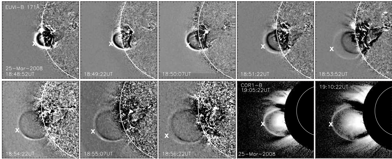
Fig. 10.— 2008 March 25, M1.7 flare/CME event observed with STEREO-B. Sequence of EUVI 171Å running difference images and COR1 images. Crosses indicate the measured leading edge from which the CME kinematics is derived (Fig. 12).
