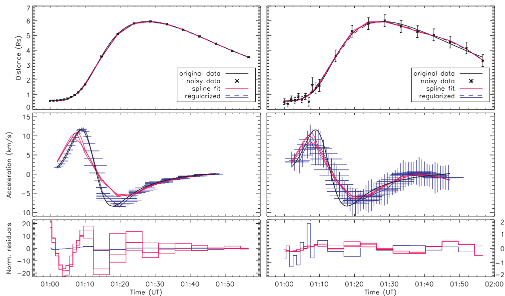
Fig. 1.— Top: Synthetic curve of CME kinematics (black) together with the data (asterisks), results derived from the regularization tool (dashed blue) and the spline fit (pink). Middle: derived acceleration profile (black: true solution, blue: regularization tool result, pink: spline fit result). Bottom: normalized residuals (we note that in the left panel case the residuals make no sense due to the division by errors of the order of zero). Left: sampling rate is smaller than for the “true” curve, but the data are without noise. Right: same sampling rate as left but with noise added to the data.
