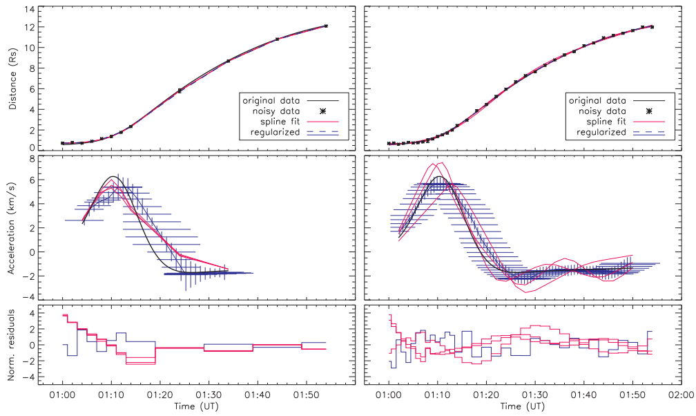
Fig. 3.— Top to bottom: same as in Fig. 1. Realistic scenario of CME evolution applying low noise to the data and error bars comparable to those from the observations. Left: Simulated is a time cadence of data points comparable to the actual observations. Right: same curve but with higher time cadence.
