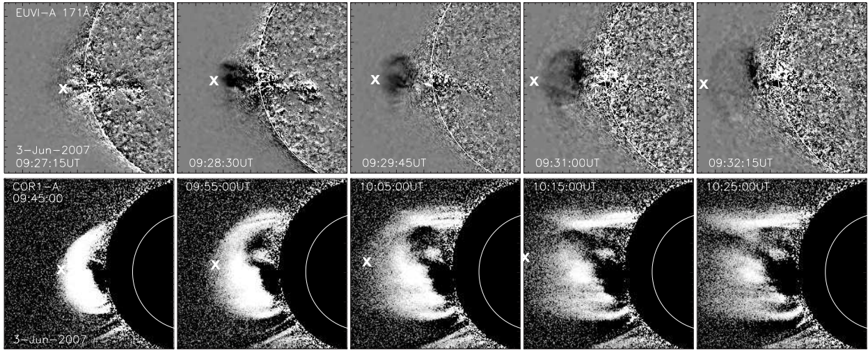
Fig. 4.— 2007 June 3, C5.3 flare/CME event observed with STEREO-A. Sequence of EUVI 171Å running difference images and COR1 total brightness images. Crosses indicate the measured leading edge from which the CME kinematics (shown in Fig. 6) is derived.
