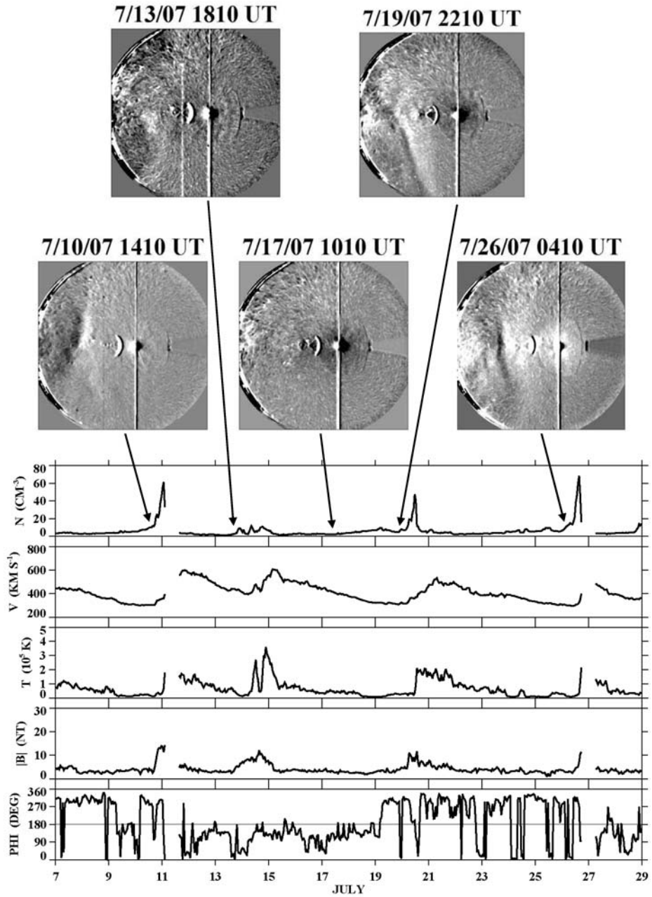
Figure 9 HI-2B images showing CIRs in the vicinity of the Earth in addition to in situ field and particle observations from the ACE spacecraft. (From Sheeley et al. , 2008b). Reproduced by permission of the AAS.
