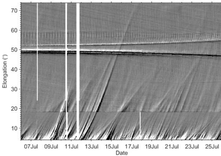
Figure 8 An elongation-time plot showing a ‘global’ picture of ejecta in the 4–74 degrees elongation range from 6 July to 26 July 2007 from HI on STEREO-A. The approximately horizontal features at around 50 degrees elongation are due to the presence of Venus and an associated optical ghosting effect, drifting through the field of view. The discontinuity at 18 degrees corresponds to the inner edge of the HI-2A field, with HI-2A observations being plotted where the HI-1A and HI-2A fields of view overlap. (From Davies et al. , 2009).
