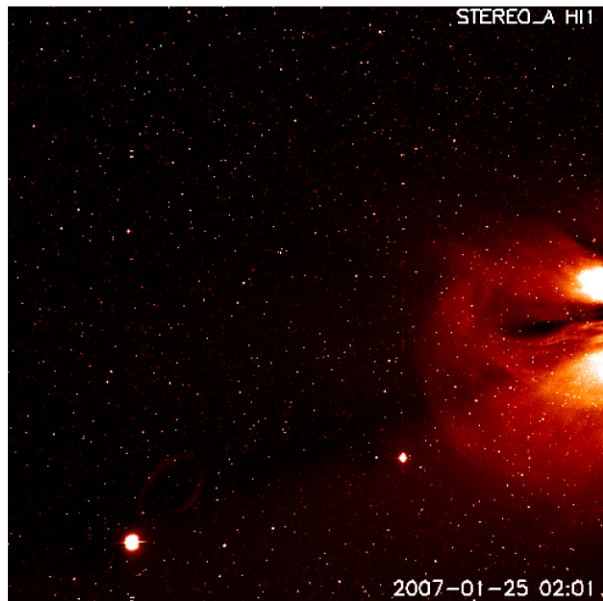
Figure 2 An HI-1A image taken on 25 January 2007. This image is 20 degrees across (80 solar radii in the plane of the sky) and the Sun is four degrees off the right of the frame. The planets Venus and Mercury can be seen (lower left and right, respectively) and a CME is clearly expanding into the right-hand side of the image. (From Harrison et al. , 2008).
