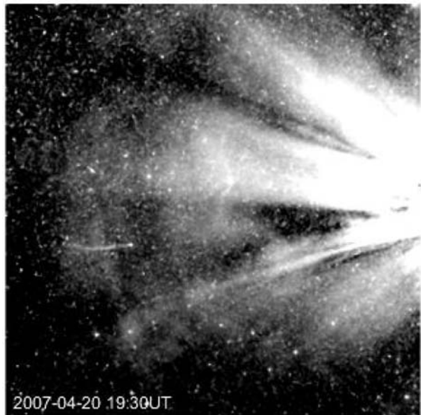
Figure 12 An HI-1A image showing comet Encke (centre-left) responding to an impact by a CME. The comet tail has been disconnected from the comet nucleus and in subsequent images was carried away from the nucleus in the solar wind flow.
