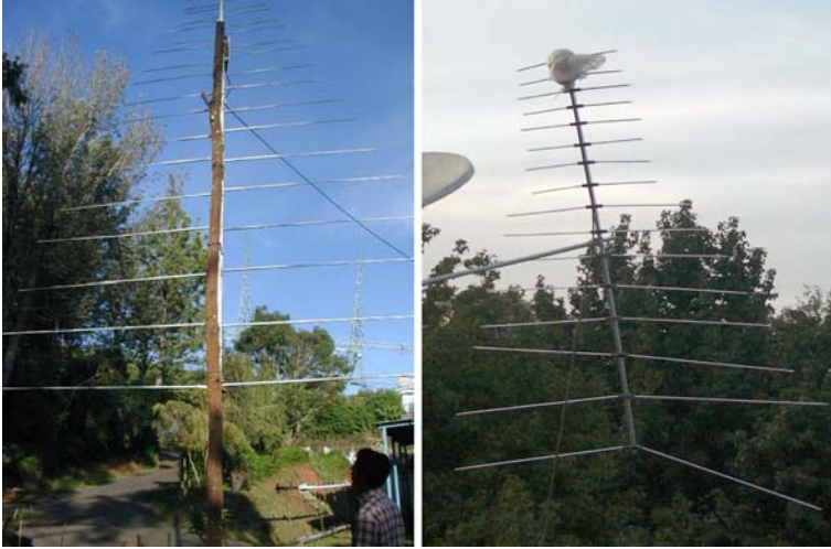
Fig. 3 Logarithmic periodic antennas of e-CALLISTO. Left: at Ootacamund (Ooty) in Tamil Nadu, India; Right: at UNAM, Mexico D.F.
