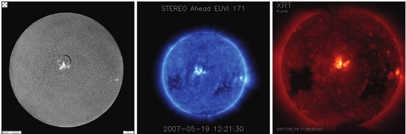
FIG. 1.—Multiwavelength solar images of the preeruption Sun on 2007 May 19. Left: BBSO global network H\alpha image (Kanzelhoehe) at 6:36 UT. Middle: SECCHI EUVI 171 Å image at \sim 12:21 UT. Right: Hinode XRT image at 11:30 UT. [Wavelet-enhanced EUVI anaglyph movies at 171 Å, 195 Å, and 304 Å are available in the electronic edition of the Journal.]
