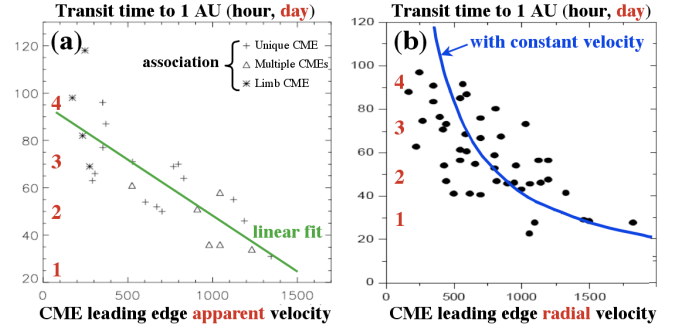
Fig. 3. The transit time of CMEs from the Sun to 1 AU in function of their coronal velocity. (a) The abscissa is the leading edge velocity of halo CMEs observed by LASCO, so it is the apparent velocity projected on the plane (Zhang et al., 2003). A simple linear least square fit is added. (b) The abscissa is the radial velocity, V_{\text{rad}} , measured from Helios 1 which was in quadrature with the Earth (within \pm 30^{\circ} from the plane of sky, Schwenn et al., 2005). The timing was corrected from Helios 1 to 1 AU by assuming a constant velocity. The expected result with a constant velocity between the Sun and 1 AU is added. It shows that ICMEs with a low initial coronal velocity are accelerated while fast ones are decelerated. The results of the two panels can be related with the result of Schwenn et al. (2005) on limb CMEs observed by LASCO: V_{\text{rad}} \approx 0.88V_{\text{exp}} (where V_{\text{exp}} is the lateral expansion velocity of the leading edge).
