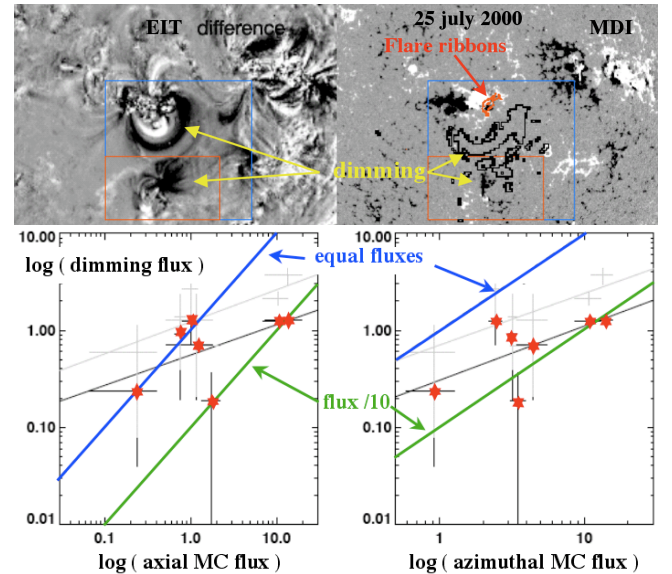
Fig. 11. Comparison of the magnetic flux found in dimmings and in the associated MC for 7 events. The top left panel shows a base difference image for one event. The dimming extensions are reported on the co-temporal magnetogram in the right panel. The bottom panels compare the flux found in dimmings with the axial and azimuthal flux found in the related MC. The red stars correspond to the mean of the absolute flux value between negative and positive dimming regions, and an azimuthal flux computed with MC length L = 1 AU. The error bars are mainly computed from varying alignment offsets (between MDI and EIT), using two dimming levels, and using the range L = 0.5 to 2 AU (Qiu et al., 2007).
