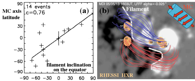
Fig. 6. Observed cases where the erupting filament and the associated MC axis have a comparable orientation. (a) Scatter plot and linear least square fits for 14 events. There is a relatively good correlation between the orientation of the filament and the MC axis, but they differ by more than 30^\circ for two events (Zhao and Hoeksema, 1998). (b) Example of association between an erupting filament and its related MC. Some field lines computed with a linear force-free extrapolation (blue and red lines) and the observed hard X-ray sources (pink regions) are added on top of the photospheric magnetogram (Yurchyshyn et al., 2006).
