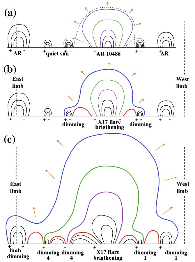
Fig. 15. Dimming spreading due to reconnection (mechanism proposed by Attrill et al., 2007, applied to the 28 Oct. 2003 event). (a) The CME lift-off. AR 10486 is represented by five field lines, while nearby bipoles are represented with three black field lines. The dashed lines represent the separatrices involved in the next reconnection (drawn symmetric to simplify the drawing). (b,c) Reconnection of the expanding CME field configuration with the surrounding bipoles (the just reconnected field lines are thicker and set to red for the short loops). By successive reconnections the outer shell of the CME expanding magnetic field is progressively rooted in more distant regions. This creates the spreading of the dimmings to larger spatial scales (Mandrini et al., 2007).
