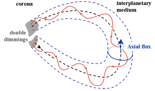
Fig. 10. Sketch showing the ejection of a flux rope already present in the corona (a negligible amount of reconnection is supposed during the ejection). When the radial extension of the field lines is well above the pressure scale height, the plasma is no longer confined in the corona by the magnetic field. It implies the formation of two dimmings at the footpoints of the flux rope. Their extension corresponds to a magnetic flux equal to the axial flux of the flux rope (detected in situ as a MC).
