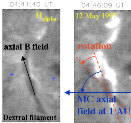
Fig. 7. Counterclockwise rotation of an erupting filament on 12 May 1997 (same event as shown on the left panel of Fig. 12). The magnetic configuration has a negative magnetic helicity as shown by several indicators (see Fig. 16): the dextral filament, the relative shift of flare ribbons, and the associated reverse-S sigmoid observed in X-rays (not shown). The rotation is confirmed by the axis direction of the associated MC at 1 AU (Green et al., 2007).
