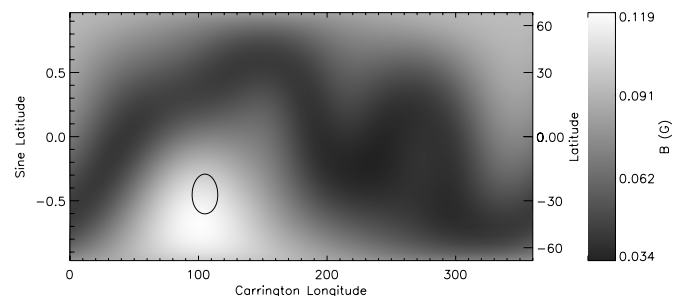
FIG. 4.—Distribution of the WSO CR 1980 extrapolated magnetic field strength at the height of 3.73 R_\odot , where the DH type II began to emit.
