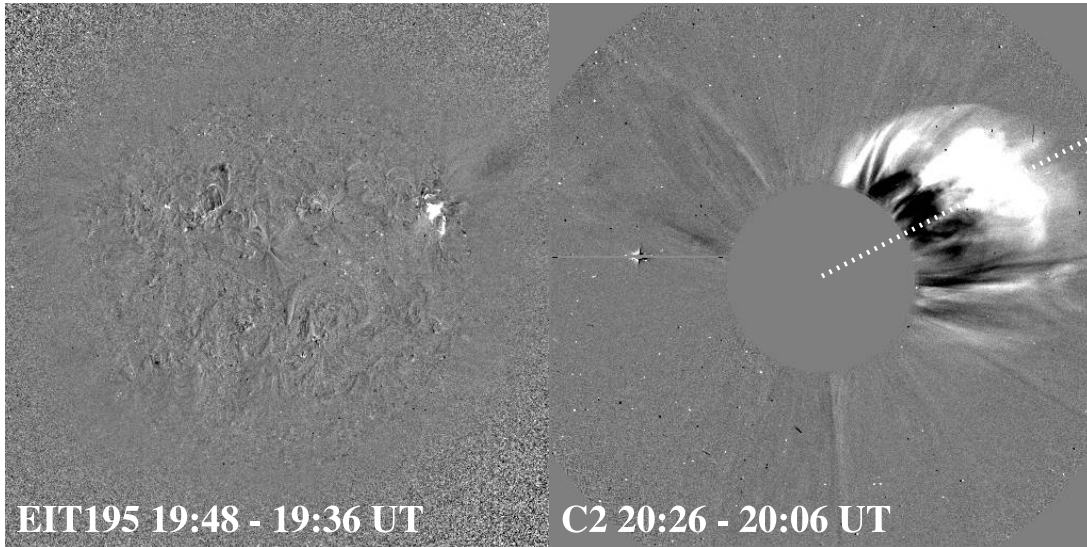
FIG. 5.—EIT and LASCO running-difference images of 2000 June 15 event.
