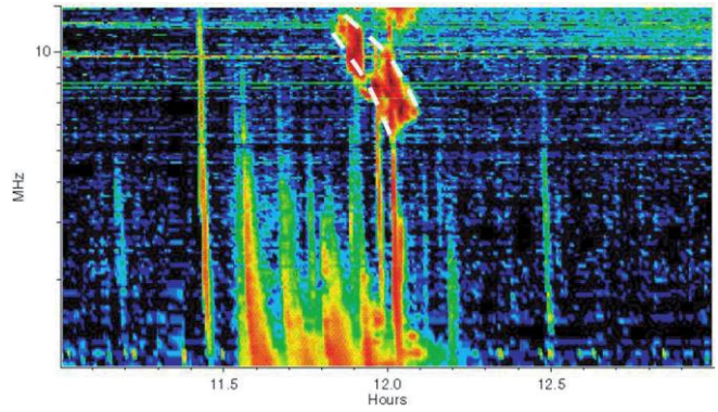
FIG. 3.— Wind/Waves observations during 11:00–13:00 UT on 2001 September 15. The dashed lines denote the frequency range of the fundamental component of a DH type II.
