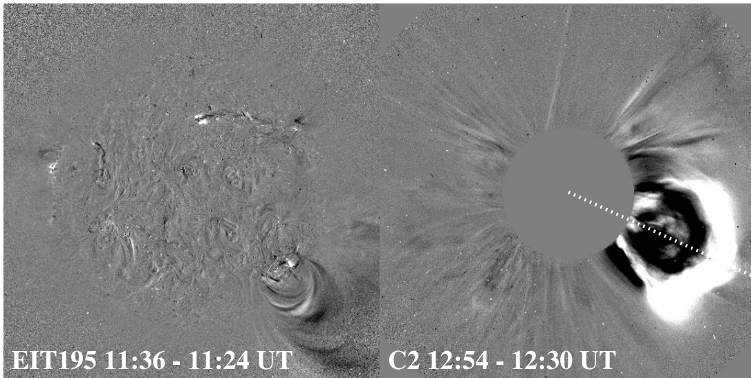
FIG. 1.—EIT and LASCO running-difference images of 2001 September 15 event. The dashed line indicates the direction along which the heights of the CME front were measured.
