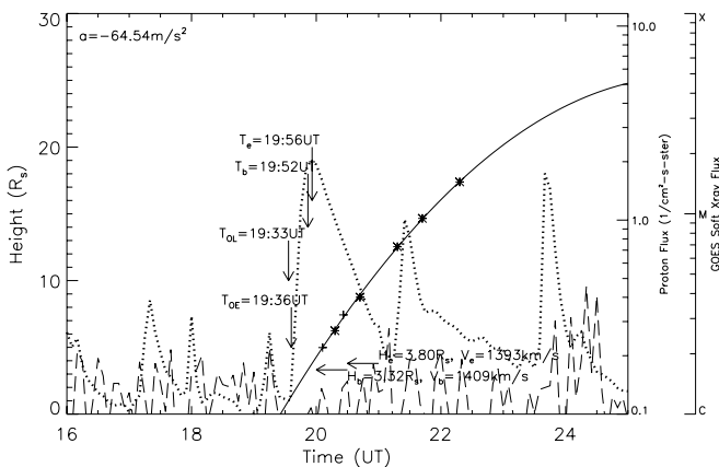
FIG. 6.—HT plot, proton flux profile, and soft X-ray profile of the 2000 June 15 event.
