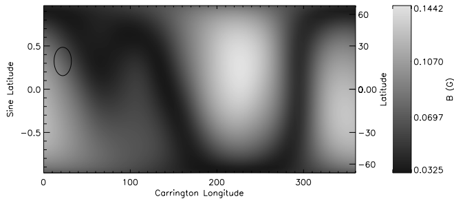
FIG. 8.—WSO CR 1963 extrapolated magnetic field strength at the height of 3.32 R_{\odot} , where the DH type II began to emit.
