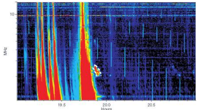
FIG. 7.—Wind/Waves observations during 19:00–21:00 UT on 2000 June 15.
