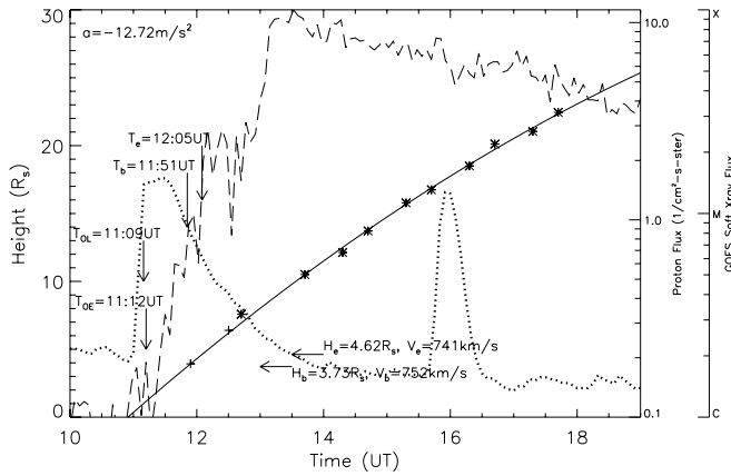
FIG. 2.—Heliocentric height-time plot of 2001 September 15 CME. The cross and asterisk denote the C2 and C3 measurements, respectively. The solid line is the second-order polynomial fitting line. T_{OL} denotes the extrapolated CME onset time. T_{OE} is the observed CME onset time in EIT images. T_b denotes the begin time of the associated DH type II, and H_b and V_b denote the height and speed of the CME front at that time. T_e denotes the end time of the DH type II, and H_e and V_e are the corresponding height and speed of the CME front. The dashed profile shows the flux of energetic protons with energy larger than 10 MeV observed by GOES . A 1 hr flight time of protons from the Sun to 1 AU has been deducted from the proton flux profile by assuming zero scattering in the interplanetary space. The dotted line denotes the GOES soft X-ray flux at the wavelength of 1.0–8.0 Å.
