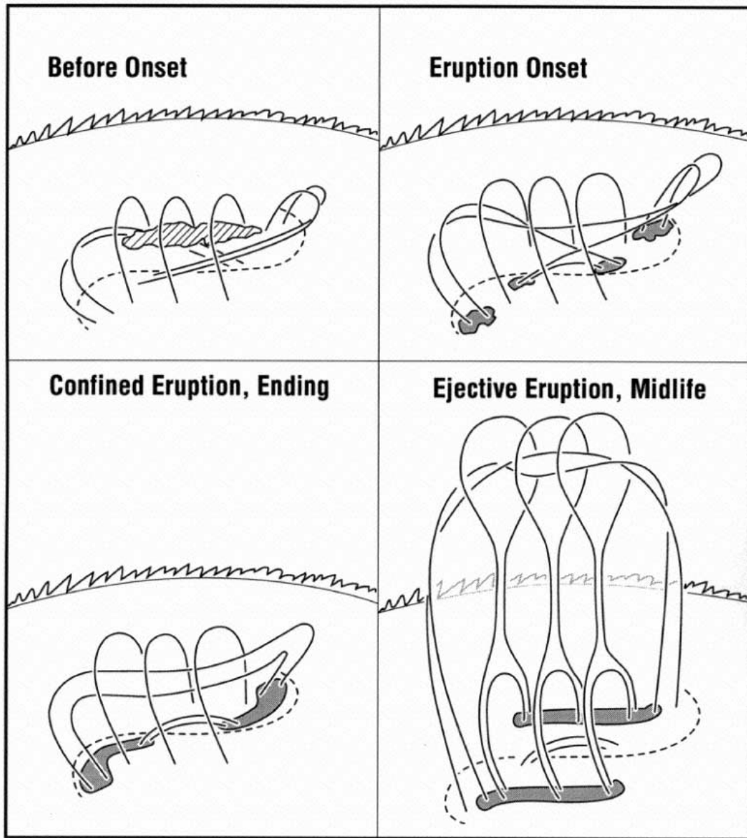
FIG. 1.—Depiction of the progression of the three-dimensional form and internal reconnection of the magnetic field in a sheared-core arcade as it explodes in either a confined (no-CME) eruption ( bottom left ) or an ejective (CME-producing) eruption ( bottom right ; figure reprinted with permission from Moore et al. 2001, ApJ, 552, 833).
