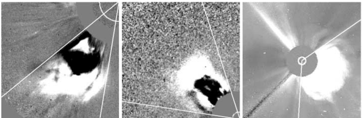
FIG. 4.— Snapshots of our three trial CMEs in the outer corona and at their final, maximum angular width. Left : LASCO/C2 running-difference image of the 2002 May 20 streamer-puff CME; final angular width: 41°. Middle : LASCO/C2 running-difference image of the 1999 February 9 quiet-region filament-eruption CME; final angular width: 64°. Right : LASCO/C3 image of the great active-region eruptive-flare CME; final angular width: 128°. [See the electronic edition of the Journal for a color version of this figure.]
