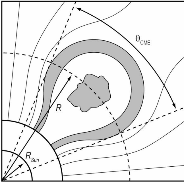
FIG. 2.— Schematic of a “spherical plasmoid with legs” CME viewed in the outer corona beyond the 2 R_{\odot} occulting disk of LASCOC2 when the radial distance R of the centroid of the CME (the center of the CME “sphere”) is about 4 R_{\odot} . At this stage, in our model CME (for any CME that explodes from a sheared-core arcade, and regardless of whether the CME is an over-and-out CME), the escaping flux-rope-and-arcade-envelope plasmoid sketched in the bottom right panel of Fig. 1 has greatly expanded and fills most of the interior of the somewhat larger entire CME plasmoid. In a typical, three-part-bubble CME such as that depicted here, we assume that this interior driving plasmoid is comprised of the magnetic field and plasma in the bright ( shaded region ) core, plus that in the surrounding dark ( unshaded region ) void, plus perhaps that in an inner layer of the bright ( shaded region ) outer shell of the CME.
