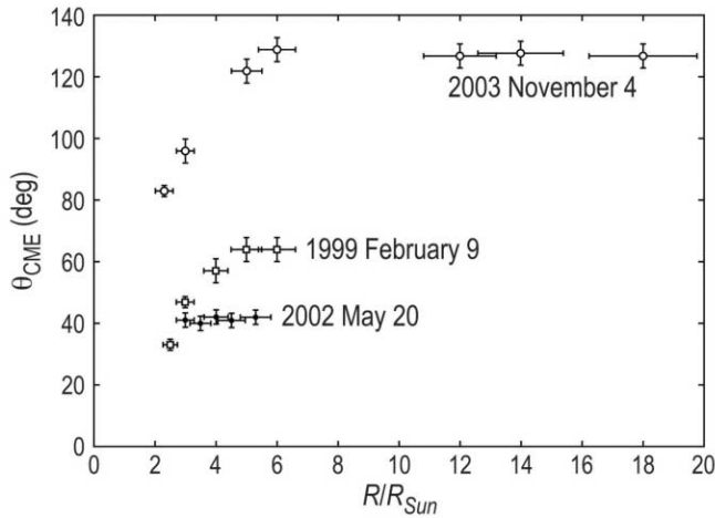
FIG. 5.—Observed progression of the angular widths of our three trial CMEs. The measured angular width \theta_{\text{CME}} is the angle between two encompassing tangent radial lines, such as those shown in Fig. 4. The measured radial distance R of the “centroid” of the CME is the average of the radial distances of the two tangent points. The error bars are from the uncertainties in the lateral and radial locations of the tangent points.
