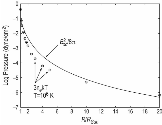
FIG. 3.—Empirically estimated radial profiles of the magnetic pressure ( B^2/8\pi ) and thermal plasma pressure ( 3n_e kT ) in the outer corona ( 2-20 R_\odot ; see text). The magnetic pressure dominates at distances of 2-10 R_\odot and is comparable to the plasma pressure at 10-20 R_\odot .
