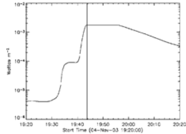
Figure 4. The CME onset time in GOES 1–8Å soft X-ray flux
