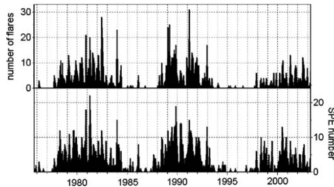
Figure 4. Monthly numbers of \geq M5 X-ray flares ( upper panel ), and monthly SPE numbers over the three solar activity cycles ( bottom panel ).
