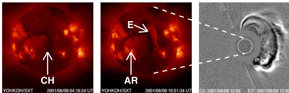
Figure 3. Two Yohkoh/SXT images on 2001 August 09 at 0418 and 1051 UT, showing the coronal hole (CH) and the SXT arcade (E). The LASCOCO difference image at 1206 UT shows a white light CME associated with the SXT arcade. This CME seems to be too early to be associated with the SEP event of 2001 August 09. Even though the solar source was close to the disk center, the CME moved mostly to the west, probably because of the extended coronal hole immediately to the east of the CME source region. Also marked is active region 9570 (AR), from which an EUV eruption was observed later in the day at 1822 UT by EIT (but not by LASCOCO).
