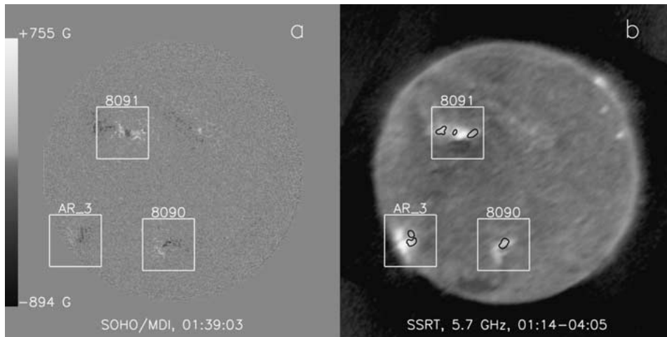
Figure 8. Comparison of the SSRT polarization map of 6 October 1997 with a photospheric magnetogram. (a) SOHO/MDI magnetogram of 6 October 1997, 01:39:03 UT. (b) SSRT Stokes I map (half-tone, same as in Figure 7(a)) overlaid with contours of the degree of polarization computed from the SSRT Stokes I and V maps under the assumption of optically thin emission. Contour levels are \pm 5\% . Half-tone images are nonlinearly displayed to show both bright and faint features. Solar north is up.
