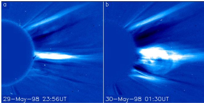
Fig. 6. LASCO/C2 data illustrating the propagation of a streamer blowout CME observed in association with the soft X-ray brightening of TLS-A2 on 29th May 1998. a) shows streamer brightening at 23:56 UT. This is followed at 00:28 UT by a plasmoid ejection extending along approximately the same angle. b) illustrates the appearance of this plasmoid at 01:30 UT.
