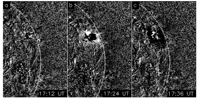
Fig. 2. SOHO/EIT 195\text{\AA} percentage difference images (20%) illustrating the event onset on 12th March 2000 from the northern hemisphere active region. This is an event from the “A” category which shows a response in the TLS to the CME. The FOV of the images are 15.6' by 22.1' . A bright region showing material moving away from the northern active region is observed in b) together with a brightening in the vicinity of the active region. c) illustrates dimming in the vicinity of the northern active region when compared to the pre-event image a) . Images are 5.2'' per pixel resolution.
