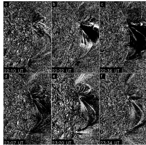
Fig. 5. Coronal EUV dimming observed in association with TLS A2 on 29th May 1998. Images are percentage difference (20%), illustrating morphology changes observed in EIT 195 Å data at a resolution of 2.6'' per pixel. The FOV of each image is 15.8' × 22'. b) illustrates evacuation of material from the vicinity of the northern active region. This dimming is seen to extend c) to the width of the transequatorial loop system. Off limb brightening to the north of the dimming region ( b) , c) , d) takes place as nearby coronal streamers are displaced by the eruption. Bright loops begin to appear in the dimming region ( e) , f) following eruption and prior to the first observation of the cusp shaped feature in SXT (Fig. 4).
