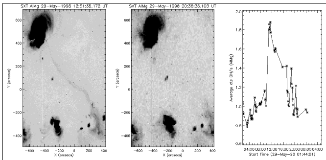
Fig. 9. The changing morphology of a TLS observed on 29th May 1998 with north and south locations N26E21 and S22W13 respectively. The first panel shows the brightened TLS following the first CME onset (11:43 UT). The second panel shows the same region following the second CME onset (17:38 UT) and TLS disappearance. The third panel shows the SXT light curve of the TLS showing the decrease in intensity back to background levels following the second CME. SXT data has a resolution of 4.9'' .
