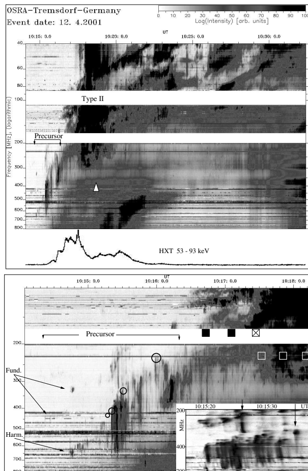
Figure 1. Dynamic radio spectrum of the event on 12 April 2001. Top panel: The event starts with a harmonic type II precursor, followed by a multilane type II burst. The precursor is accompanied by hard X-ray emission. At frequencies above those of type II a strong type IV occurs. Second panel: hard X-ray light curve (HXT) in the range 53–93 keV. Bottom panel: the precursor lanes consist mainly of a sequence of fast reverse slope (RS) drift bursts. Insert: Enlarged part shows the precursors (RS) bursts. Two of them are indicated by arrows.
