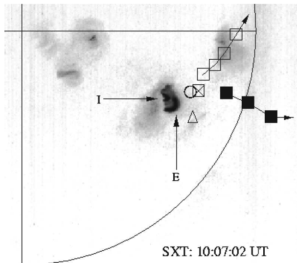
Figure 2. Pre-flare Yohkoh SXT image overlaid on radio source positions (centroids) at the time indicated by corresponding marks in Fig. 1. \circ – precursors source position. The squares represent the positions and trajectories of different type II lanes. \blacksquare – type II sources at 164 MHz 10:16:41–10:18:11 UT. \square – type II sources at 236 MHz at 10:17:31–10:19:11 UT. \boxtimes – an additional type II source at 164 MHz at 10:17:21 UT. \triangle – type IV source at 432 & 327 MHz at 10:18:40 UT. Arrows point at the inner (I) and outer (E) loops. North is up, west is to the right.
