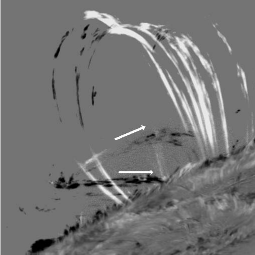
Fig. 4. b. The H-alpha Doppler image of the loop system in Figure 4a. Material moving toward the observer is dark gray to black; material moving away is light gray to white. The northern leg of the “bent-over” loop is strongly blueshifted (very dark) above the limb; below the limb, this leg shows as a thin dark strand linking on down to its foot under the arcade.
