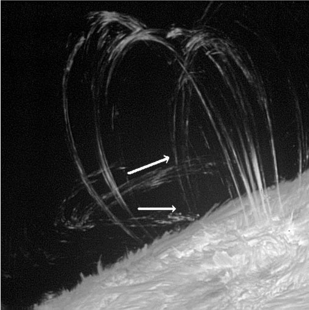
Fig. 4. a. The large post-flare loop system observed by the Lockheed group with the Swedish telescope at La Palma. This H-alpha line-center filtergram was taken at about 8:15 UT, 26 June. The arrows here and in Figure 4b indicate that the center-line and Doppler movies show that the H-alpha material all along both legs of the “bent-over” loop was flowing downward at this time. This image has been edge-enhanced and the brightness and contrast adjusted to best show the loops above the limb. In Figures 4b and 4c, the northern leg of the “bent-over” loop is traced below the limb to its foot on the floor of the arcade tunnel.
