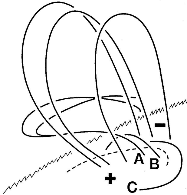
Fig. 5. Summary sketch of the 3-D configuration of the main magnetic structures observed in the late phase of our large two-ribbon flare, showing that the core field extending out of the north end of the arcade had a coronal elbow with its far end rooted behind the arcade. We have deduced this 3-D magnetic field configuration directly from the observations presented in this paper. See Section 3 for detailed identification of the sketched features with observed features.
