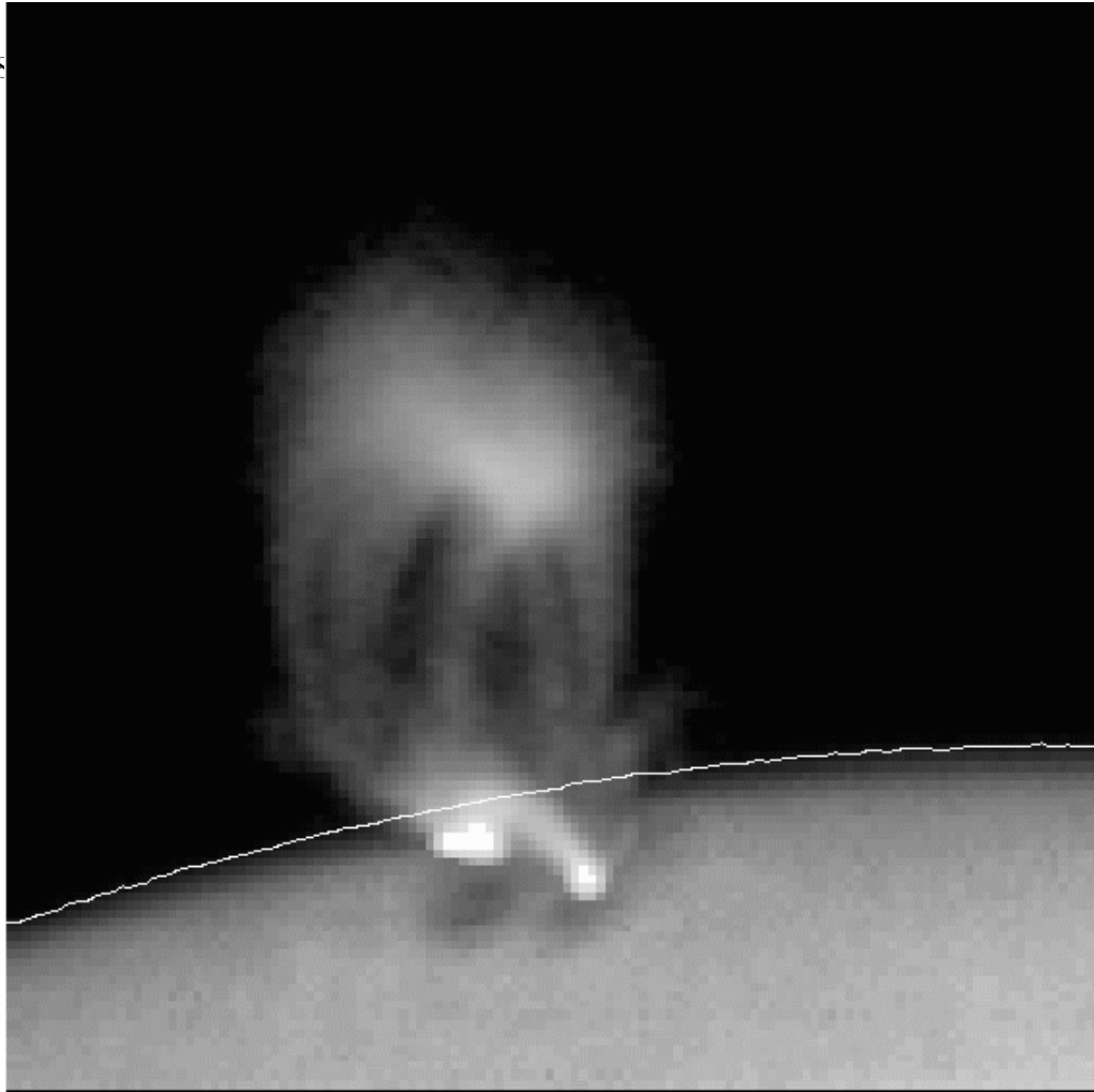
Fig. 3. The large flare arcade and a subflare in the underlying core field late in the decay phase of the large flare. A Yohkoh SXT X-ray image of the flare (at 06:56:13 UT, 26 June) is superposed on a Yohkoh SXT visible-light image (taken at 07:07:25 UT) showing the sunspots in the flare region. The thin white arc traces the photospheric limb.
