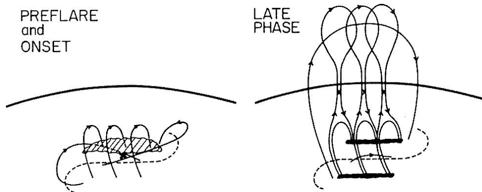
Fig. 1. The 3-D magnetic field configuration and eruption model deduced by Moore and LaBonte (1980) for the large two-ribbon flare of 29 July 1973. The heavy arc is the east limb; the backward-S dashed curve is the photospheric polarity dividing line of the overall bipolar magnetic field of the flare site; curves with arrowheads are magnetic field lines; Xs mark places where reconnection occurs. The shaded feature is the large dark chromospheric filament that was suspended in the preflare backward-S sheared core field and erupted with the core field at flare onset. In this scenario, early in the eruption, reconnection occurs under the filament, between the inner legs of the core-field coronal elbows [having their outer ends in the curls of the early flare ribbons (not shown here)], releasing the upper reconnected core field to erupt upward and “open” itself and the overarching envelope field. In the late phase, the opened envelope field recloses by reconnection, forming the growing arcade of flare loops rooted in the spreading flare ribbons. At the late stage of the flare ribbons depicted here, the 3-D topology of the magnetic field would be as shown, but the erupted field would reach far into the outer corona, much farther than in this sketch.
