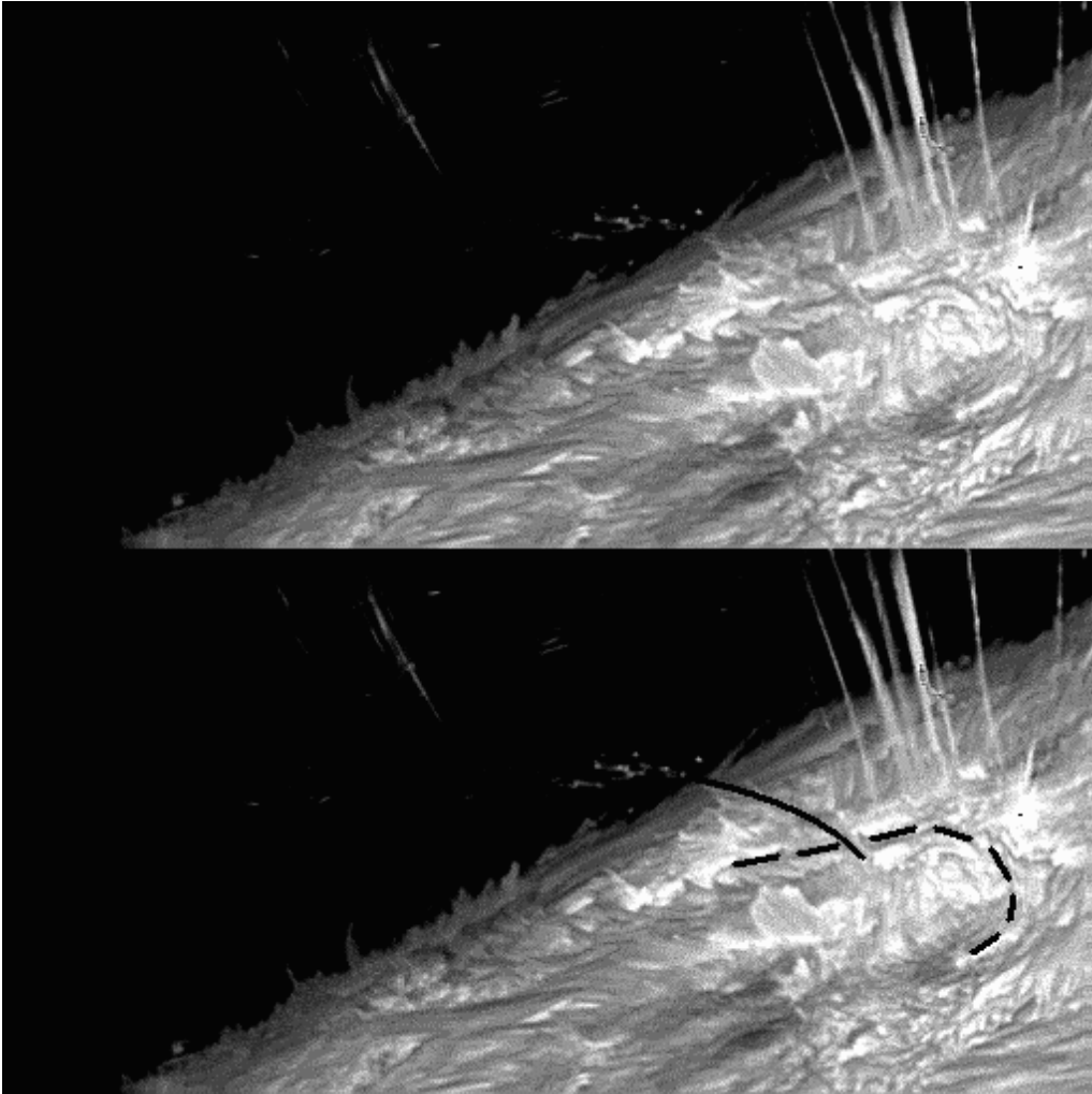
Fig. 4. c. Magnetic location of the foot of the northern leg of the “bent-over” loop. The image in the top panel is the same as that in Figure 4a but with the brightness and contrast adjusted to best show the fibril structure under the arcade. This image is repeated in the bottom panel with two curves drawn in, tracing key structures seen in the top panel: the dashed curve is the locus of the polarity dividing line traced by the low thin filament under the arcade, and the solid curve traces the northern leg of the “bent-over” loop below the limb. It is seen that the lower end of this leg crosses in front of the thin filament, showing that this leg of the “bent-over” loop was rooted on the near side of the polarity dividing line.
