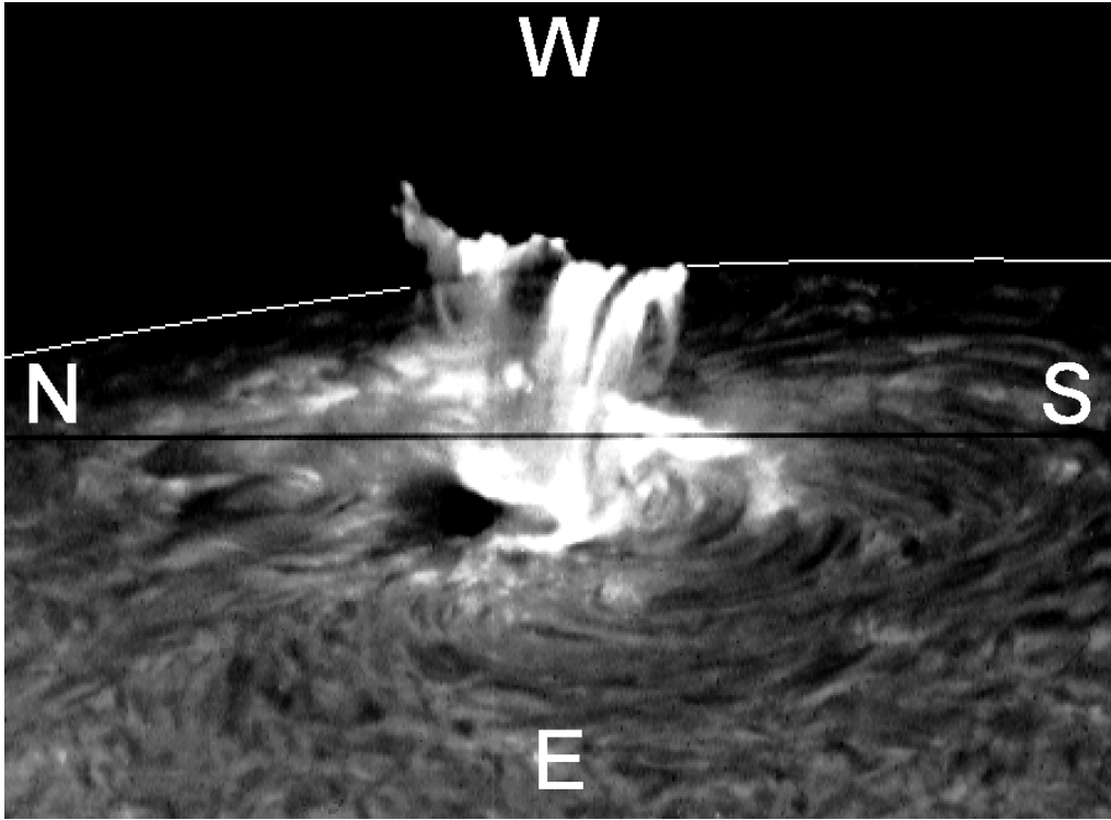
Fig. 2. Flare ribbons, flare loop arcade, and chromospheric fibrils early in the decay phase of the large two-ribbon flare of 25/26 June 1992. The background arc traces the chromospheric west limb. This H-alpha image (from a spectrograph slit jaw) was taken at Hida Observatory at 20:54:23 UT on 25 June 1992.
