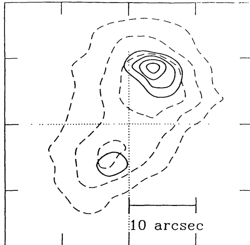
Figure 12 White-light emission patches ( dashed contours ) at the footpoints of the loop structure of the 15 November 1991 flare, as observed at 4308 Å with the Yohkoh/SXT instrument. The overlay shows the position coincidence with the hard X-ray sources ( solid contours ) detected by Yohkoh/HXT (Sakao et al 1992), establishing the penetration of nonthermal electrons deep into the chromosphere.
