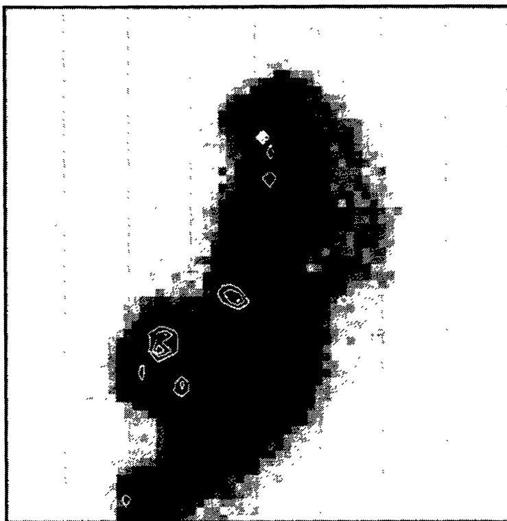
Figure 11 Footpoint brightening seen in soft X rays by the Yohkoh/SXT in a flare of 26 January 1992 (Hudson et al 1994c). The continuous tones represent soft ( \sim 1 keV) X-ray brightness, and the contours represent hard (33–53 keV) X-ray brightness. They both show a patchy character with some common features. This pattern is typical of most flares during the impulsive phase and tends to confirm the occurrence of particle-driven evaporation during the impulsive phase of the flare. The pixel size is 2.46'' . N is up and E is to the left. The flare occurred near the SW limb in a region almost totally devoid of sunspots.
