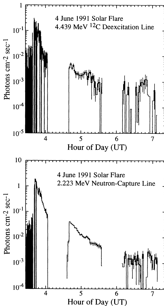
Figure 5 Time variations of 2.223 MeV (neutron capture; top panel ) and 4.44 MeV ( 12 C deexcitation; bottom panel ) following the 4 June 1991 event, again illustrating the extraordinary duration of the high-energy processes (Murphy et al 1994). These line measurements were accompanied by a time-extended detection of solar neutrons at ground level (Struminsky et al 1994a).
