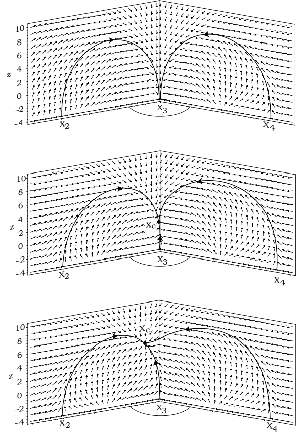
Fig. 8. Vector field in the plane of the separators X_2X_3 and X_3X_4 . Top: Configuration corresponding to the system parameters presented in Table 2. Middle: the same for the case when charge 3 is moved to the point x_3 = 29.4 . X_c is a new null point. Bottom: the same for the case when charge 3 is moved to the point (x_3, y_3) = (30.0, 37.0) .
