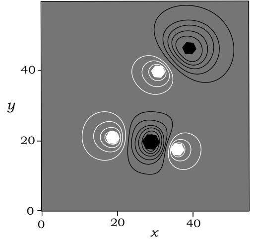
Fig. 3. Model magnetogram corresponding to 00:00 UT.
