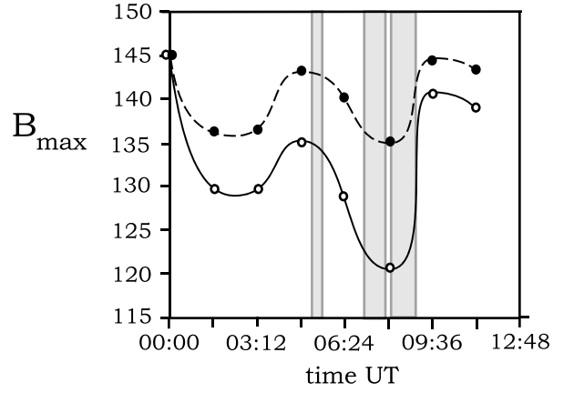
Fig. 7. Maximum values of magnetic field (in Gauss) on both separators for each of the eight time points. Black and white circles correspond to the separators X_2X_3 and X_3X_4 , respectively.
