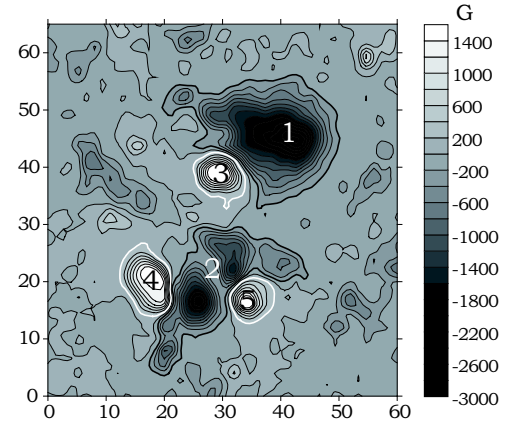
Fig. 2. Magnetogram obtained by MDI/SOHO at 00:00 UT on 2003 Nov 18. The white (black) thick lines are 200 G (-200 G) levels. A length unit corresponds to one MDI pixel ( 1.45 \cdot 10^8 cm).
