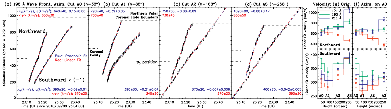
Figure 10. (a)–(d) Positions of the north- and southward 193 Å EUV wave fronts obtained from azimuthal space–time diagrams as in Figure 4. The sign of the southward distance is reversed. Overlaid dashed lines are parabolic (blue) and linear (red) fits, labeled with fitted parameters. The horizontal dotted line denotes the position where the velocity v_0 from parabolic fits is evaluated. (e) Height distribution of velocities from linear fits to wave fronts on different azimuthal cuts at 171, 193, and 211 Å. (f) Same as (e) but for velocities scaled onto the lowest cut A0, equivalent to angular velocities in the azimuthal direction with respect to the disk center. (A color version of this figure is available in the online journal.)
